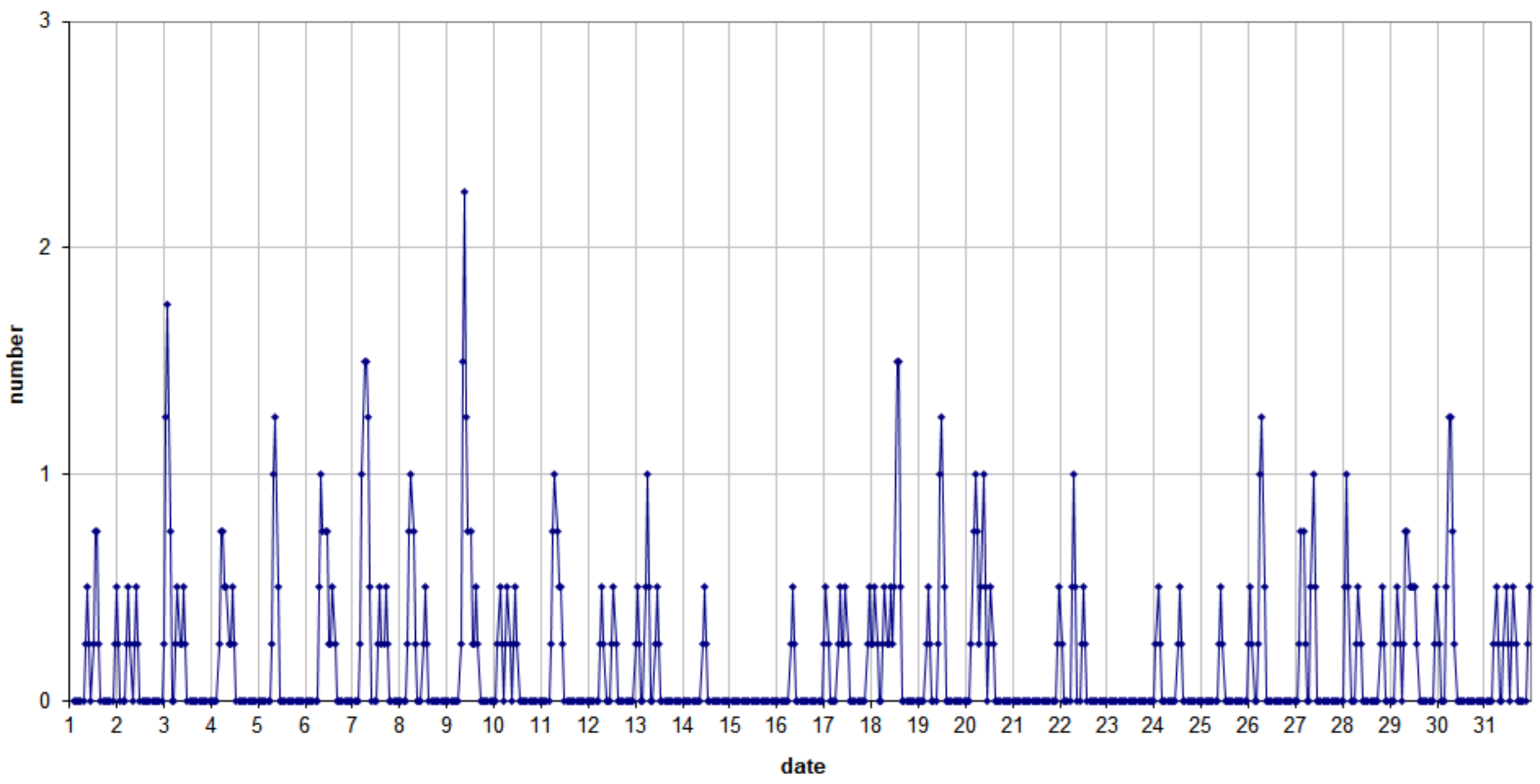
49.99MHz - RadioMeteors March 2021 number of reflections >10 seconds per hour (weighted average) Felix Verbelen (Kampenhout)
