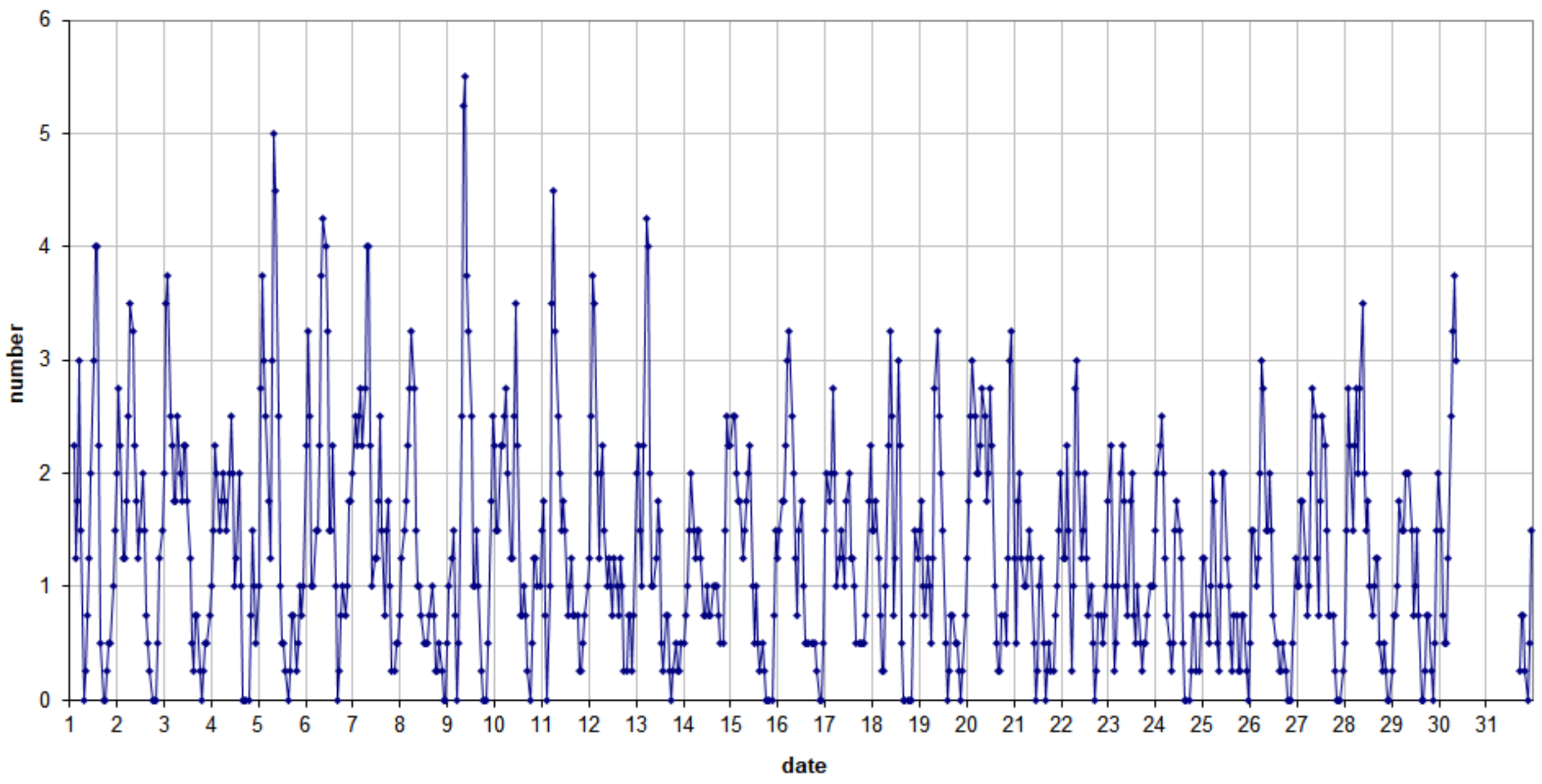
49.99MHz - RadioMeteors March 2021 number of overdense reflections per hour (weighted average) Felix Verbelen (Kampenhout)
