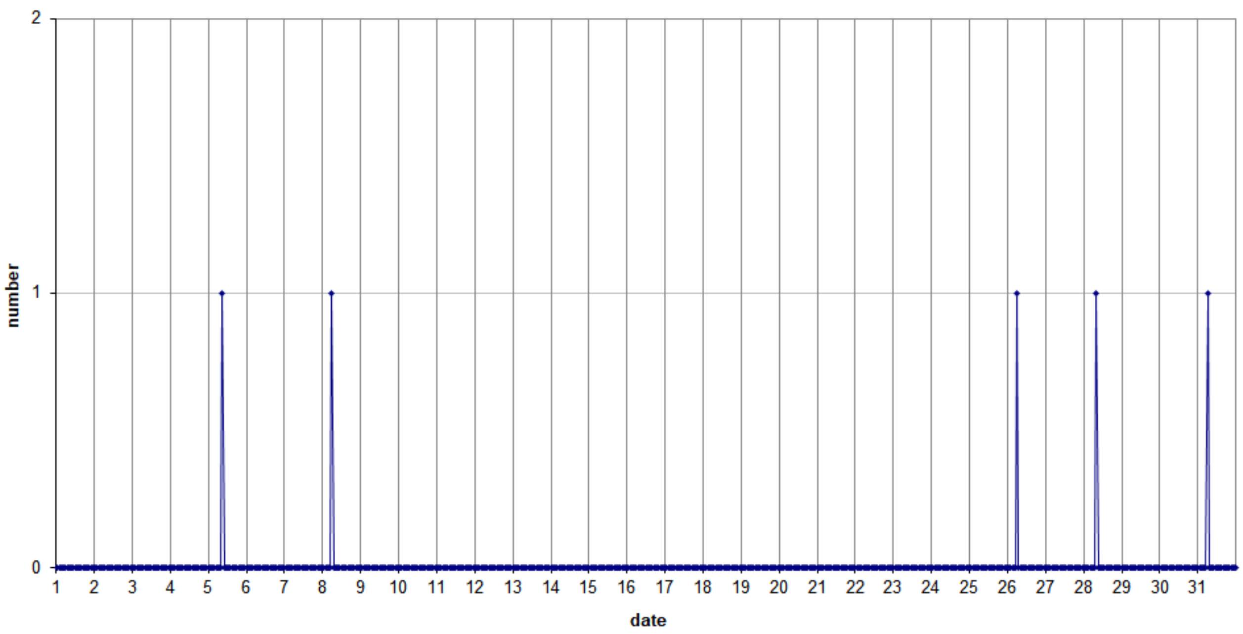
49.99MHz - RadioMeteors March 2021 hourly totals of overdense reflections longer than 1 minute Felix Verbelen (Kampenhout/BE)
