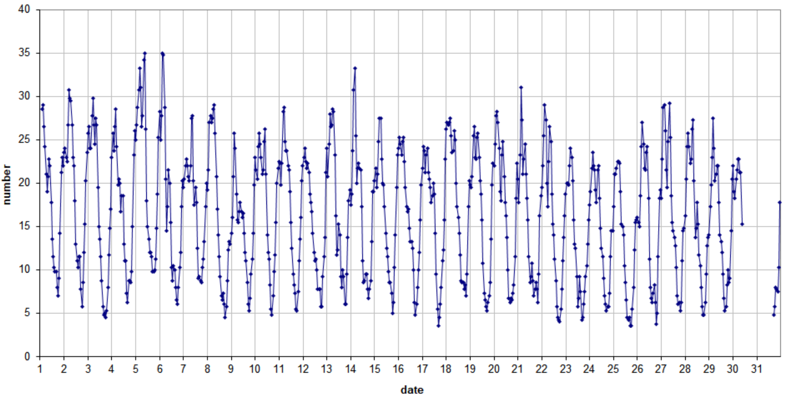
49.99 MHz - RadioMeteors March 2021 number of "all" reflections per hour (weighted average) (automatic count_Mettel5_7Hz) Felix Verbelen (Kampenhout)
