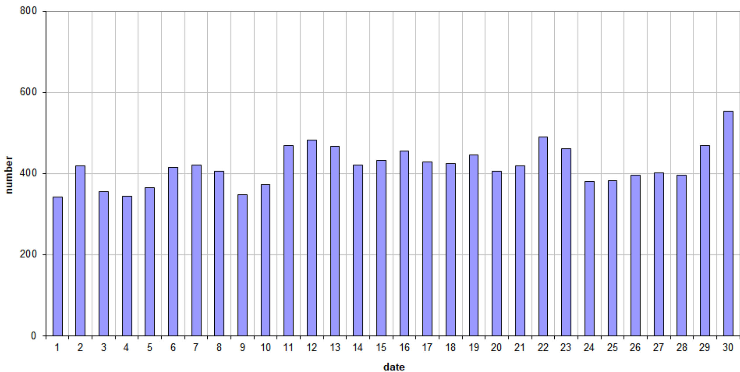
49.99MHz - RadioMeteors April 2021 daily totals of "all" reflections (automatic count_Mettel5_7Hz) Felix Verbelen (Kamphenhout)
