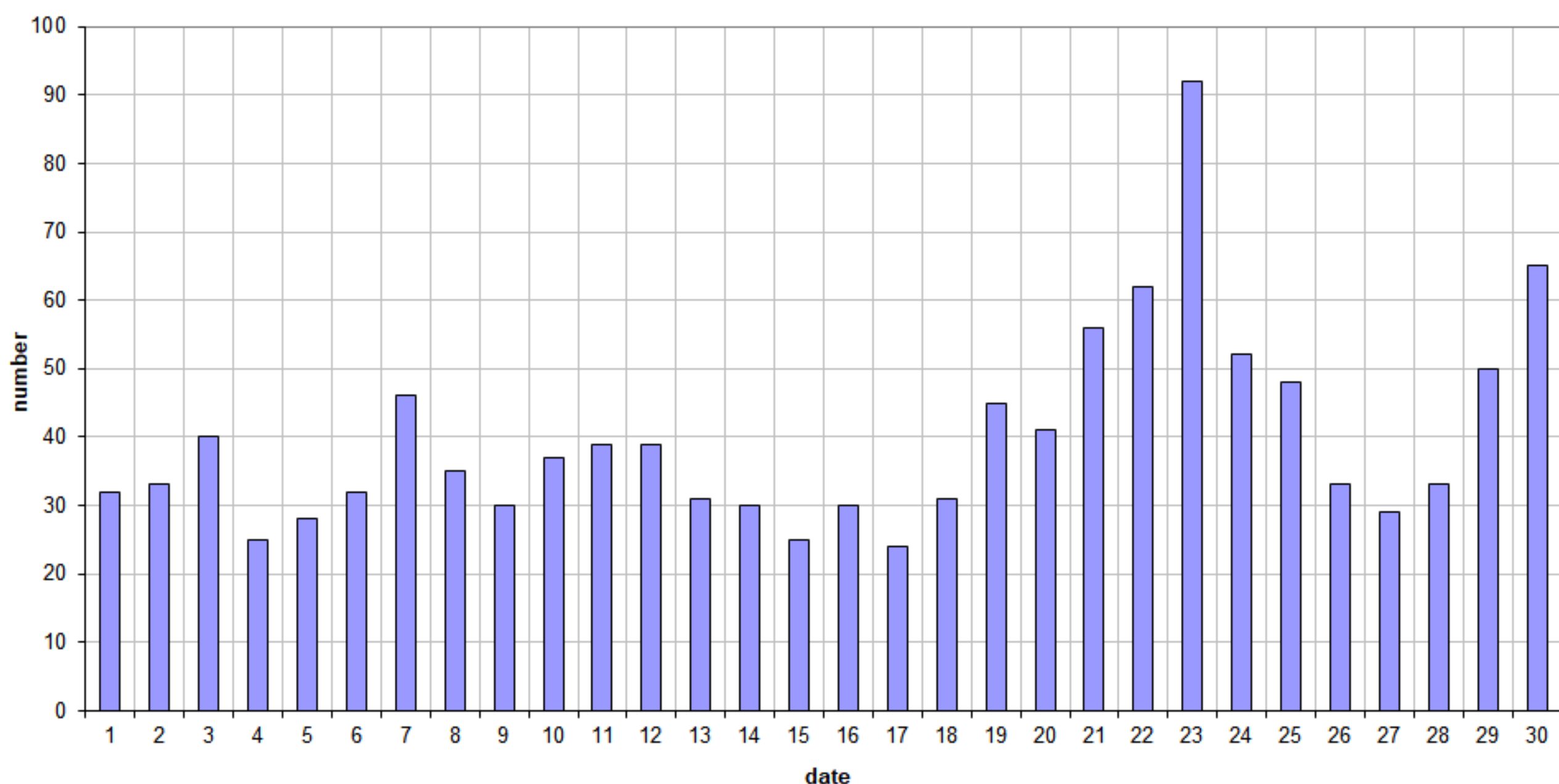
49.99MHz - RadioMeteors April 2021 daily totals of all overdense reflections Felix Verbelen (Kamphenhout)
