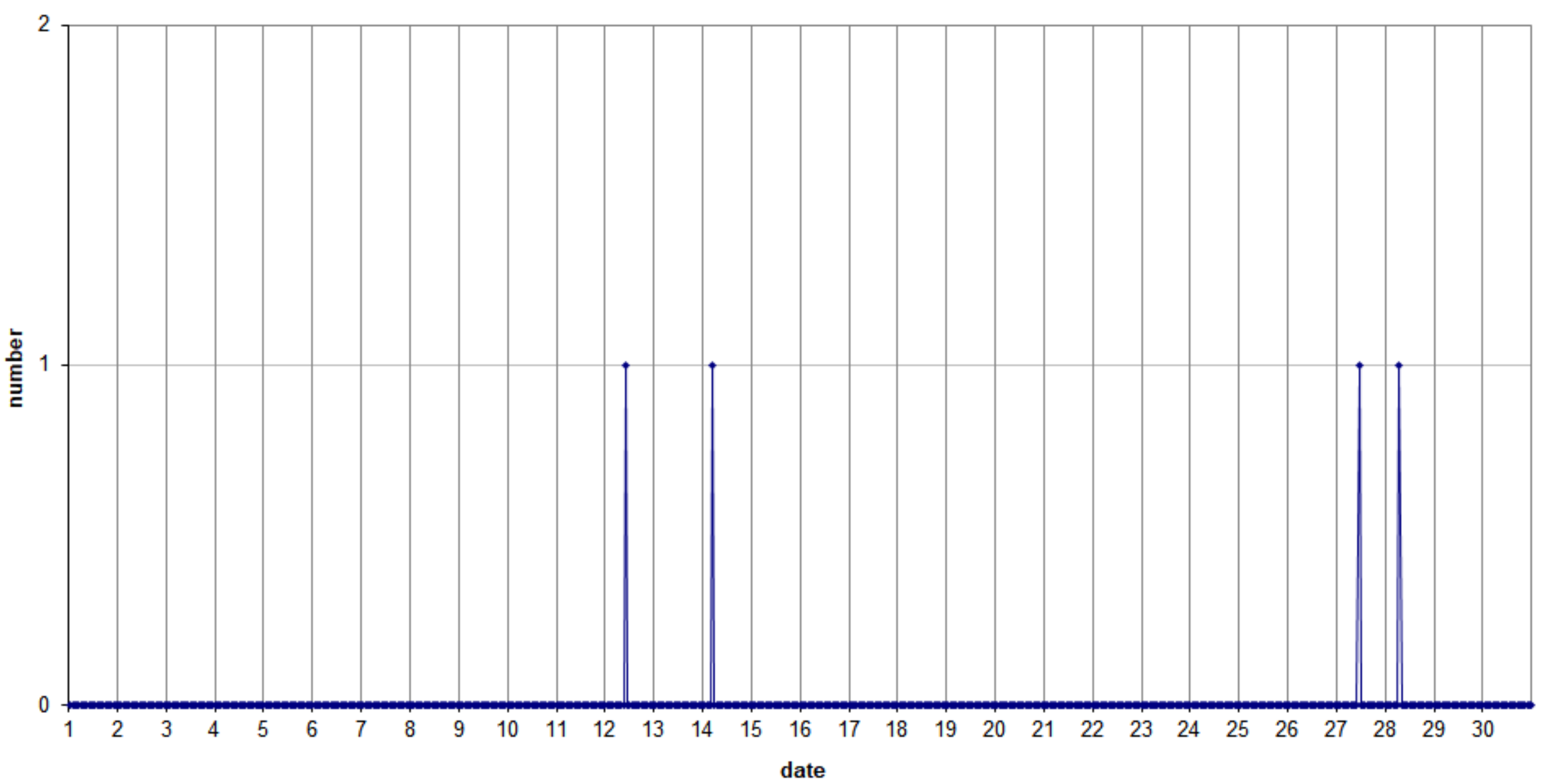
49.99MHz - RadioMeteors April 2021 hourly totals of overdense reflections longer than 1 minute Felix Verbelen (Kampenhout/BE)
