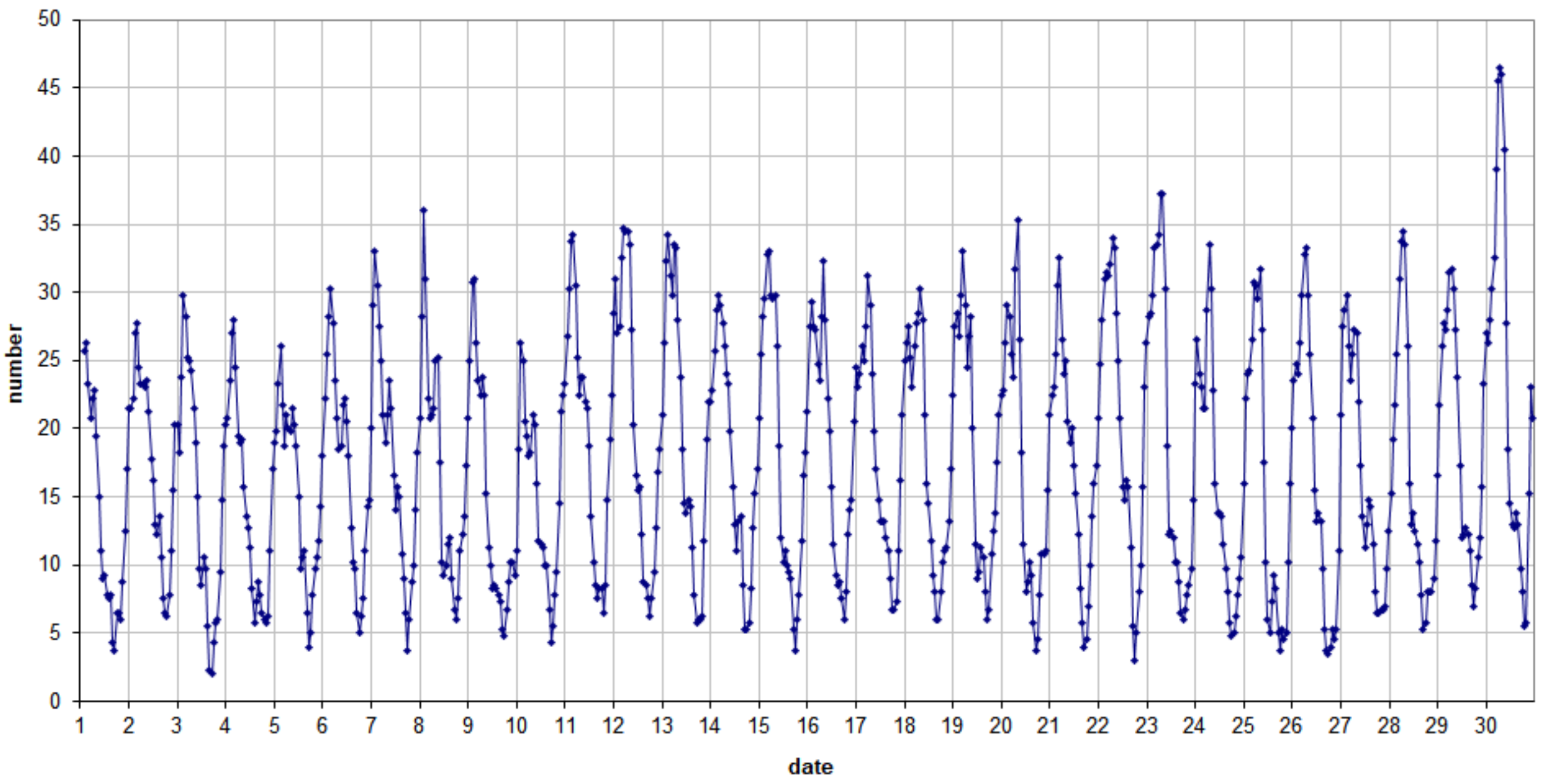
49.99 MHz - RadioMeteors April 2021 number of "all" reflections per hour (weighted average) (automatic count_MetteI5_7Hz) Felix Verbelen (Kampenhout)
