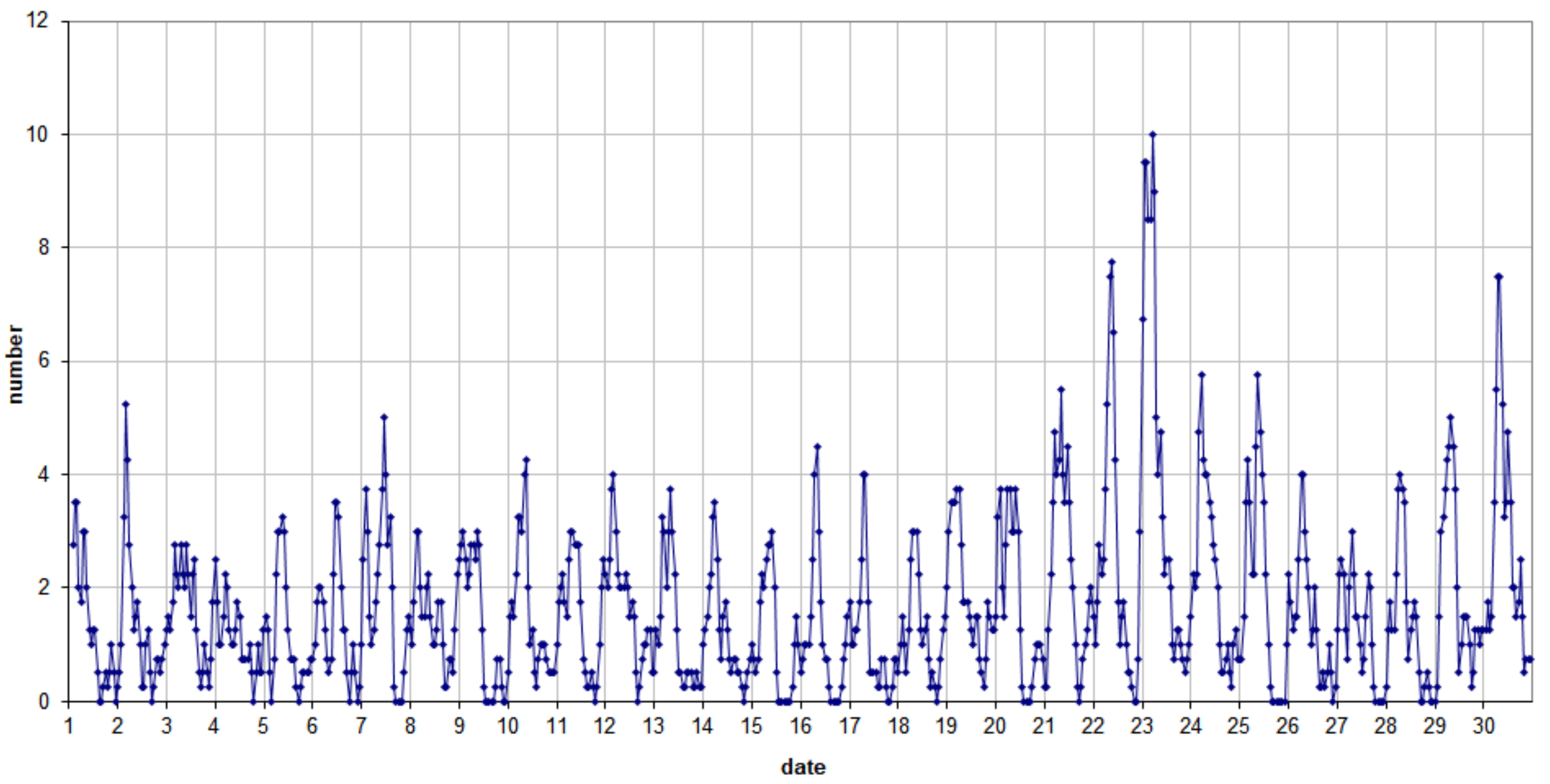
49.99MHz - RadioMeteors April 2021 number of overdense reflections per hour (weighted average) Felix Verbelen (Kampenhout)
