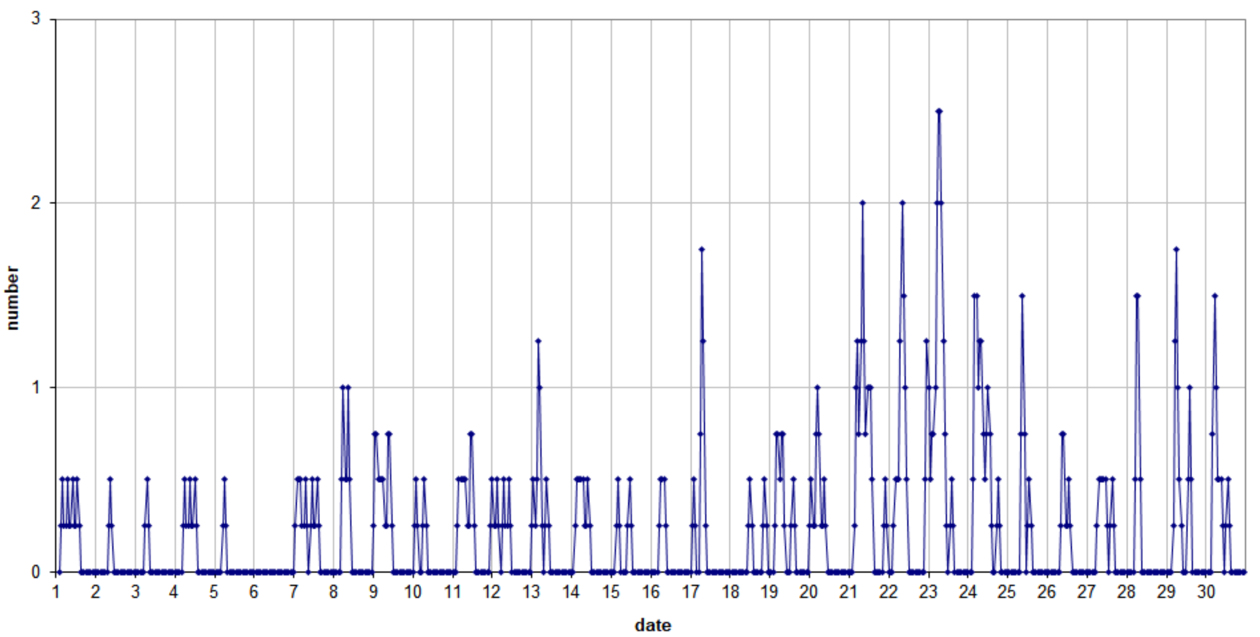
49.99MHz - RadioMeteors April 2021 number of reflections >10 seconds per hour (weighted average) Felix Verbelen (Kampenhout)
