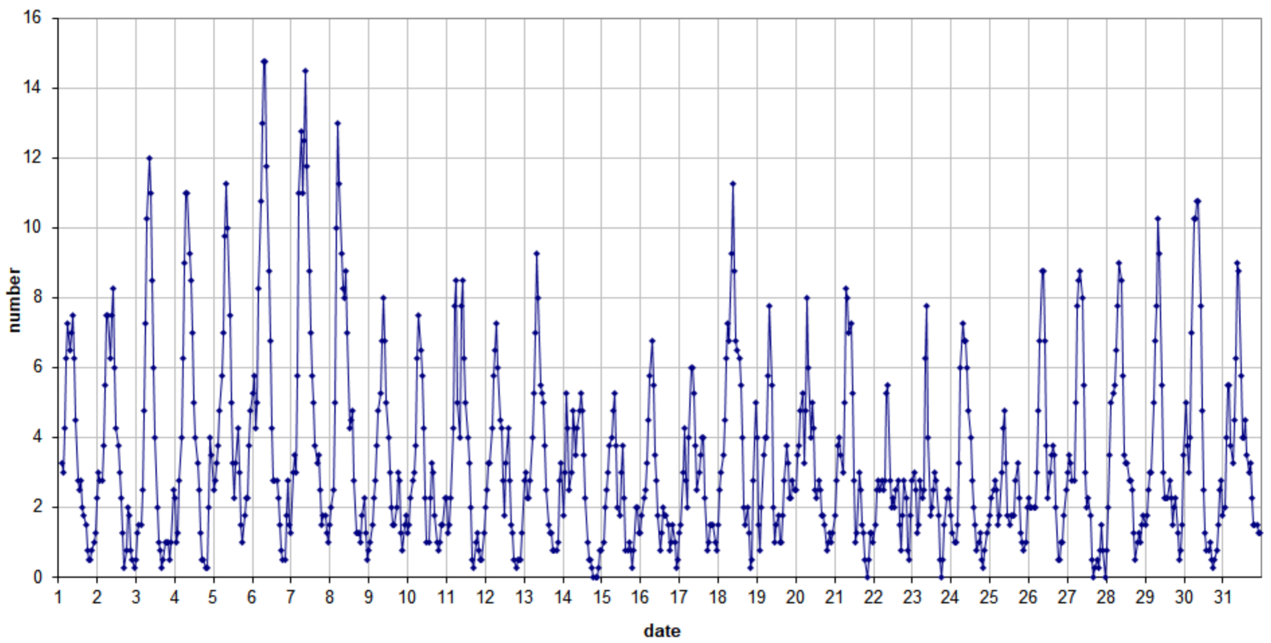
49.99MHz - RadioMeteors May 2021 number of overdense reflections per hour (weighted average) Felix Verbelen (Kamphenhout)
