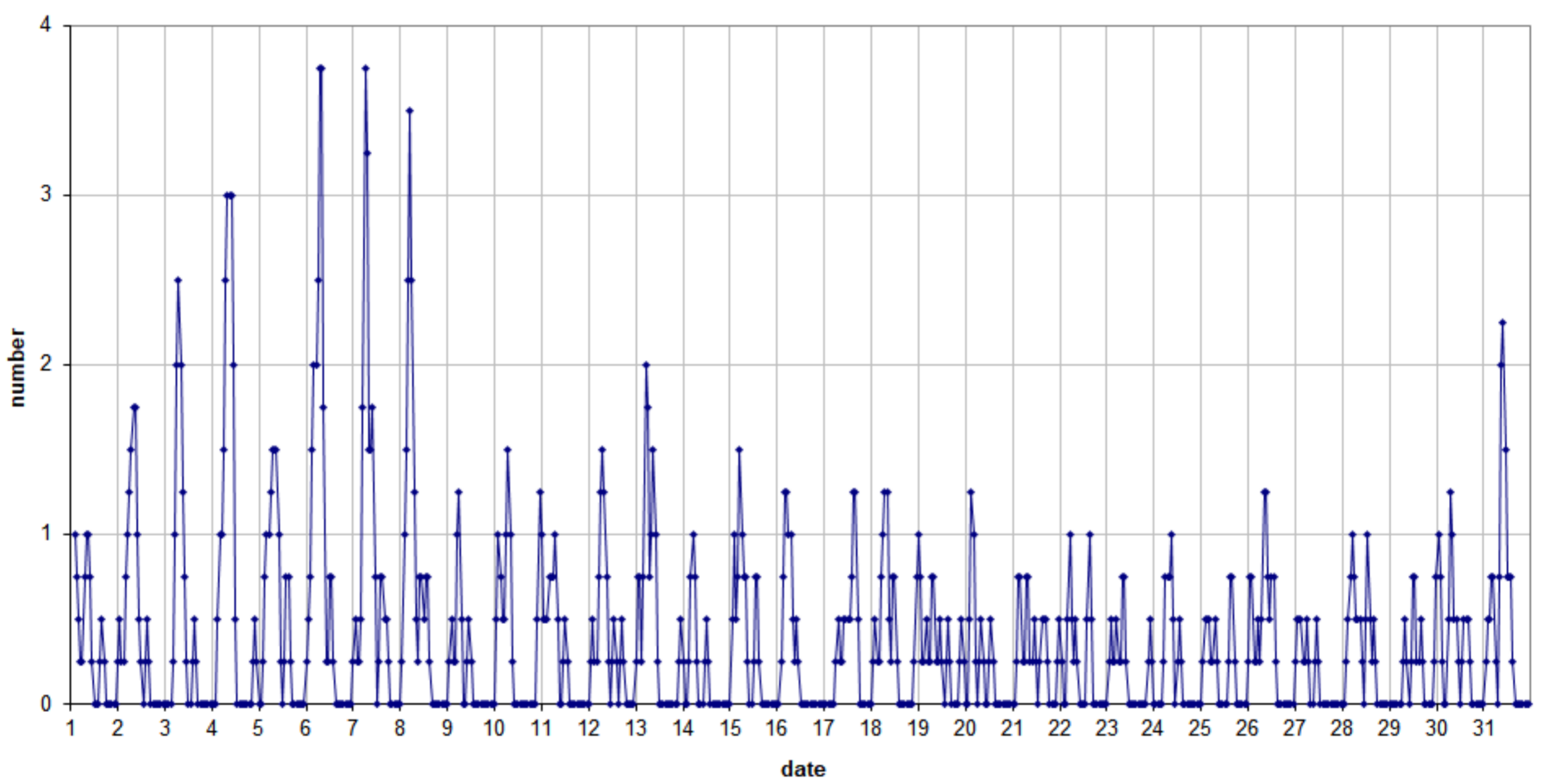
49.99MHz - RadioMeteors May 2021 number of reflections >10 seconds per hour (weighted average) Felix Verbelen (Kamphenhout)
