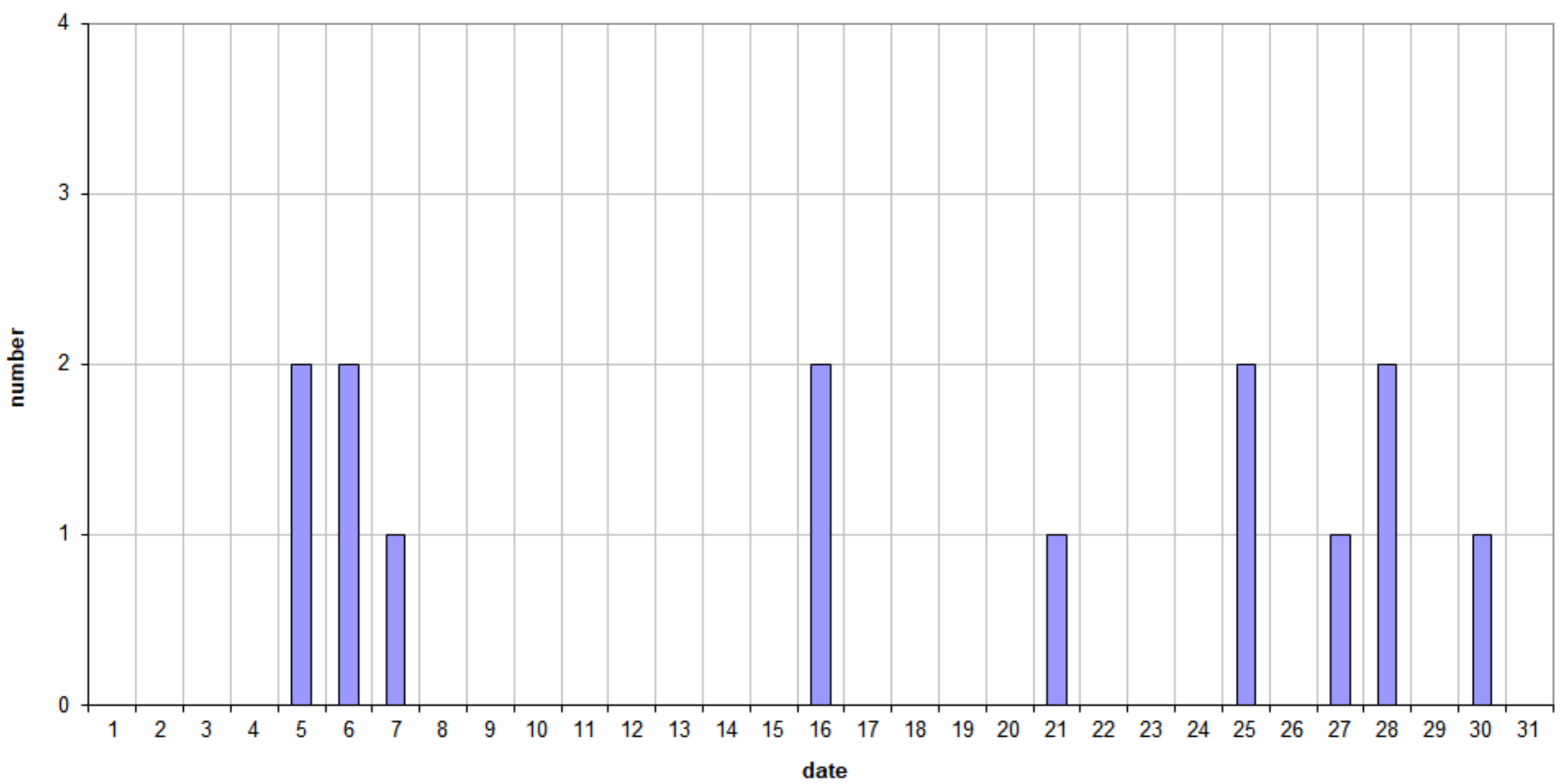
49.99MHz - RadioMeteors July 2021 daily totals of reflections longer than 1 minute Felix Verbelen (Kamphenhout)
