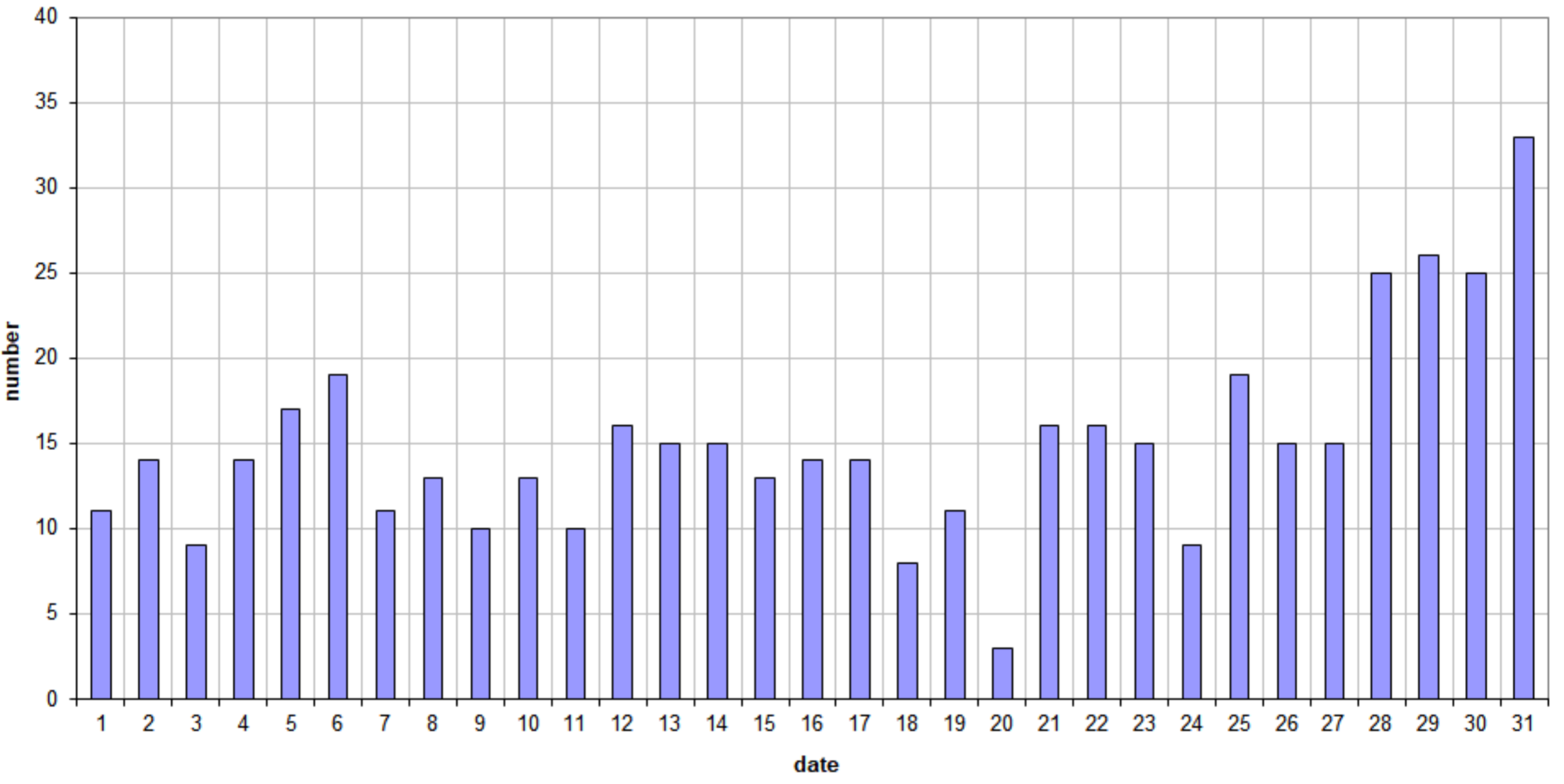
49.99MHz - RadioMeteors July 2021 daily totals of reflections longer than 10 seconds Felix Verbelen (Kamphenhout)
