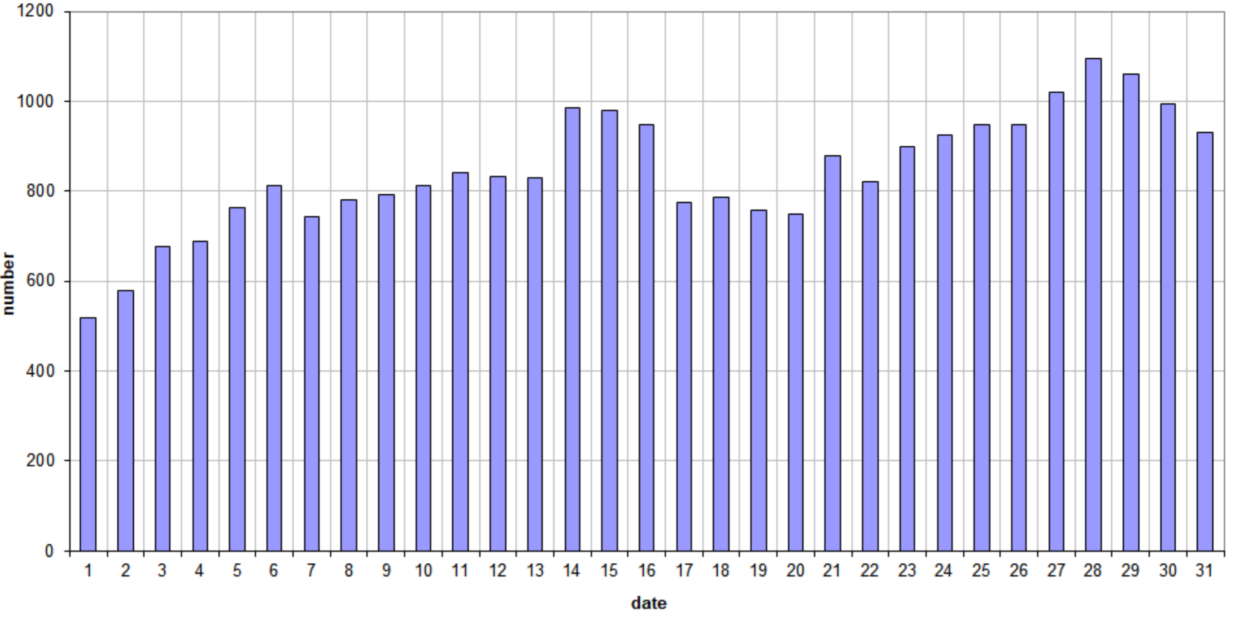
49.99MHz - RadioMeteors July 2021 daily totals of "all" reflections (automatic count_Mettel5_7Hz) Felix Verbelen (Kamphenhout)
