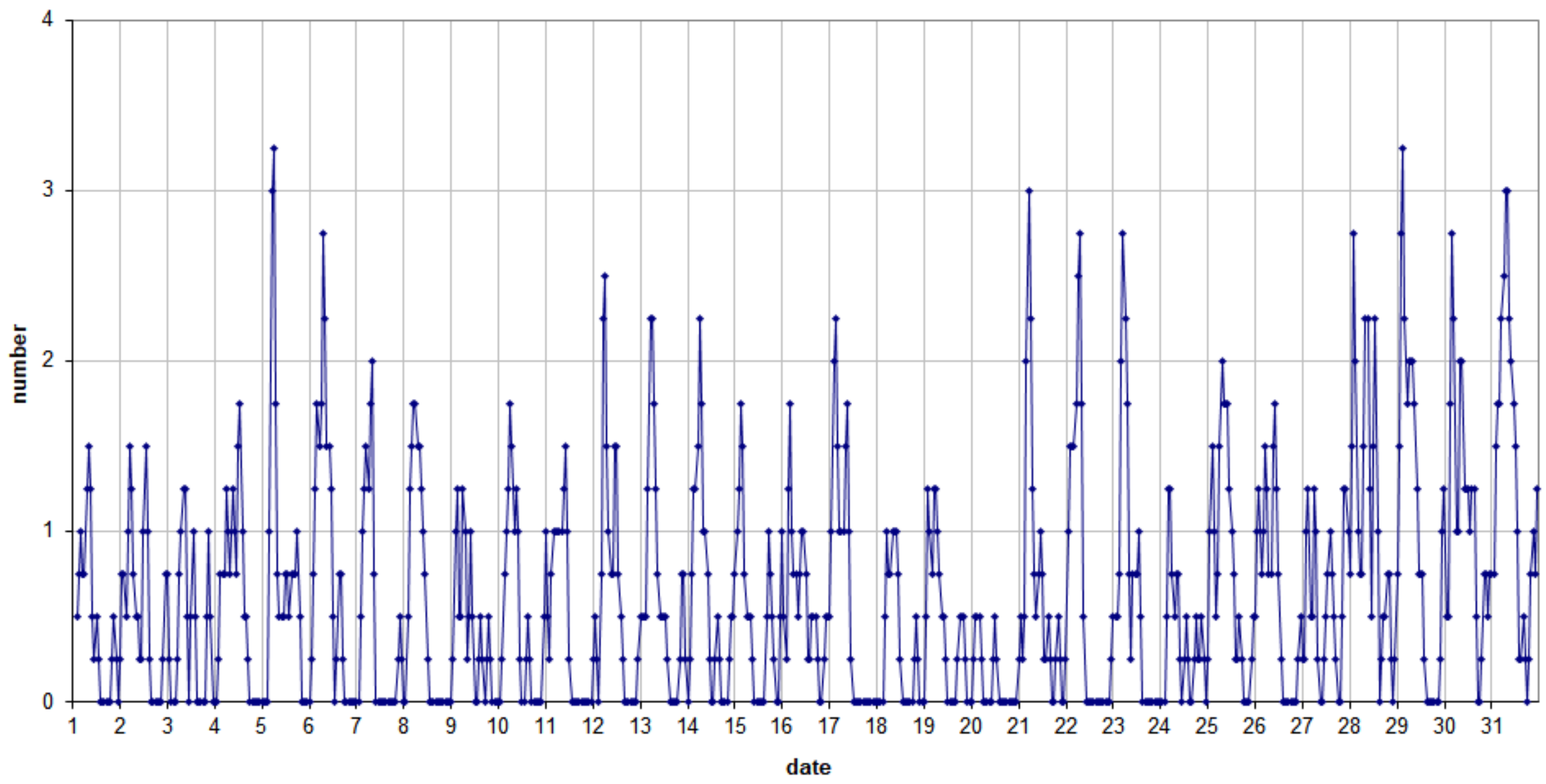
49.99MHz - RadioMeteors July 2021 number of reflections >10 seconds per hour (weighted average) Felix Verbelen (Kamphenhout)
