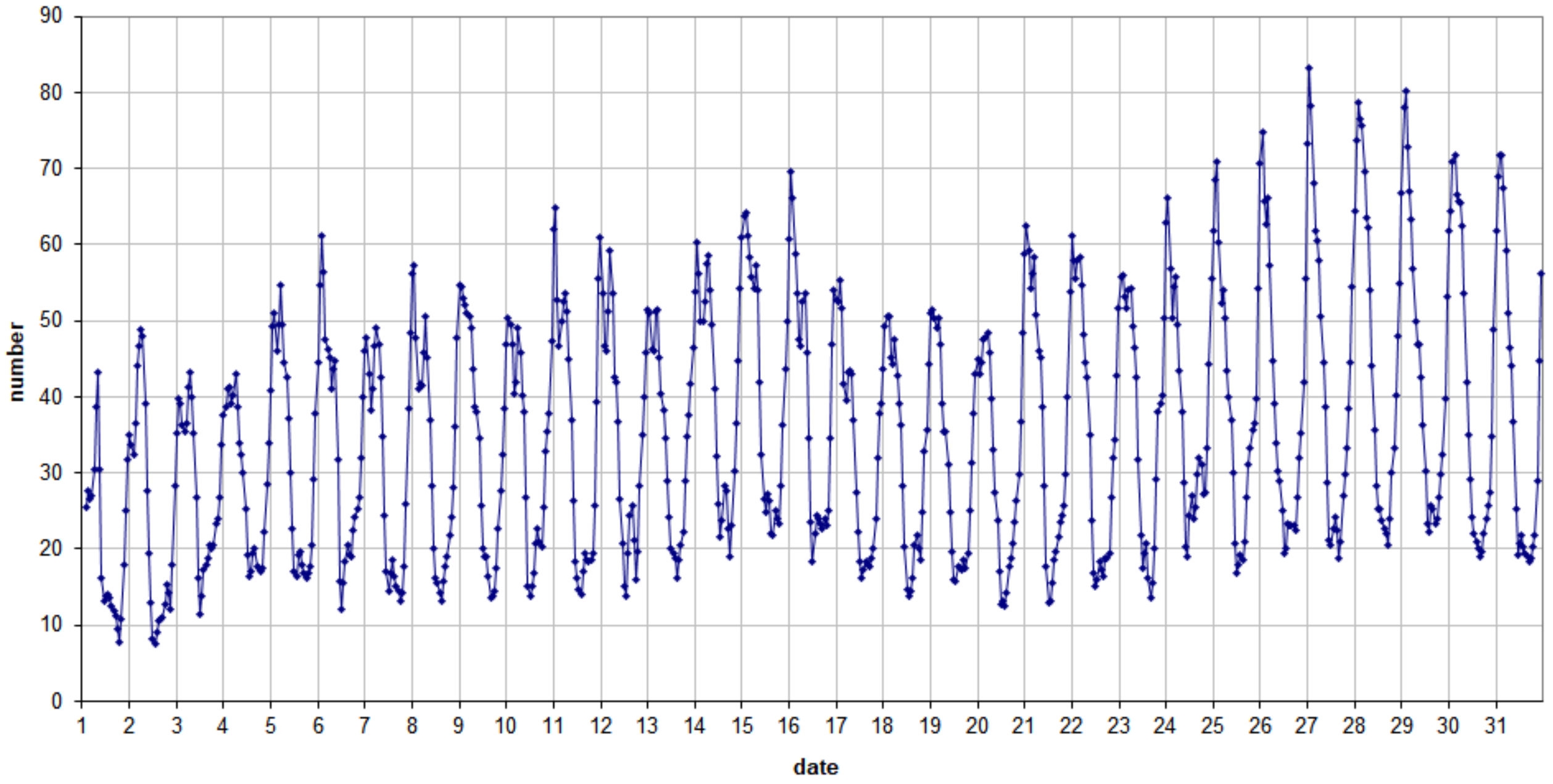
49.99 MHz - RadioMeteors July 2021 number of "all" reflections per hour (weighted average) (automatic count_Mettel5_7Hz) Felix Verbelen (Kamphenhout)
