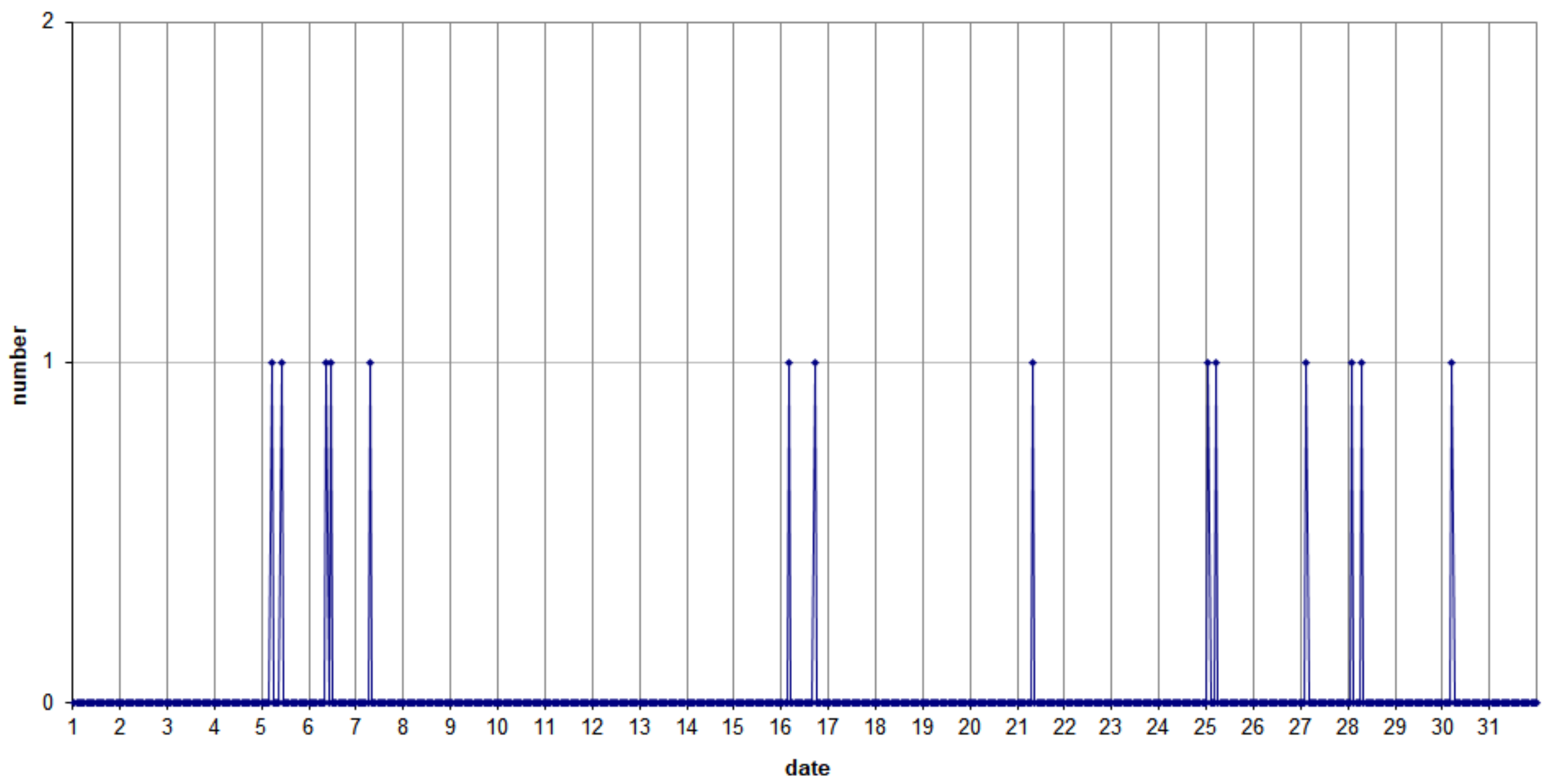
49.99MHz - RadioMeteors July 2021 hourly totals of overdense reflections longer than 1 minute Felix Verbelen (Kamphenhout/BE)
