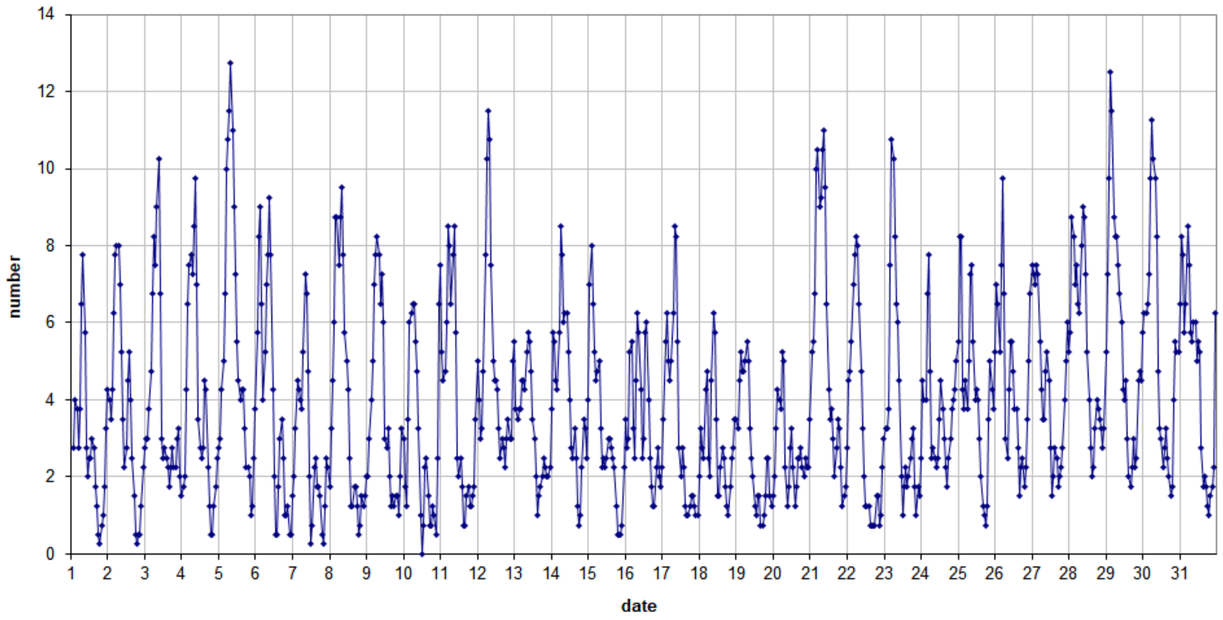
49.99MHz - RadioMeteors July 2021 number of overdense reflections per hour (weighted average) Felix Verbelen (Kamphenhout)
