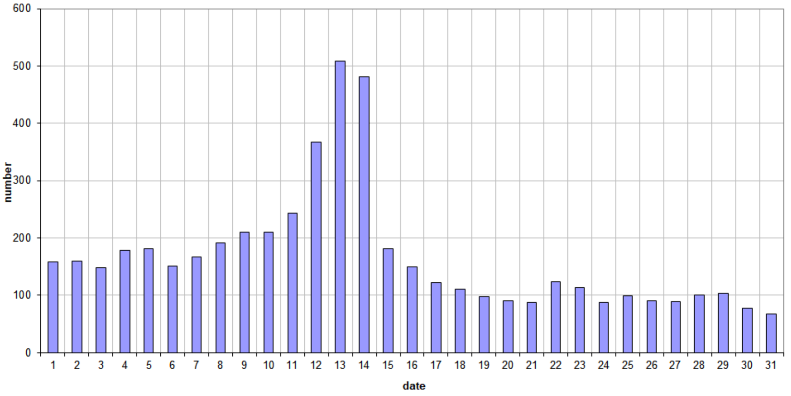
49.99MHz - RadioMeteors August 2021 daily totals of all overdense reflections Felix Verbelen (Kamphenhout)
