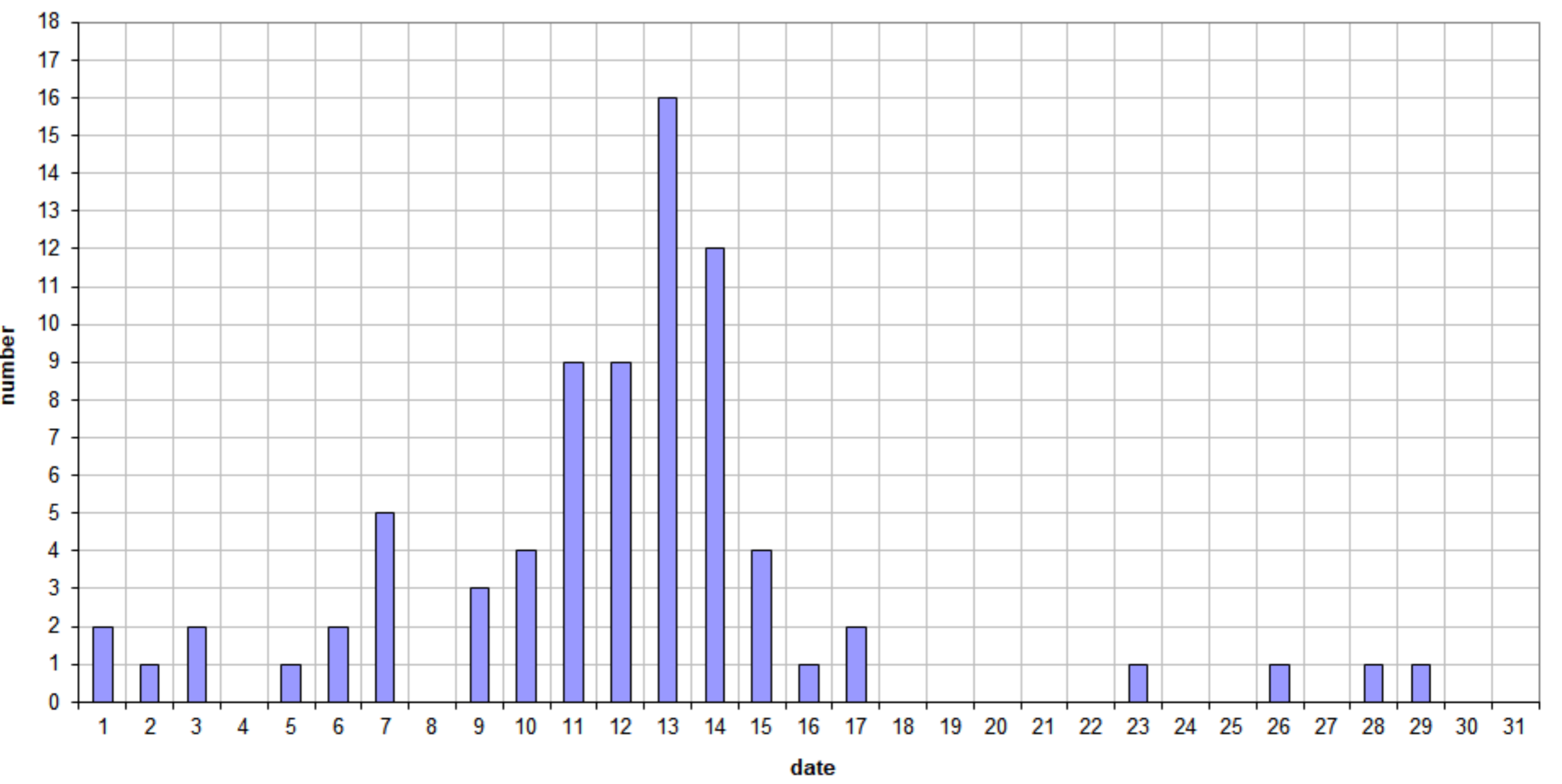
49.99MHz - RadioMeteors August 2021 daily totals of reflections longer than 1 minute Felix Verbelen (Kamphenhout)
