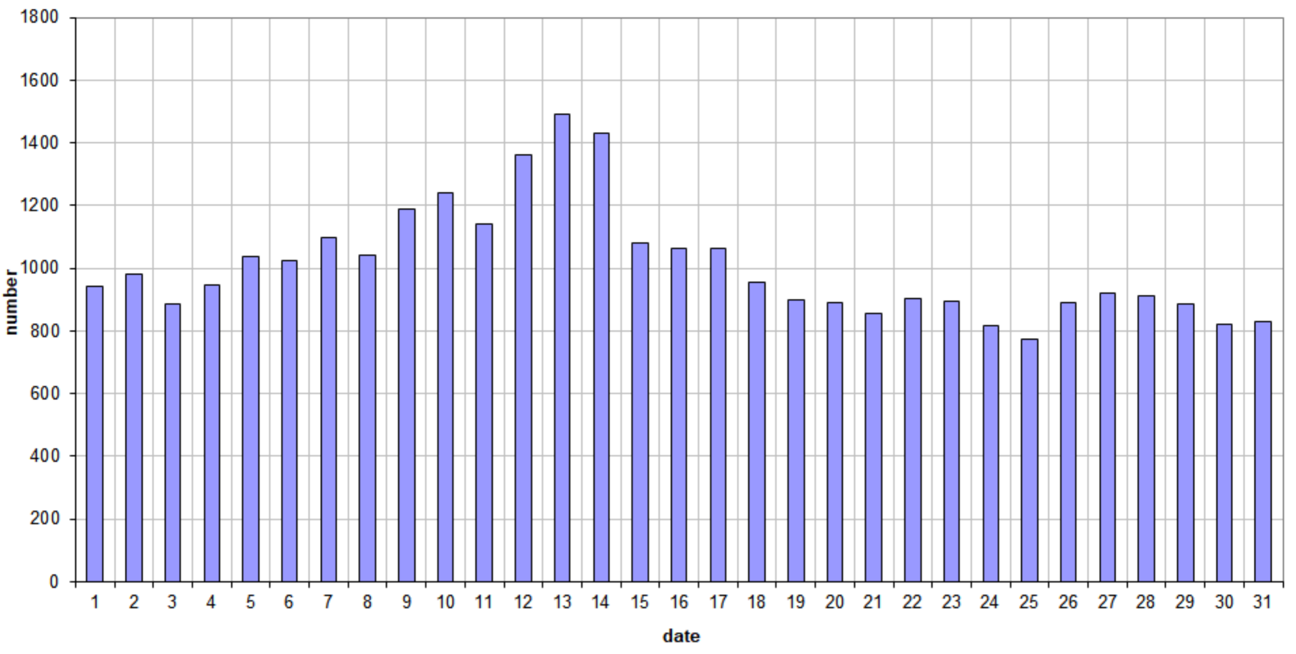
49.99MHz - RadioMeteors August 2021 daily totals of "all" reflections (automatic count_Mettel5_7Hz) Felix Verbelen (Kamphenhout)
