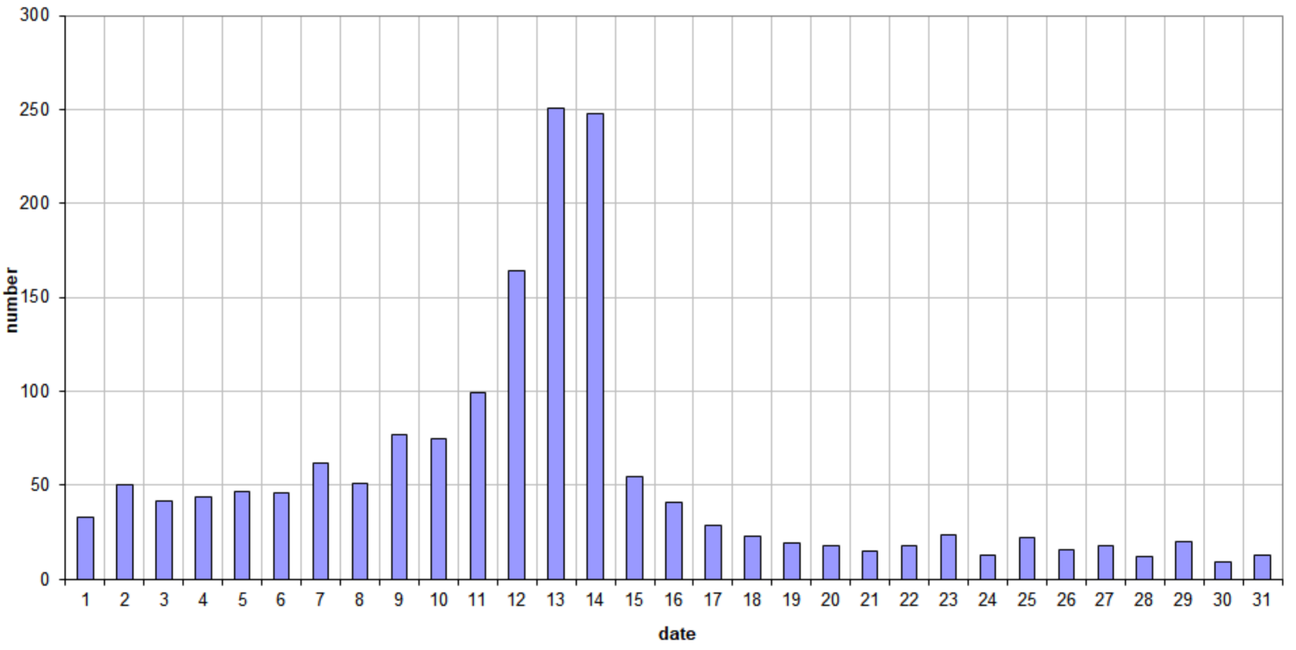
49.99MHz - RadioMeteors August 2021 daily totals of reflections longer than 10 seconds Felix Verbelen (Kamphenhout)
