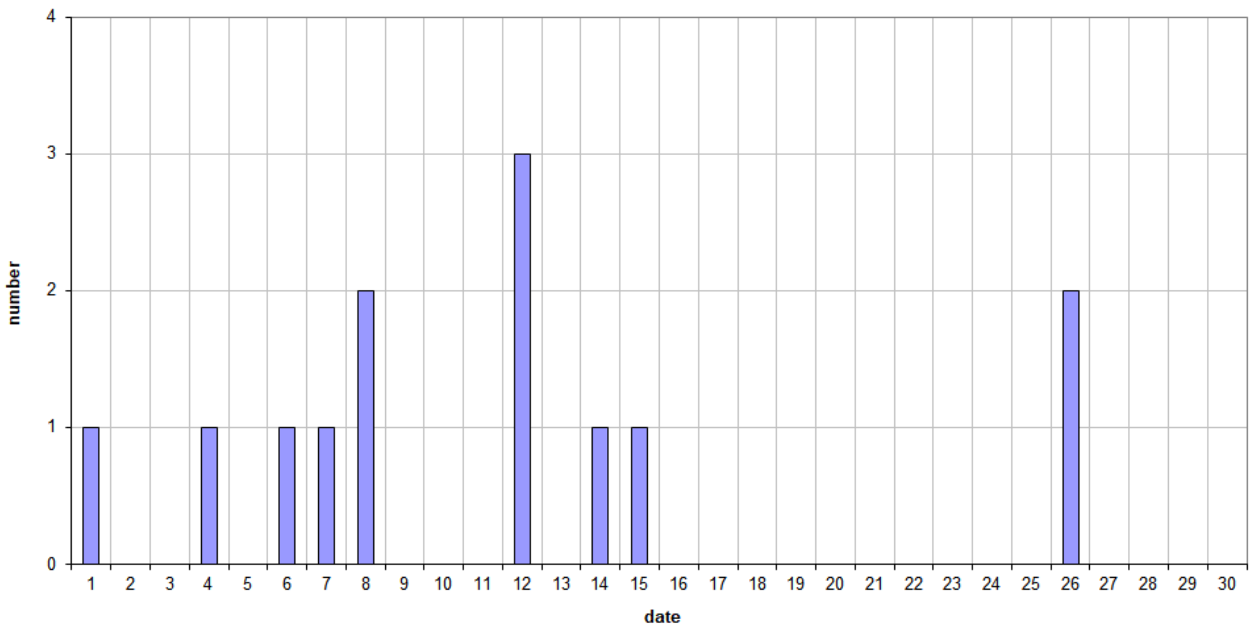
49.99MHz - RadioMeteors September 2021 daily totals of reflections longer than 1 minute Felix Verbelen (Kamphenhout)
