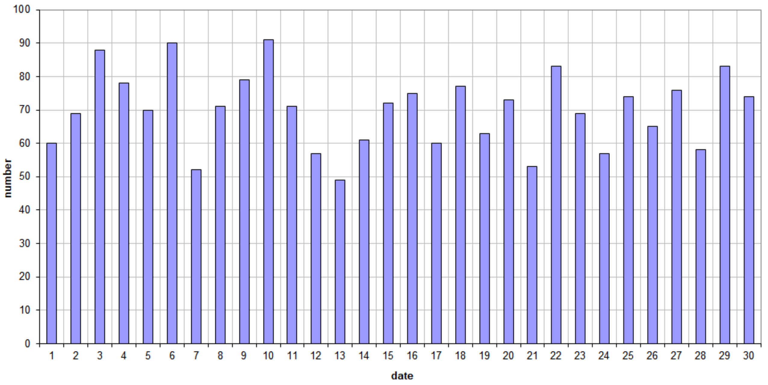
49.99MHz - RadioMeteors September 2021 daily totals of all overdense reflections Felix Verbelen (Kamphenhout)
