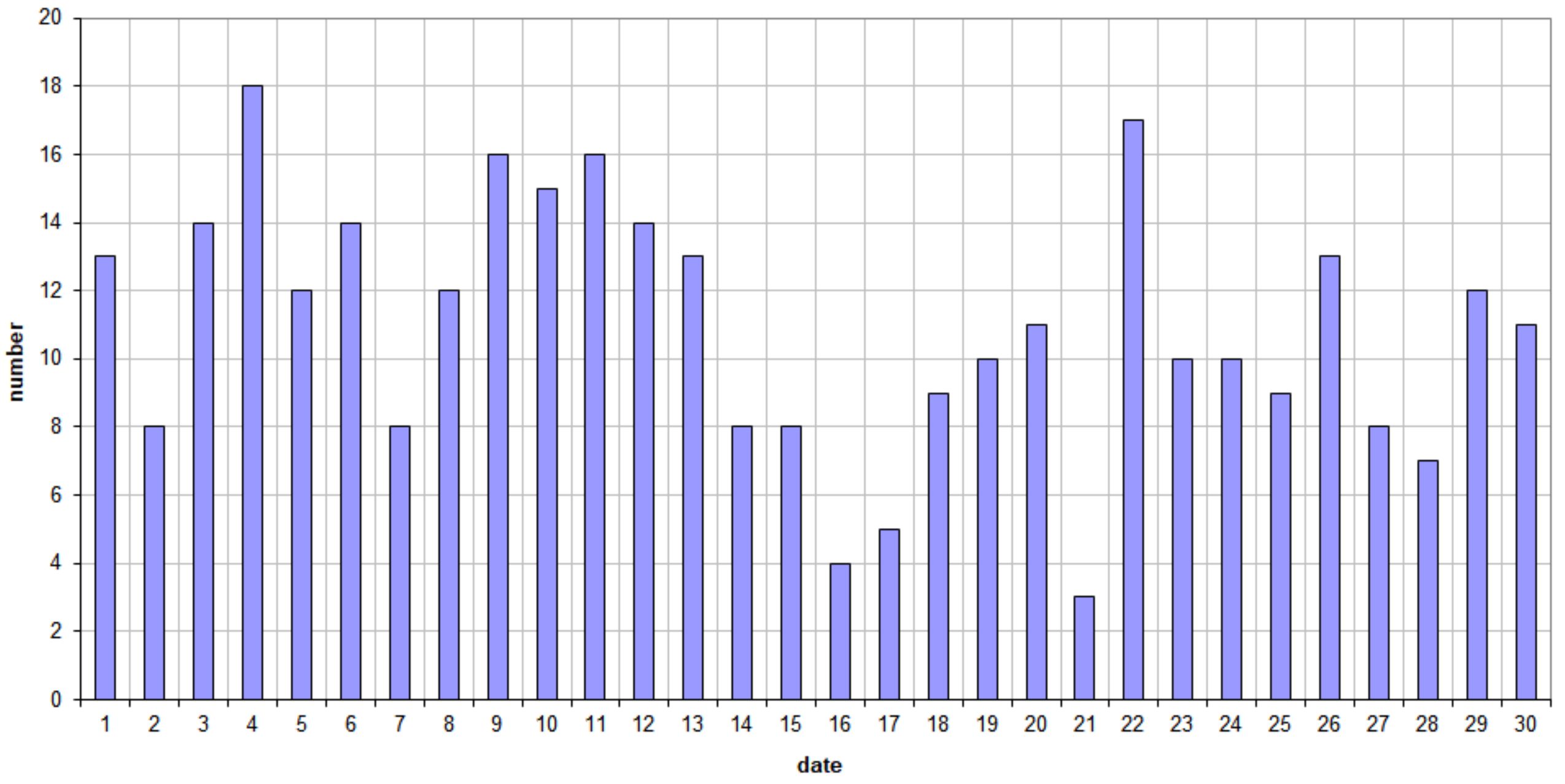
49.99MHz - RadioMeteors September 2021 daily totals of reflections longer than 10 seconds Felix Verbelen (Kamphenhout)
