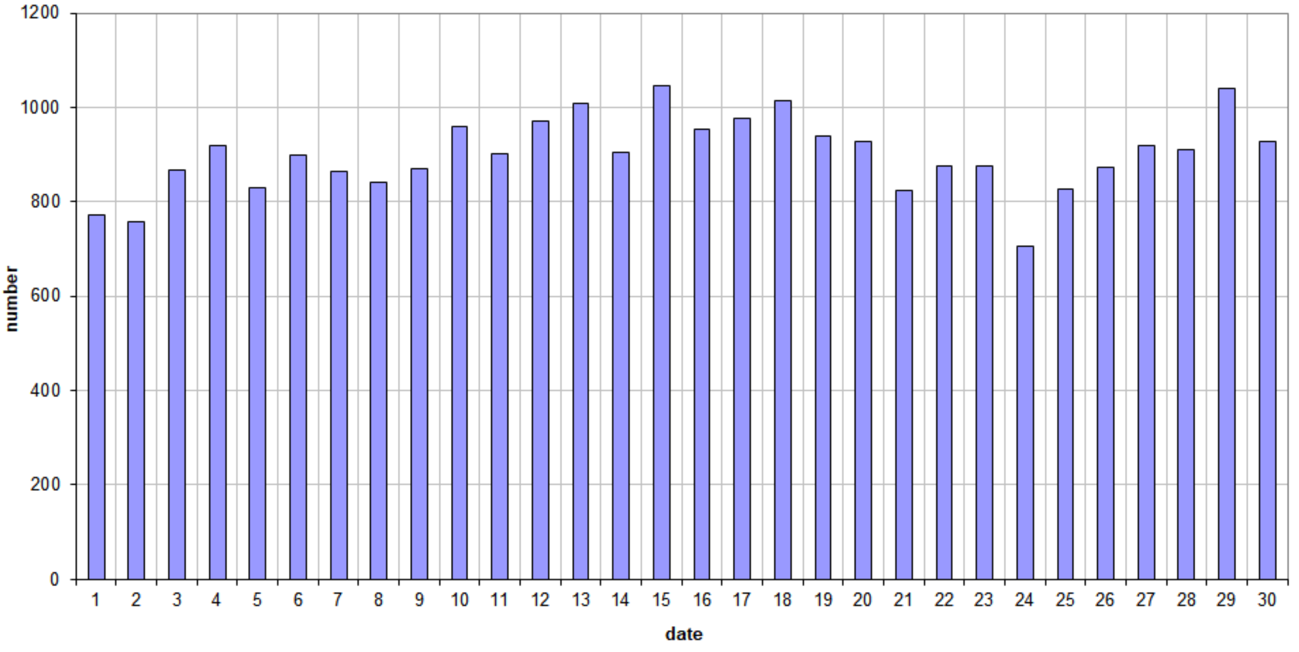
49.99MHz - RadioMeteors September 2021 daily totals of "all" reflections (automatic count_Mettel5_7Hz) Felix Verbelen (Kamphenhout)
