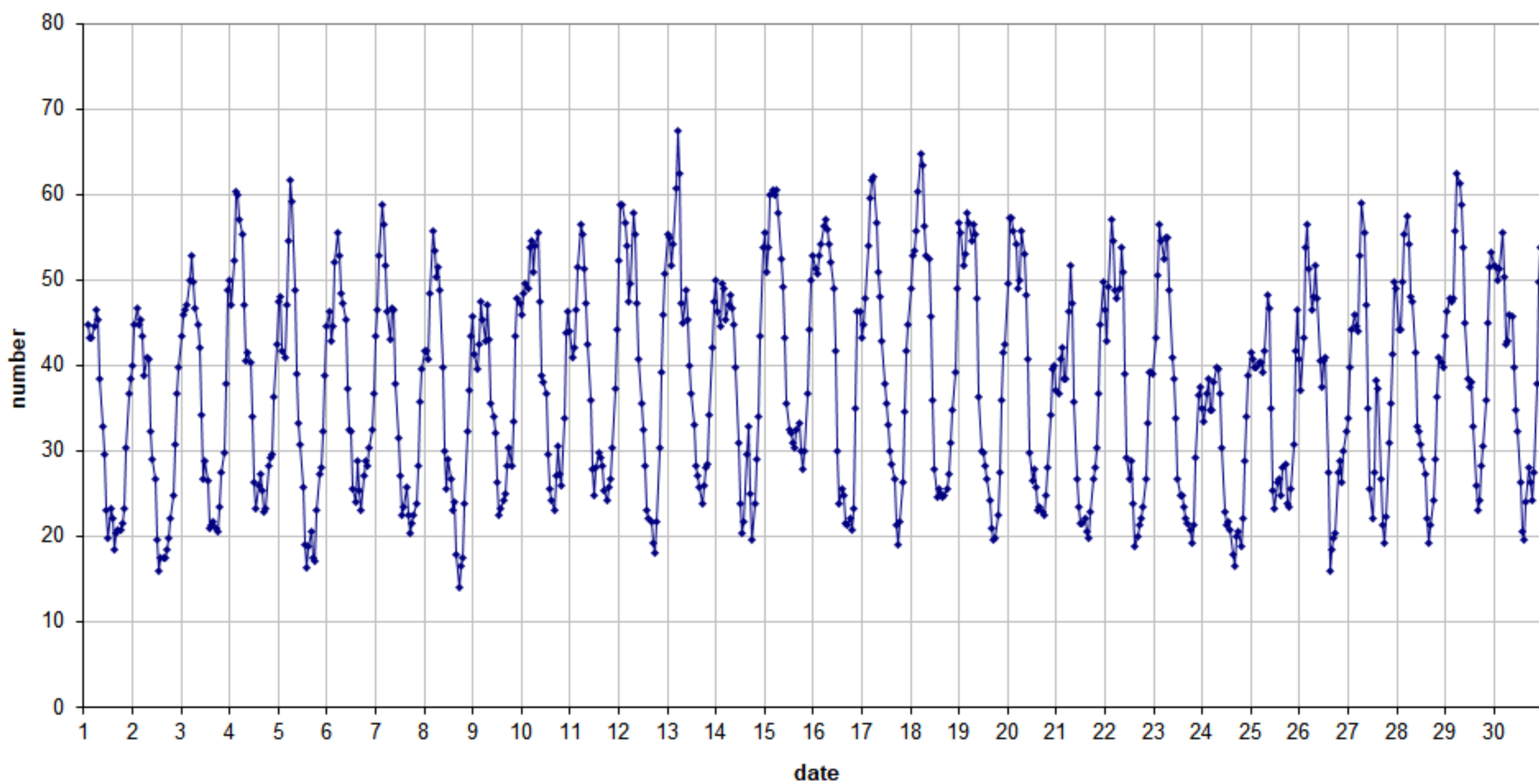
49.99 MHz - RadioMeteors September 2021 number of "all" reflections per hour (weighted average) (automatic count_Mettel5_7Hz) Felix Verbelen (Kampenhout)
