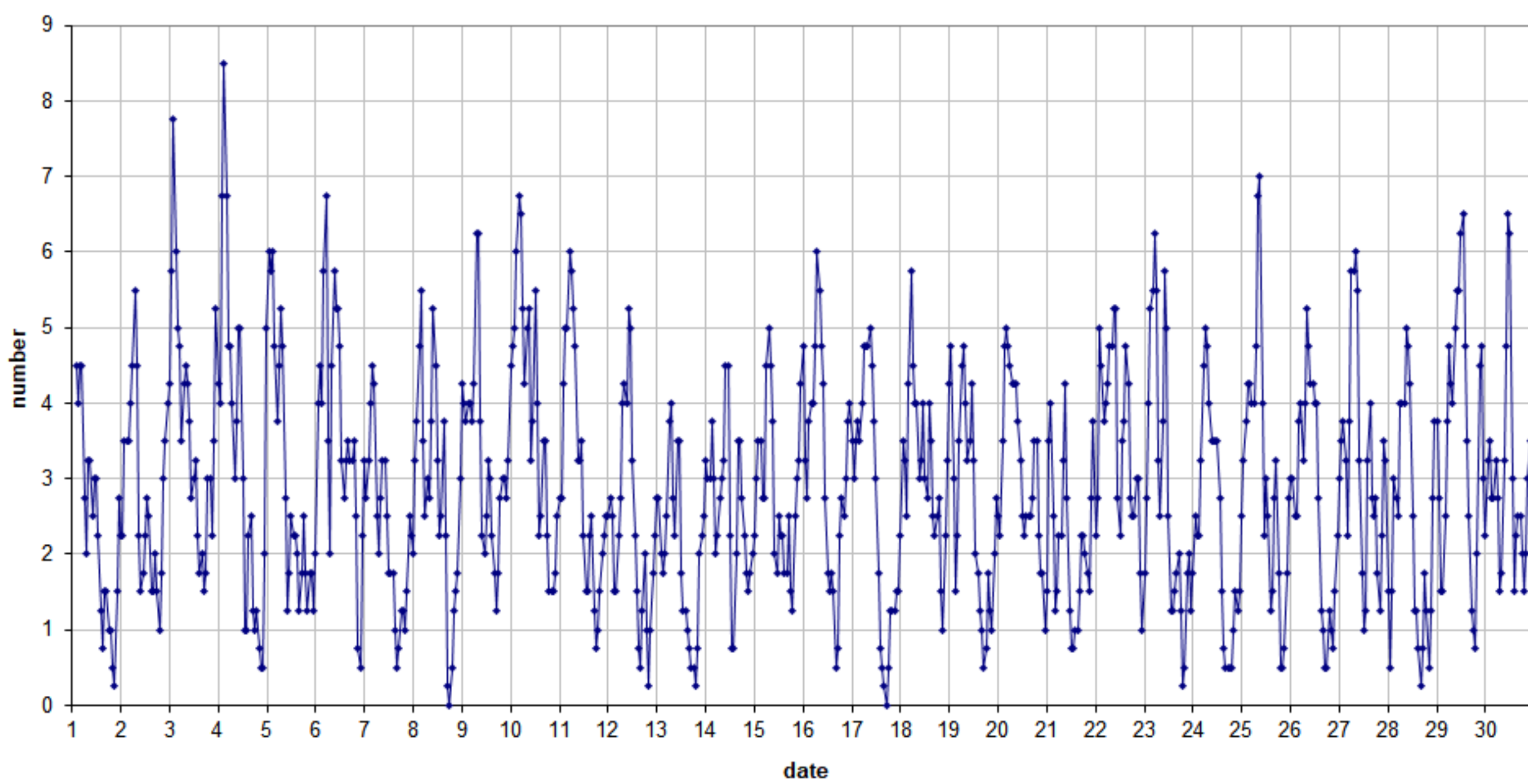
49.99MHz - RadioMeteors September 2021 number of overdense reflections per hour (weighted average) Felix Verbelen (Kampenhout)
