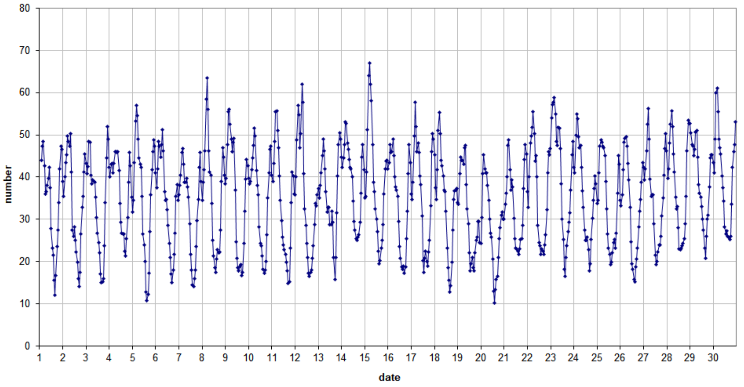
49.99 MHz - RadioMeteors November 2021 number of "all" reflections per hour (weighted average) (automatic count_Mettel5_7Hz) Felix Verbelen (Kamphenhout)
