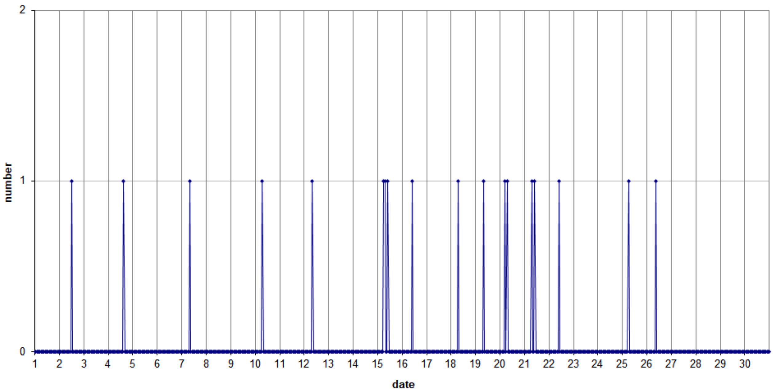
49.99MHz - RadioMeteors November 2021 hourly totals of overdense reflections longer than 1 minute Felix Verbelen (Kamphenhout/BE)
