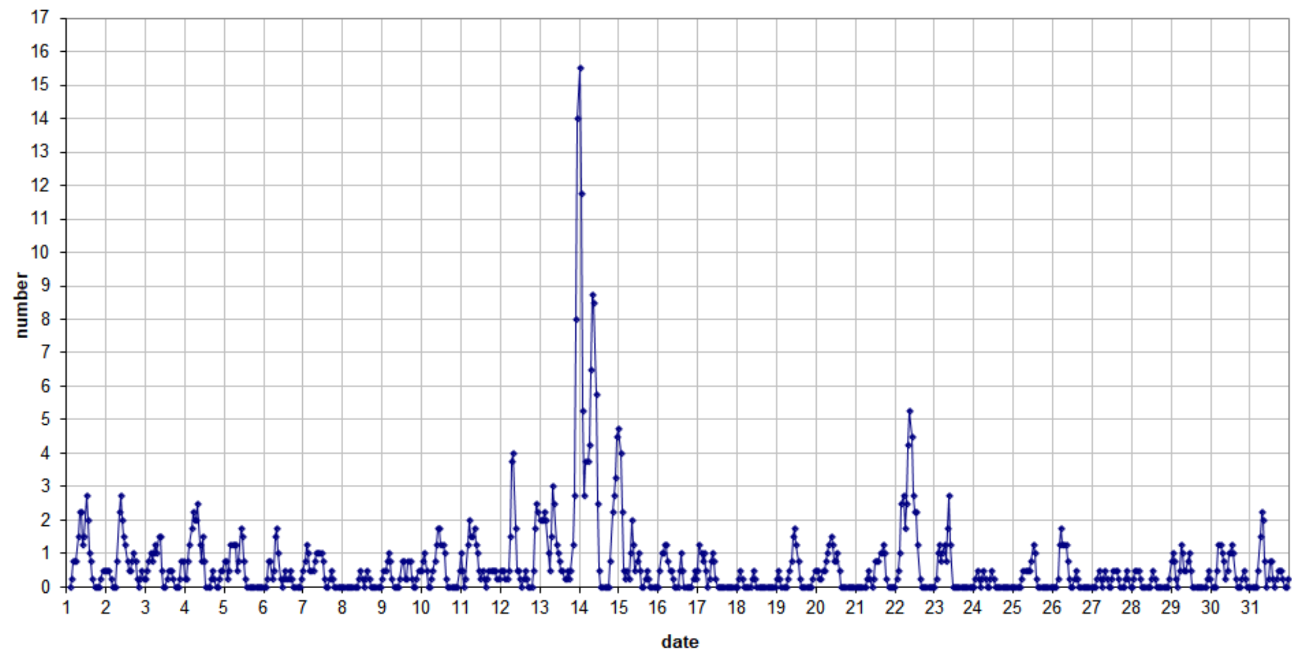
49.99MHz - RadioMeteors December 2021 number of reflections >10 seconds per hour (weighted average) Felix Verbelen (Kamphenhout)
