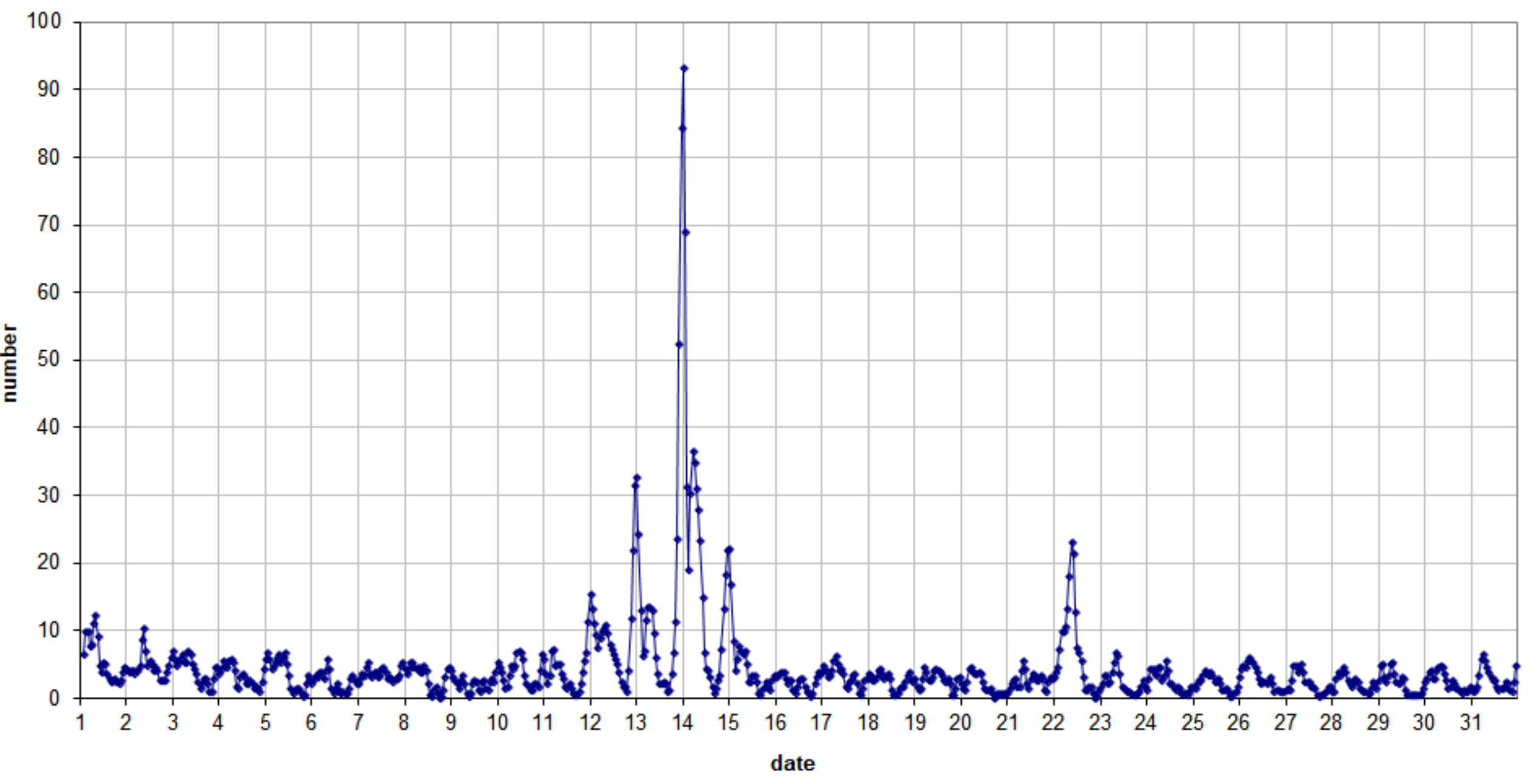
49.99MHz - RadioMeteors December 2021 number of overdense reflections per hour (weighted average) Felix Verbelen (Kamphenhout)
