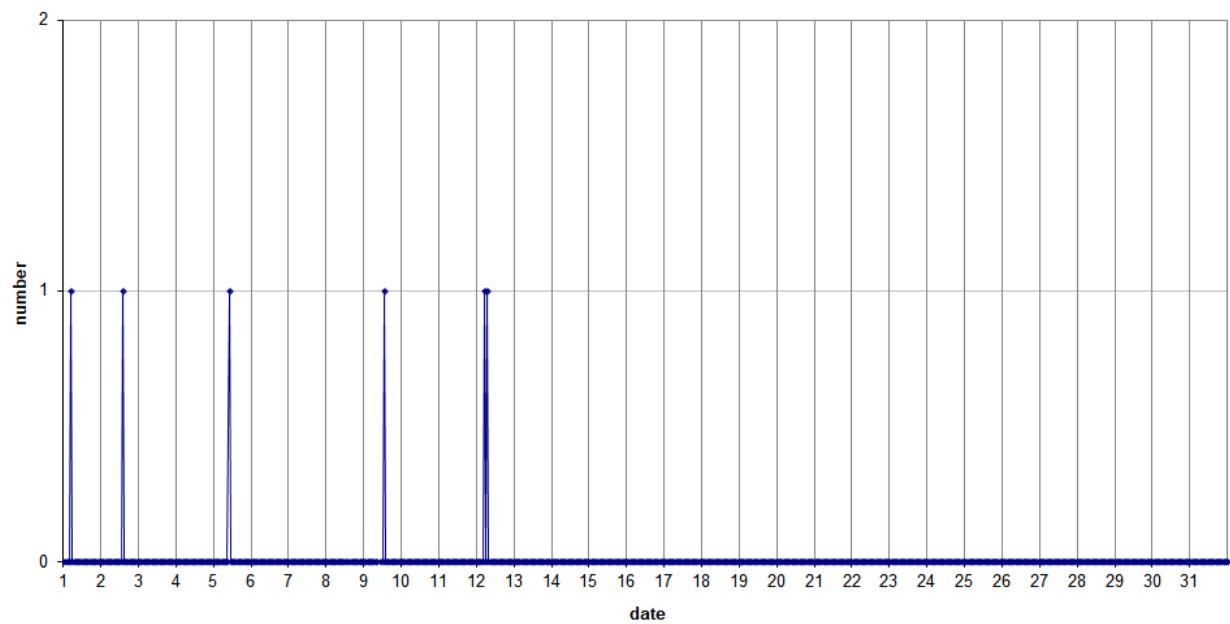
49.99MHz - RadioMeteors December 2021 hourly totals of overdense reflections longer than 1 minute Felix Verbelen (Kamphenhout/BE)
