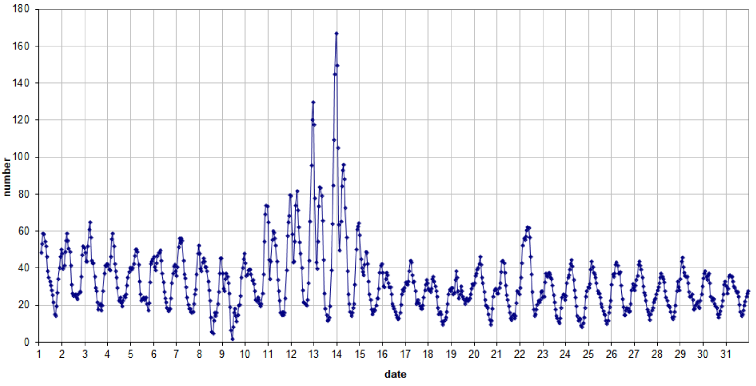
49.99 MHz - RadioMeteors December 2021 number of "all" reflections per hour (weighted average) (automatic count_Mettel5_7Hz) Felix Verbelen (Kamphenhout)
