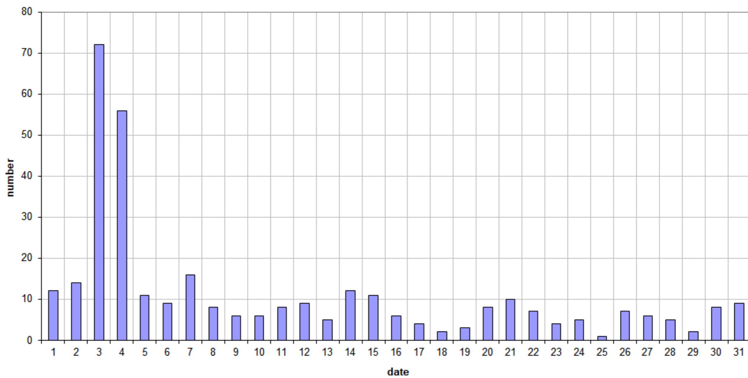
49.99MHz - RadioMeteors January 2022 daily totals of reflections longer than 10 seconds Felix Verbelen (Kampenhout)
