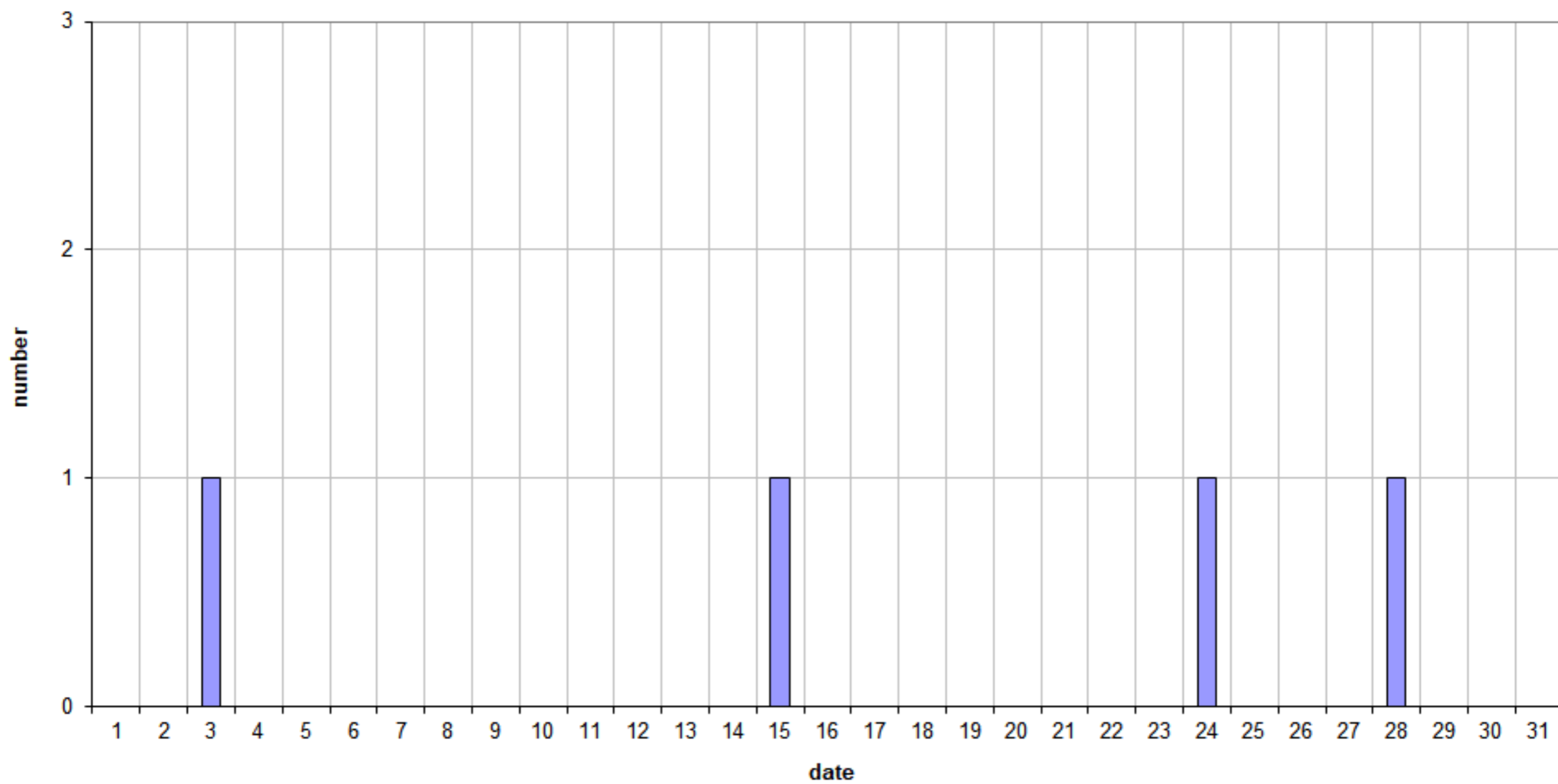
49.99MHz - RadioMeteors January 2022 daily totals of reflections longer than 1 minute Felix Verbelen (Kampenhout)
