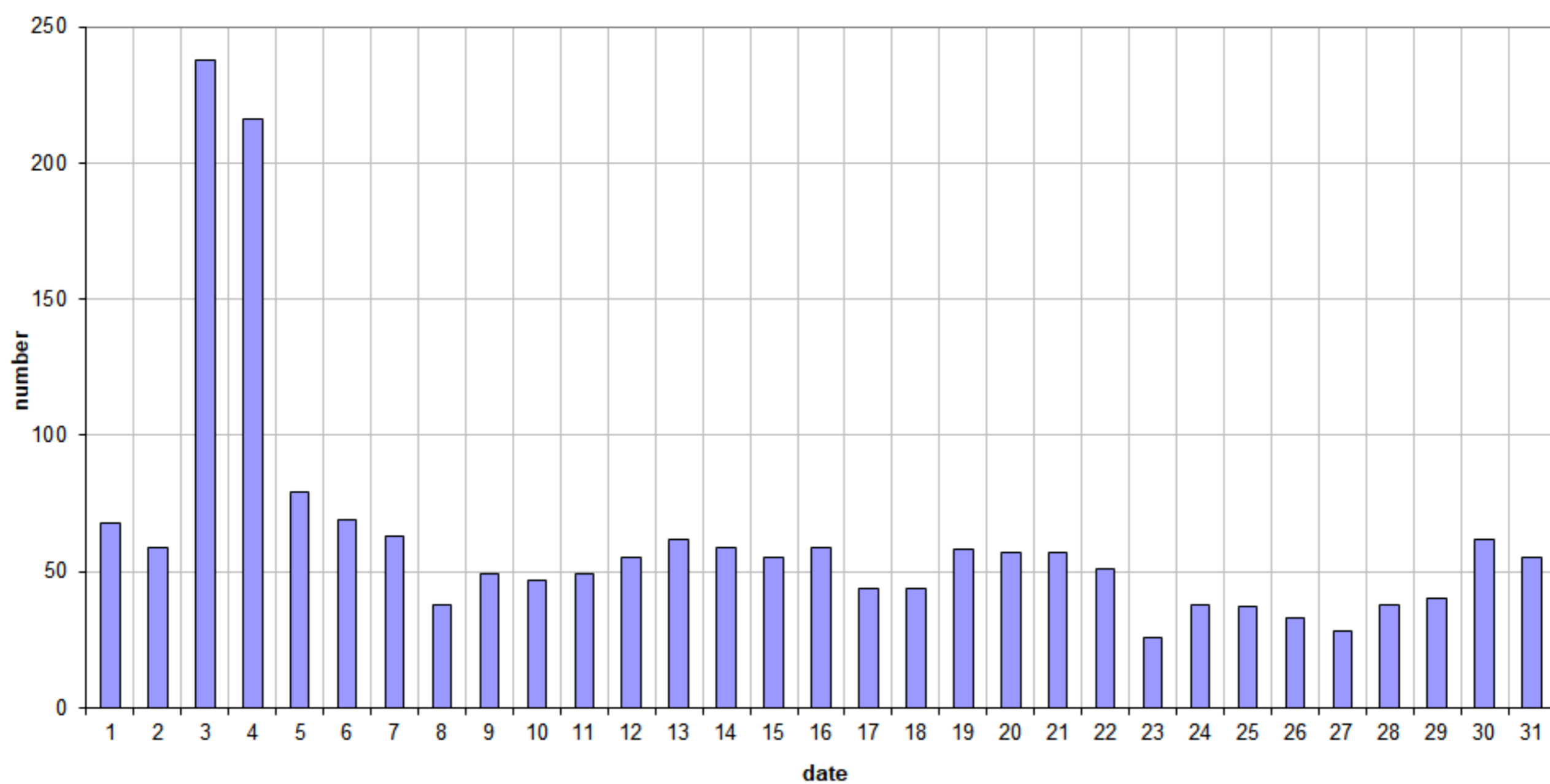
49.99MHz - RadioMeteors January 2022 daily totals of all overdense reflections Felix Verbelen (Kampenhout)
