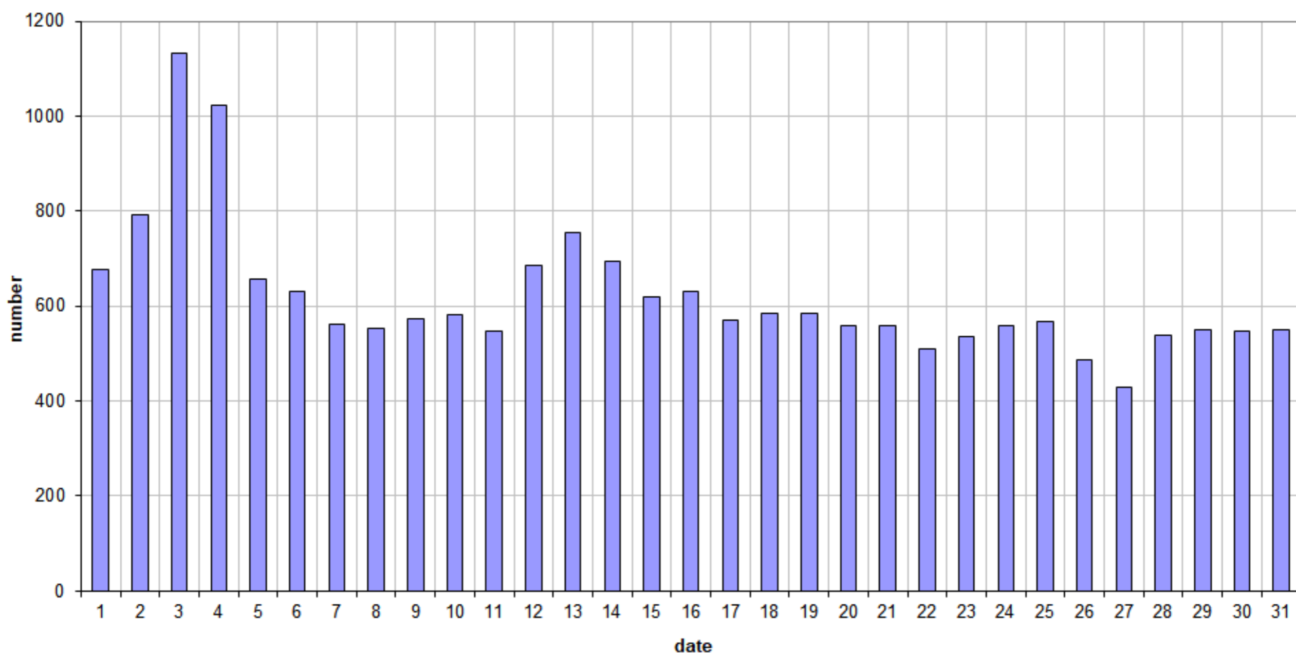
49.99MHz - RadioMeteors January 2022 daily totals of "all" reflections (automatic count_Mettel5_7Hz) Felix Verbelen (Kampenhout)
