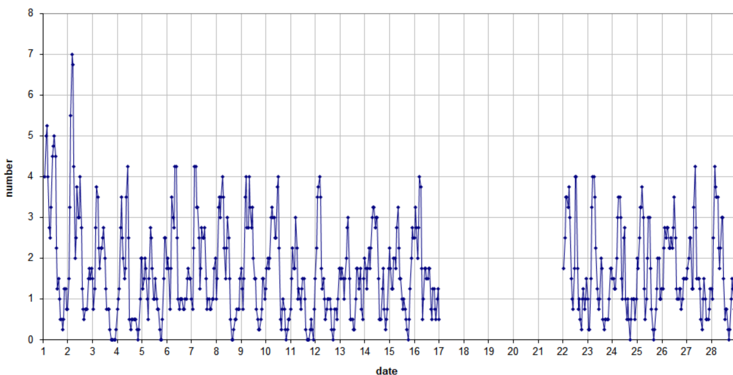
49.99MHz - RadioMeteors February 2022 number of overdense reflections per hour (weighted average) Felix Verbelen (Kamphenhout)
