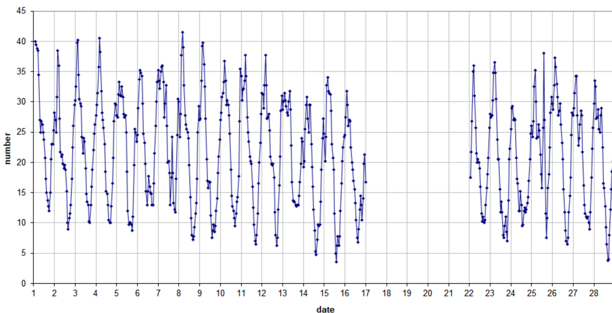
49.99 MHz - RadioMeteors February 2022 number of "all" reflections per hour (weighted average) (automatic count_Mette15_7Hz) Felix Verbelen (Kamphenhout)
