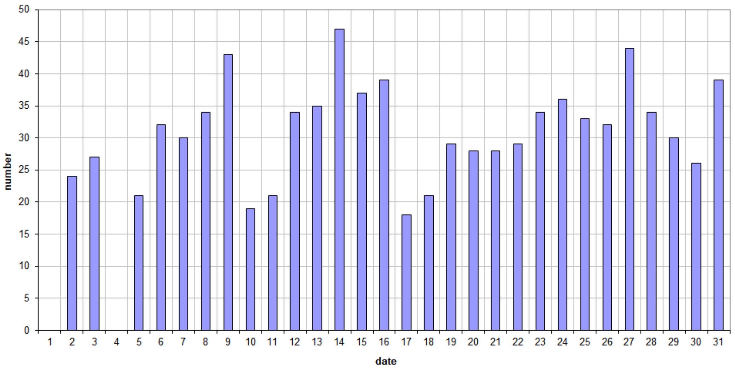
49.99MHz - RadioMeteors March 2022 daily totals of all overdense reflections Felix Verbelen (Kamphenhout)
