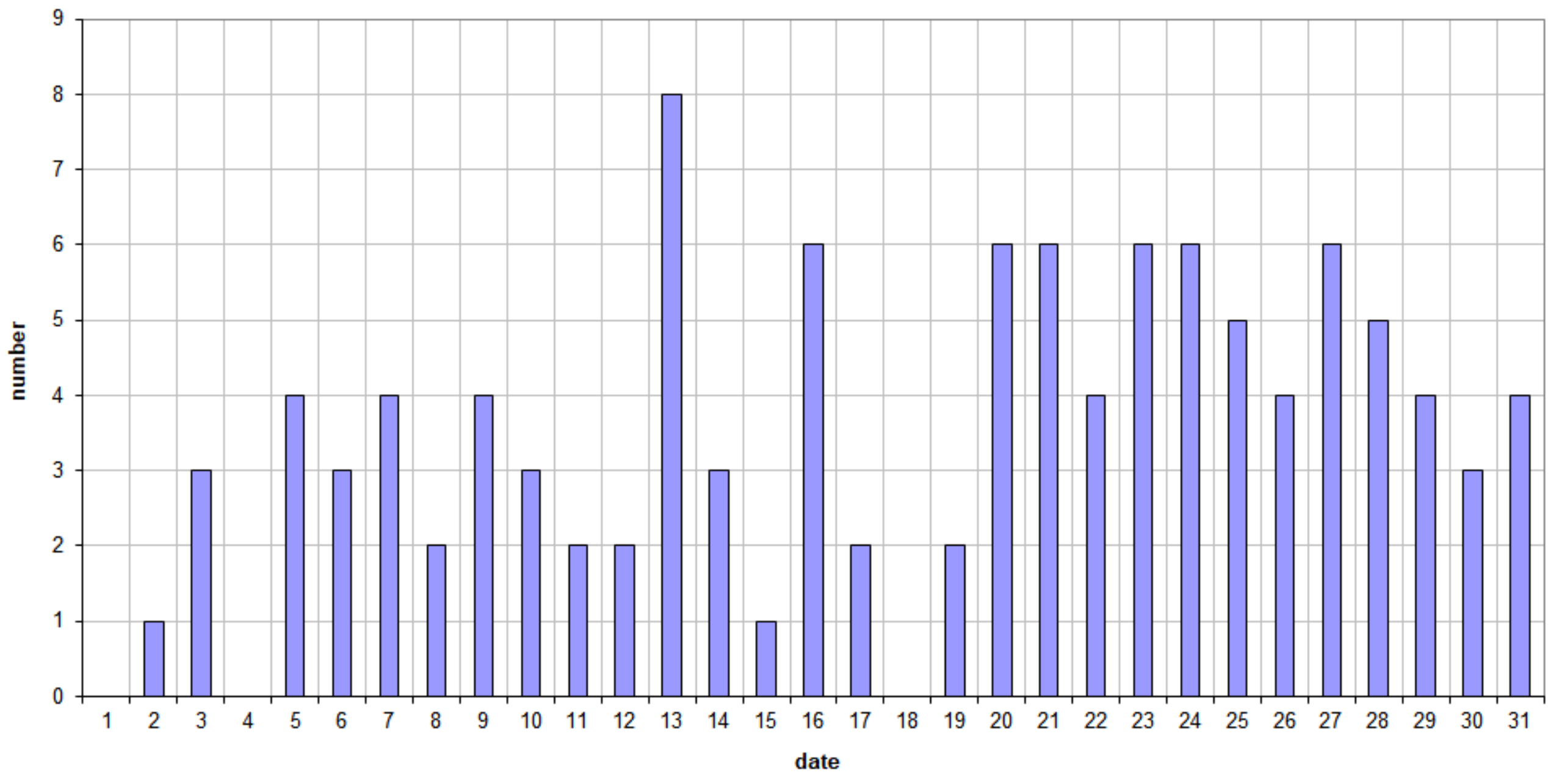
49.99MHz - RadioMeteors March 2022 daily totals of reflections longer than 10 seconds Felix Verbelen (Kamphenhout)
