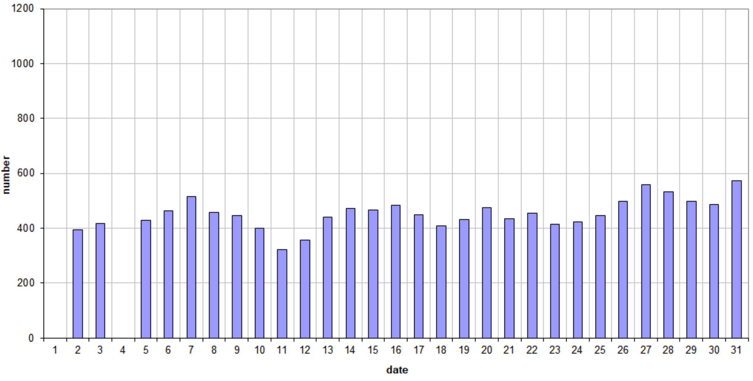
49.99MHz - RadioMeteors March 2022 daily totals of "all" reflections (automatic count_Mettel5_7Hz) Felix Verbelen (Kamphenhout)
