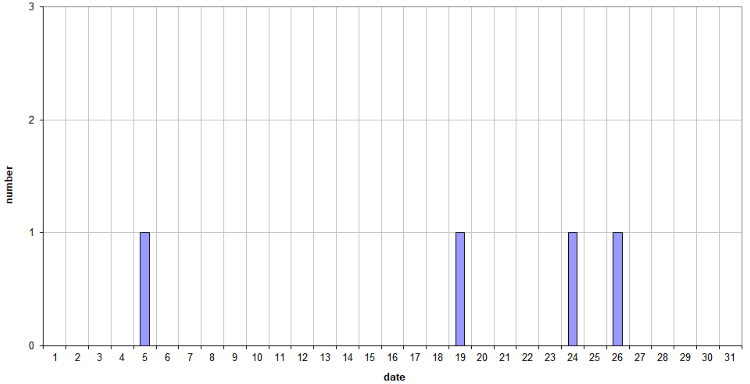
49.99MHz - RadioMeteors March 2022 daily totals of reflections longer than 1 minute Felix Verbelen (Kamphenhout)
