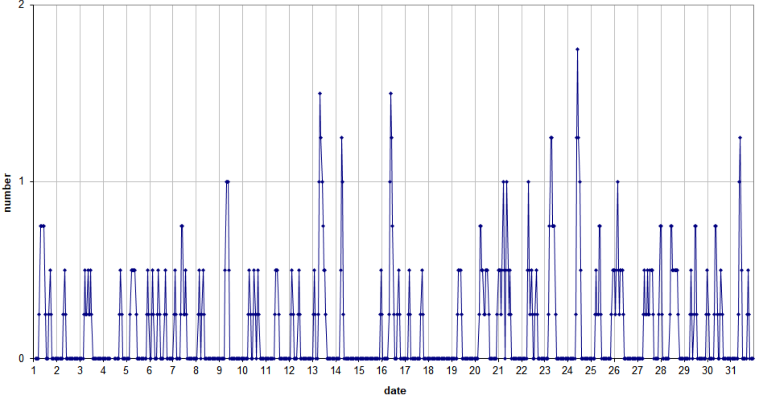
49.99MHz - RadioMeteors March 2022 number of reflections >10 seconds per hour (weighted average) Felix Verbelen (Kamphenhout)
