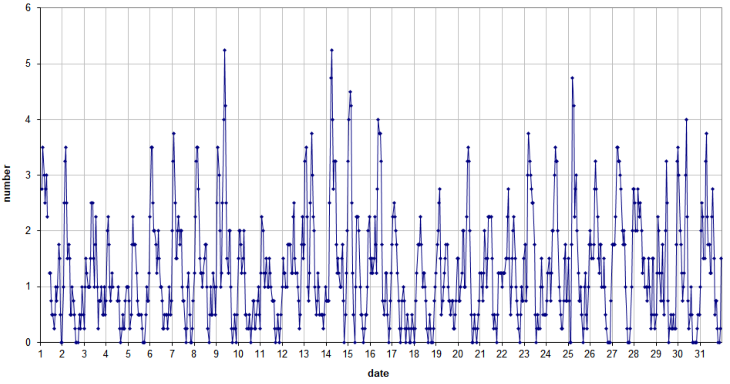
49.99MHz - RadioMeteors March 2022 number of overdense reflections per hour (weighted average) Felix Verbelen (Kamphenhout)
