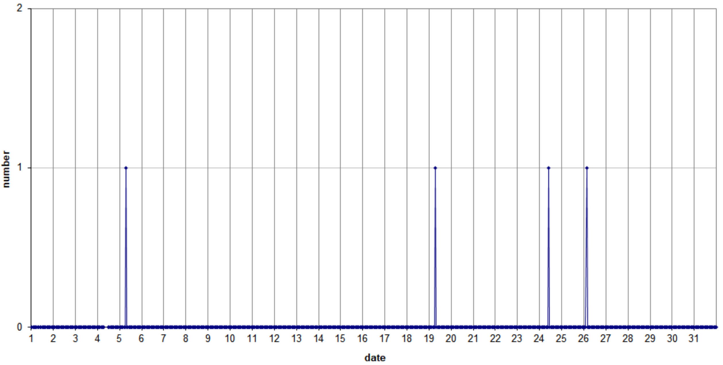
49.99MHz - RadioMeteors March 2022 hourly totals of overdense reflections longer than 1 minute Felix Verbelen (Kamphenhout/BE)
