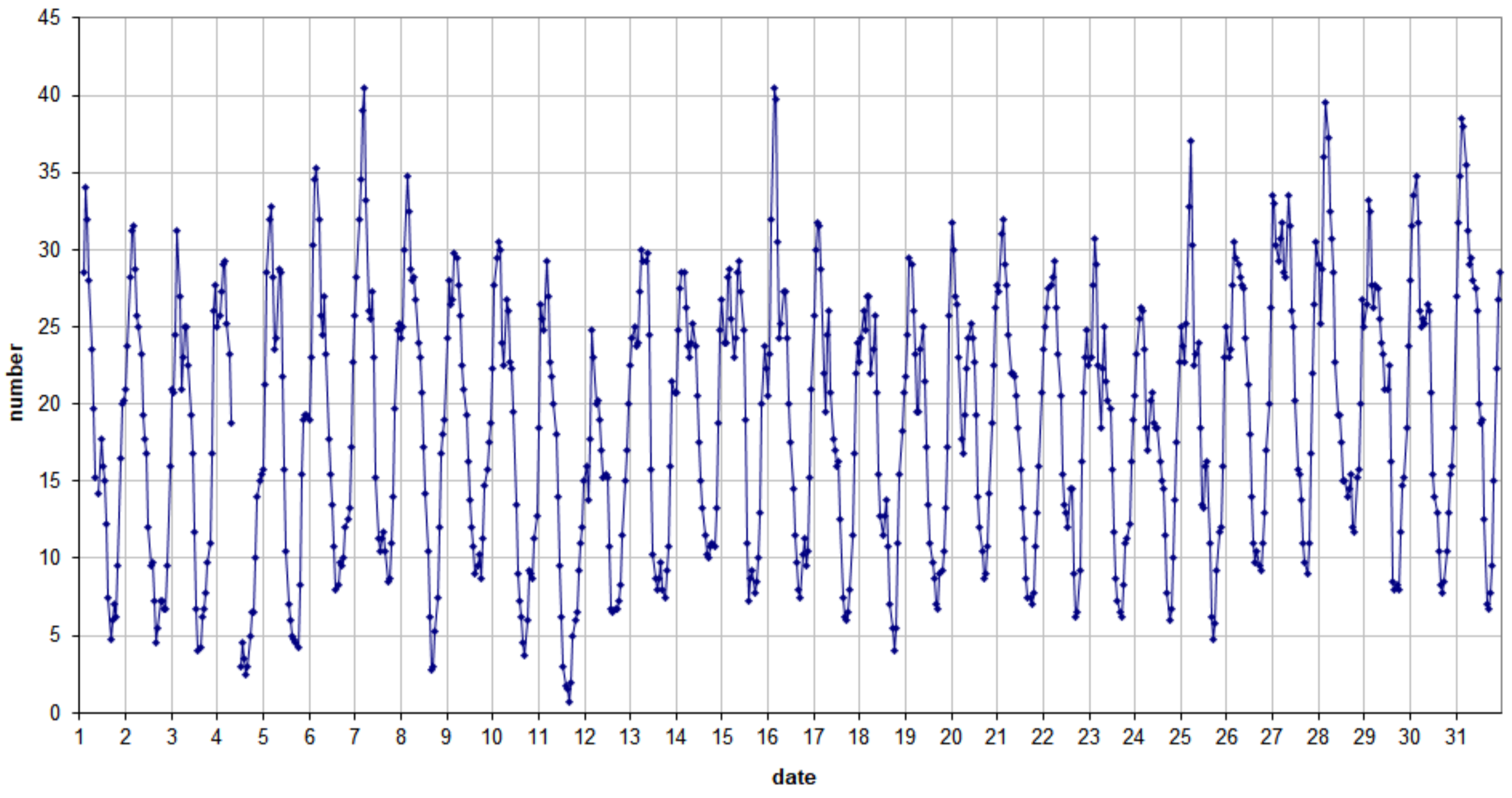
49.99 MHz - RadioMeteors March 2022 number of "all" reflections per hour (weighted average) (automatic count_Mette15_7Hz) Felix Verbelen (Kamphenhout)
