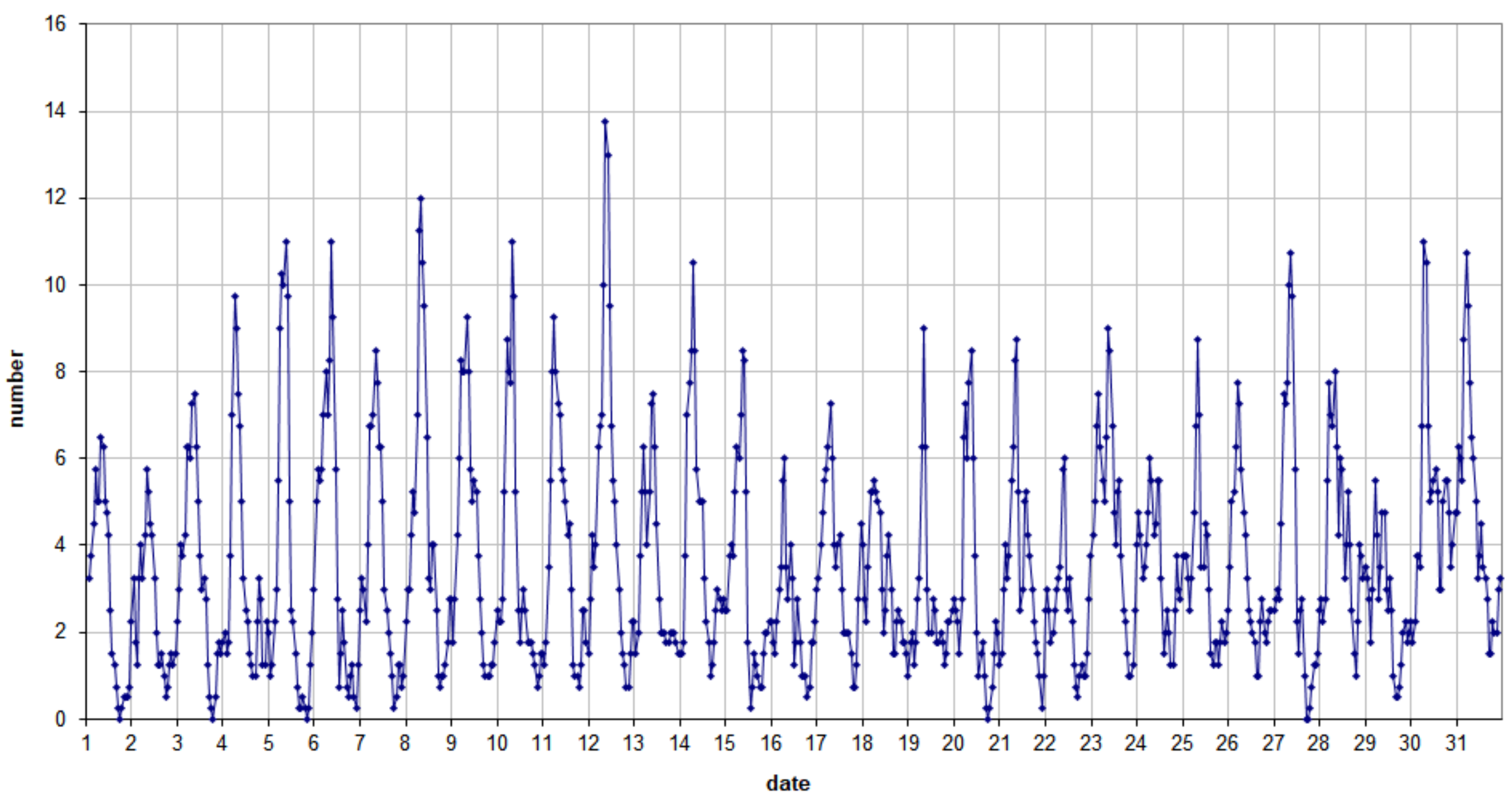
49.99MHz - RadioMeteors May 2022 number of overdense reflections per hour (weighted average) Felix Verbelen (Kamphenhout)
