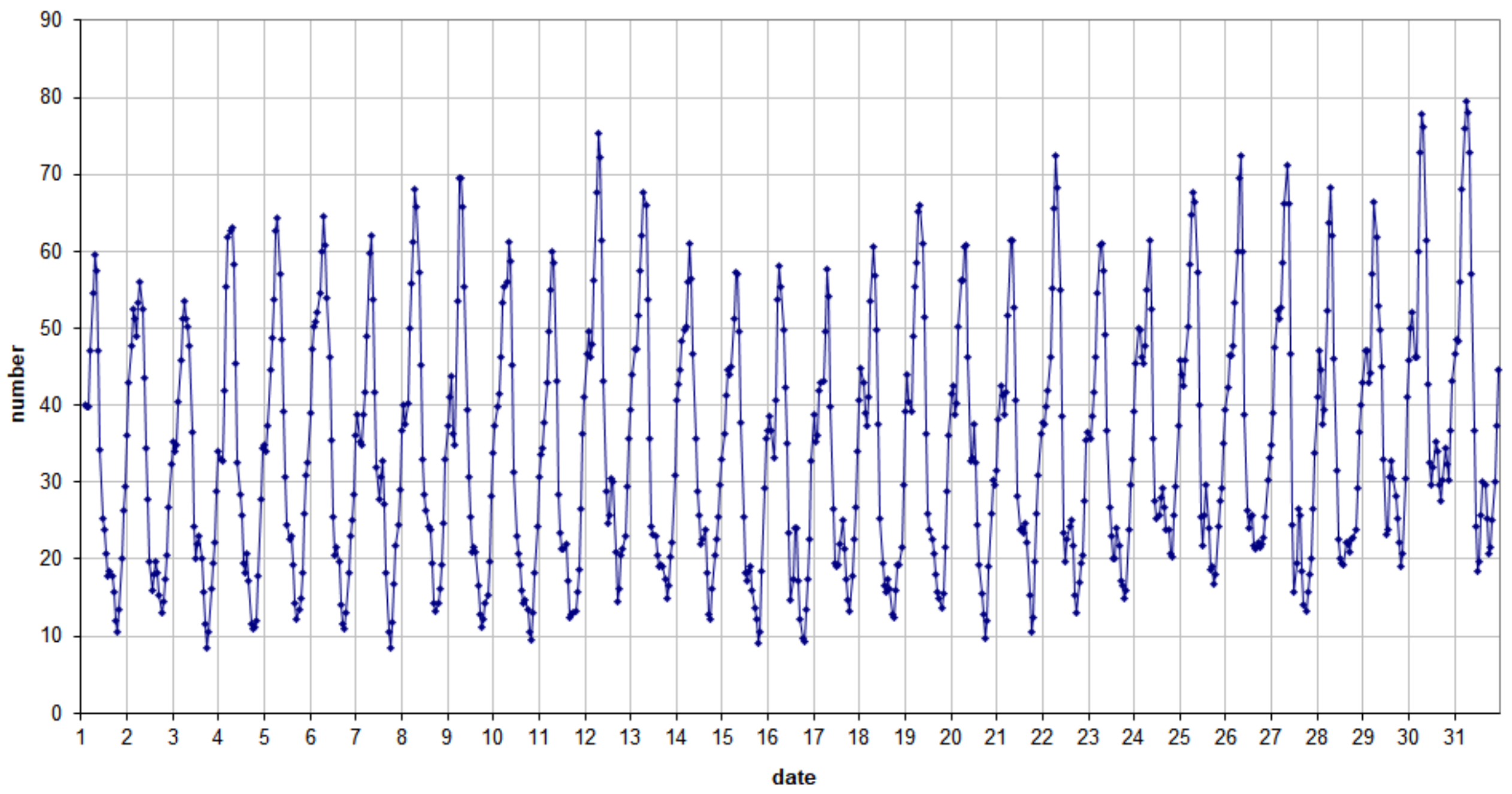
49.99 MHz - RadioMeteors May 2022 number of "all" reflections per hour (weighted average) (automatic count_Mette15_7Hz) Felix Verbelen (Kamphenhout)
