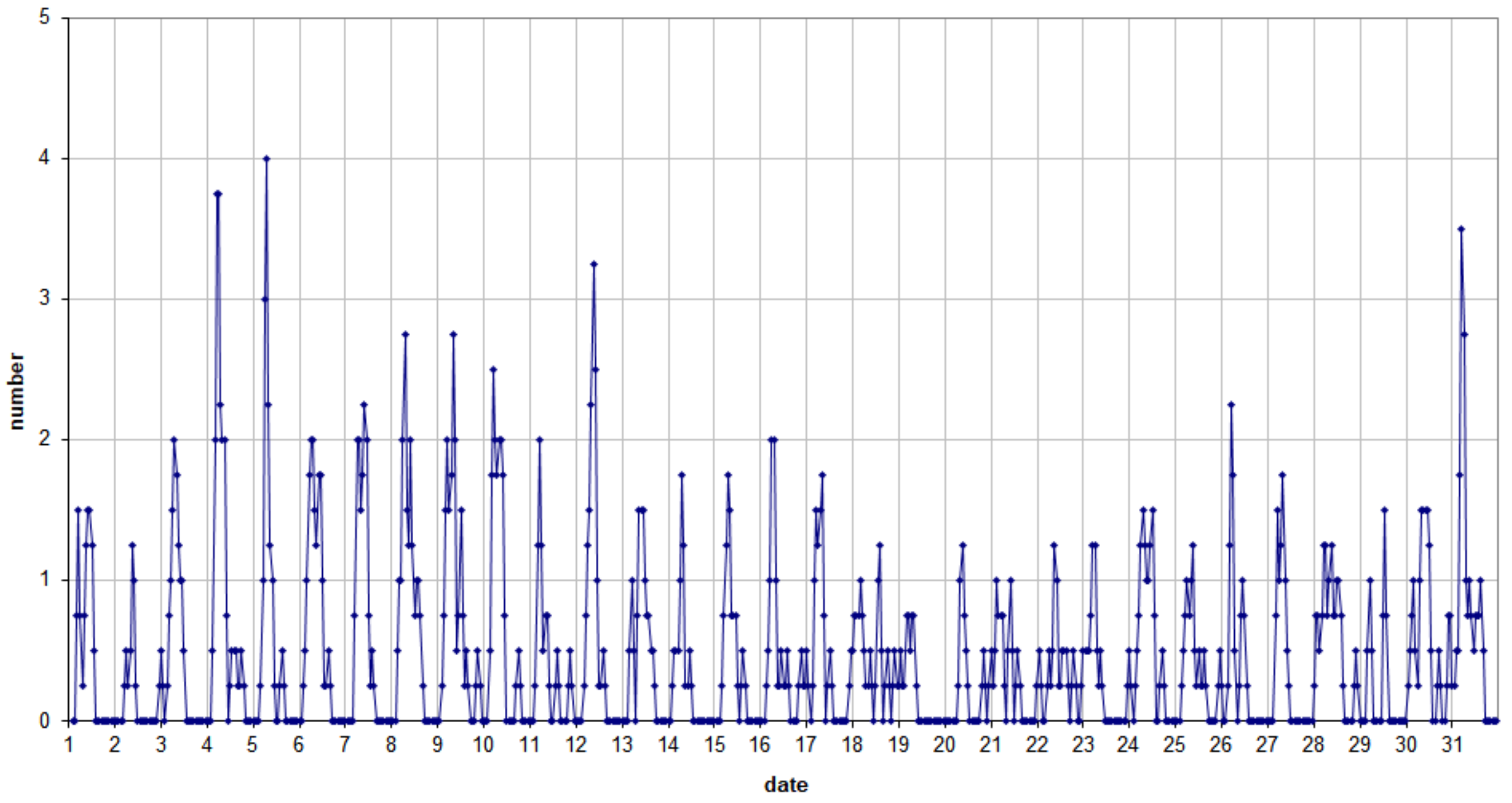
49.99MHz - RadioMeteors May 2022 number of reflections >10 seconds per hour (weighted average) Felix Verbelen (Kamphenhout)
