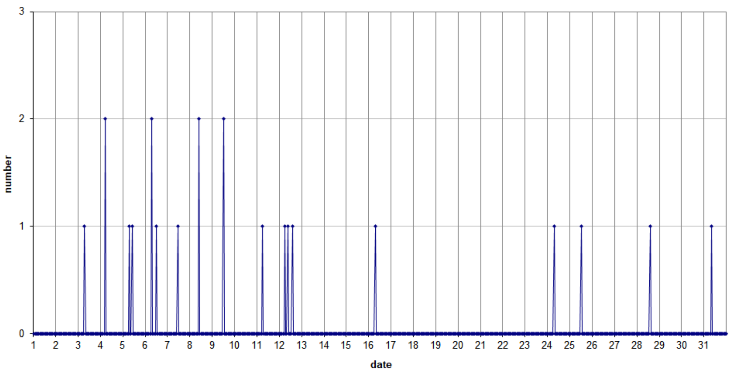
49.99MHz - RadioMeteors May 2022 hourly totals of overdense reflections longer than 1 minute Felix Verbelen (Kamphenhout/BE)
