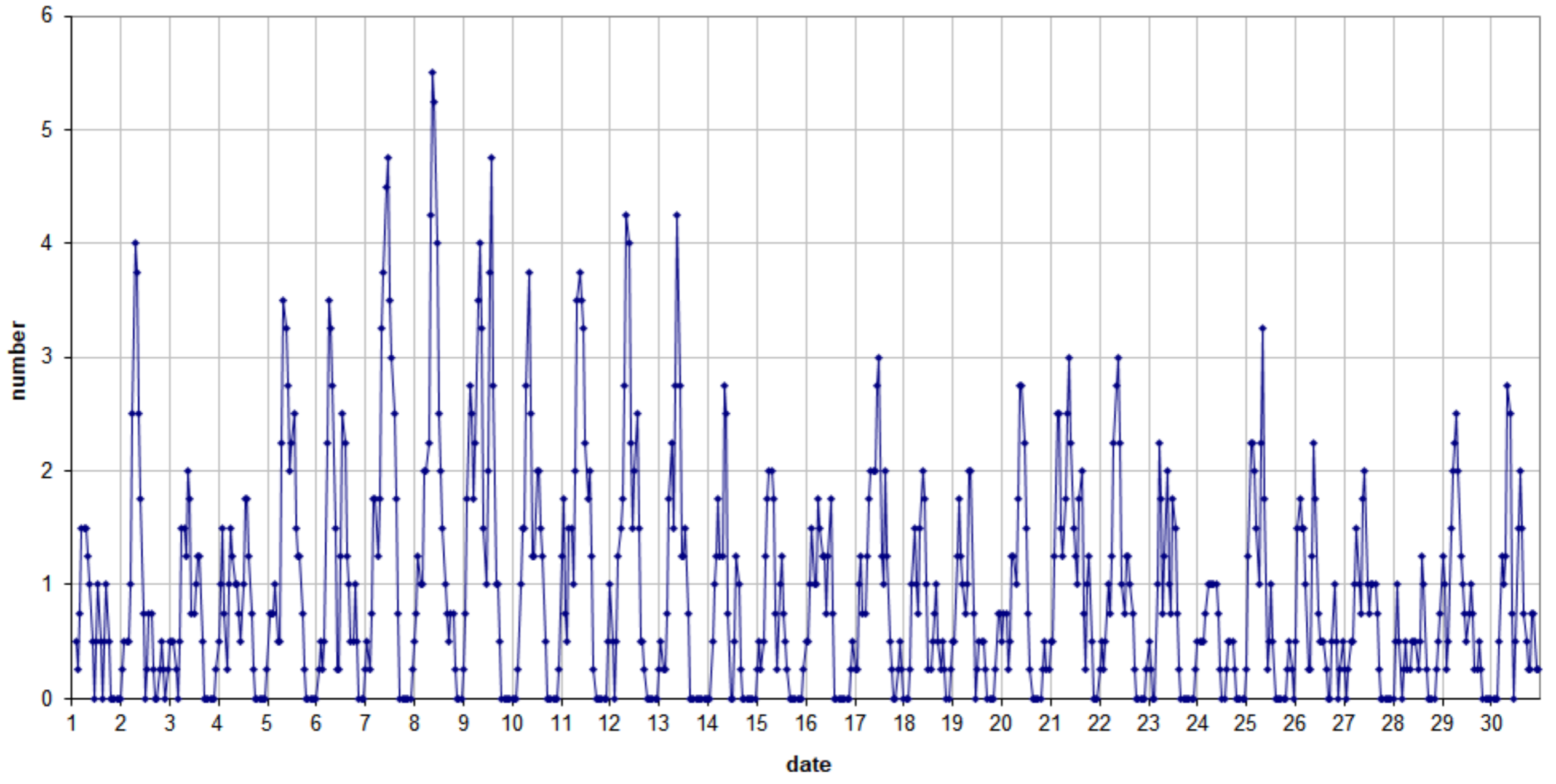
49.99MHz - RadioMeteors June 2022 number of reflections >10 seconds per hour (weighted average) Felix Verbelen (Kamphenhout)
