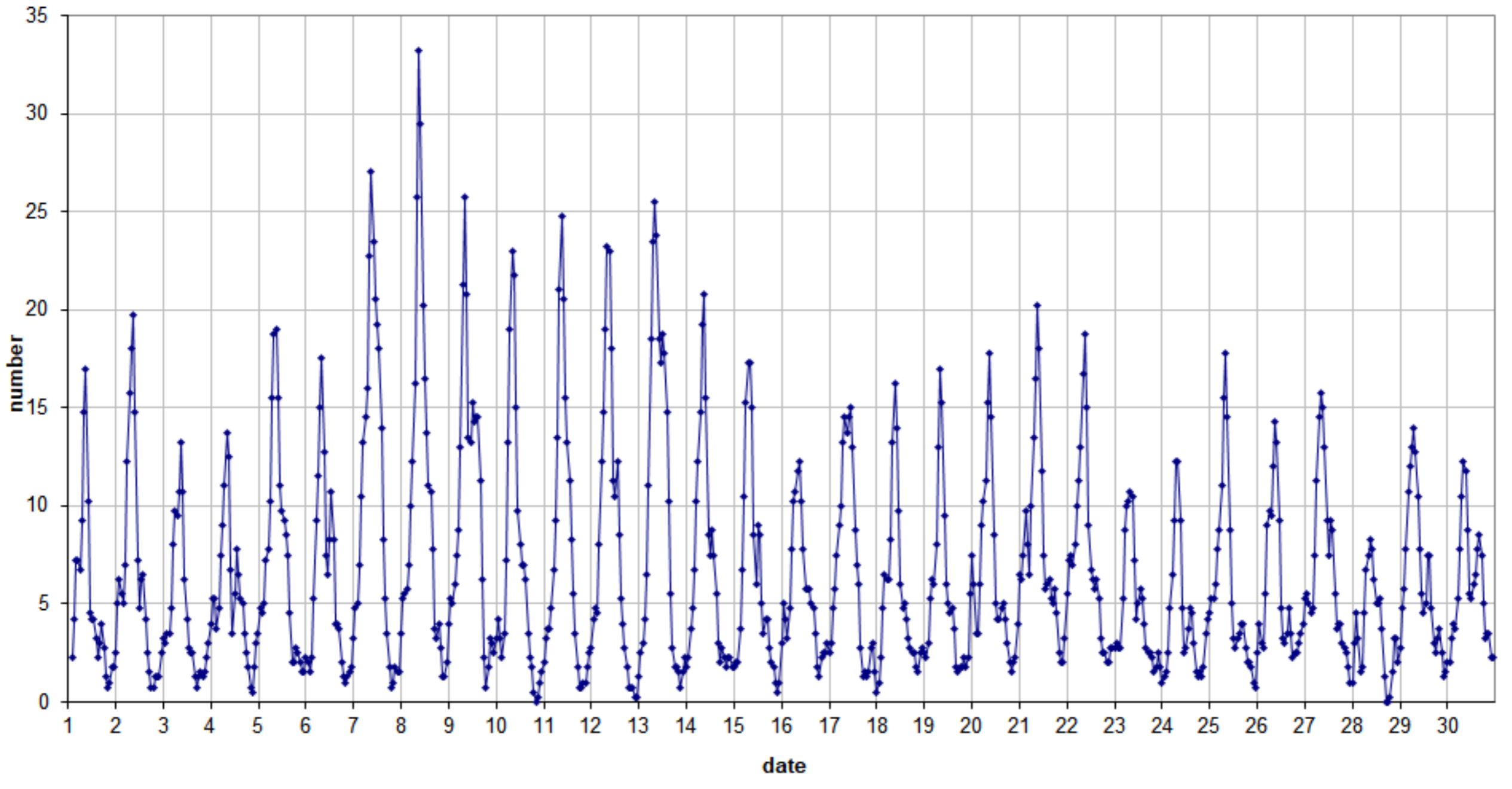
49.99MHz - RadioMeteors June 2022 number of overdense reflections per hour (weighted average) Felix Verbelen (Kamphenhout)
