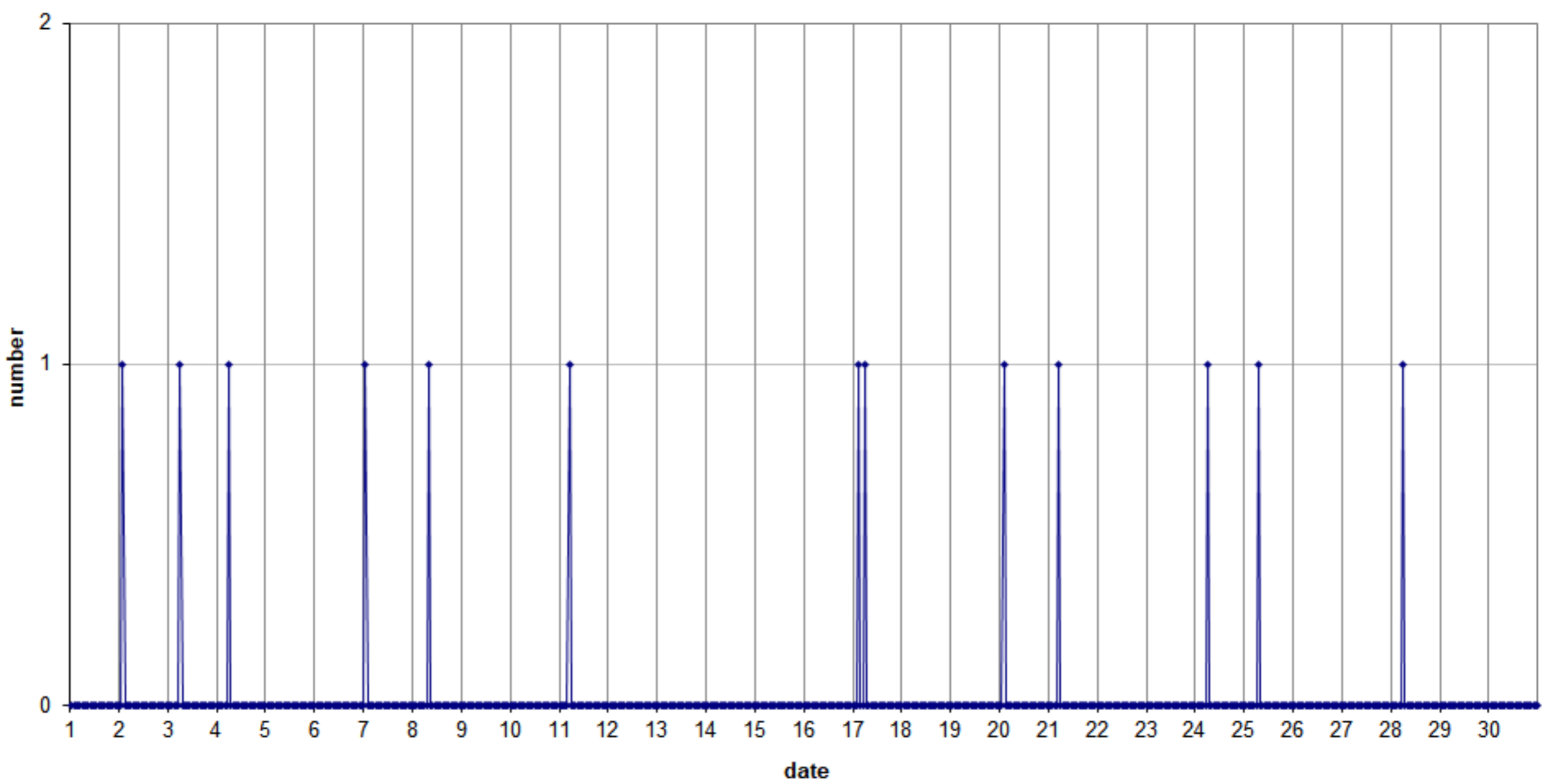
49.99MHz - RadioMeteors June 2022 hourly totals of overdense reflections longer than 1 minute Felix Verbelen (Kamphenhout/BE)
