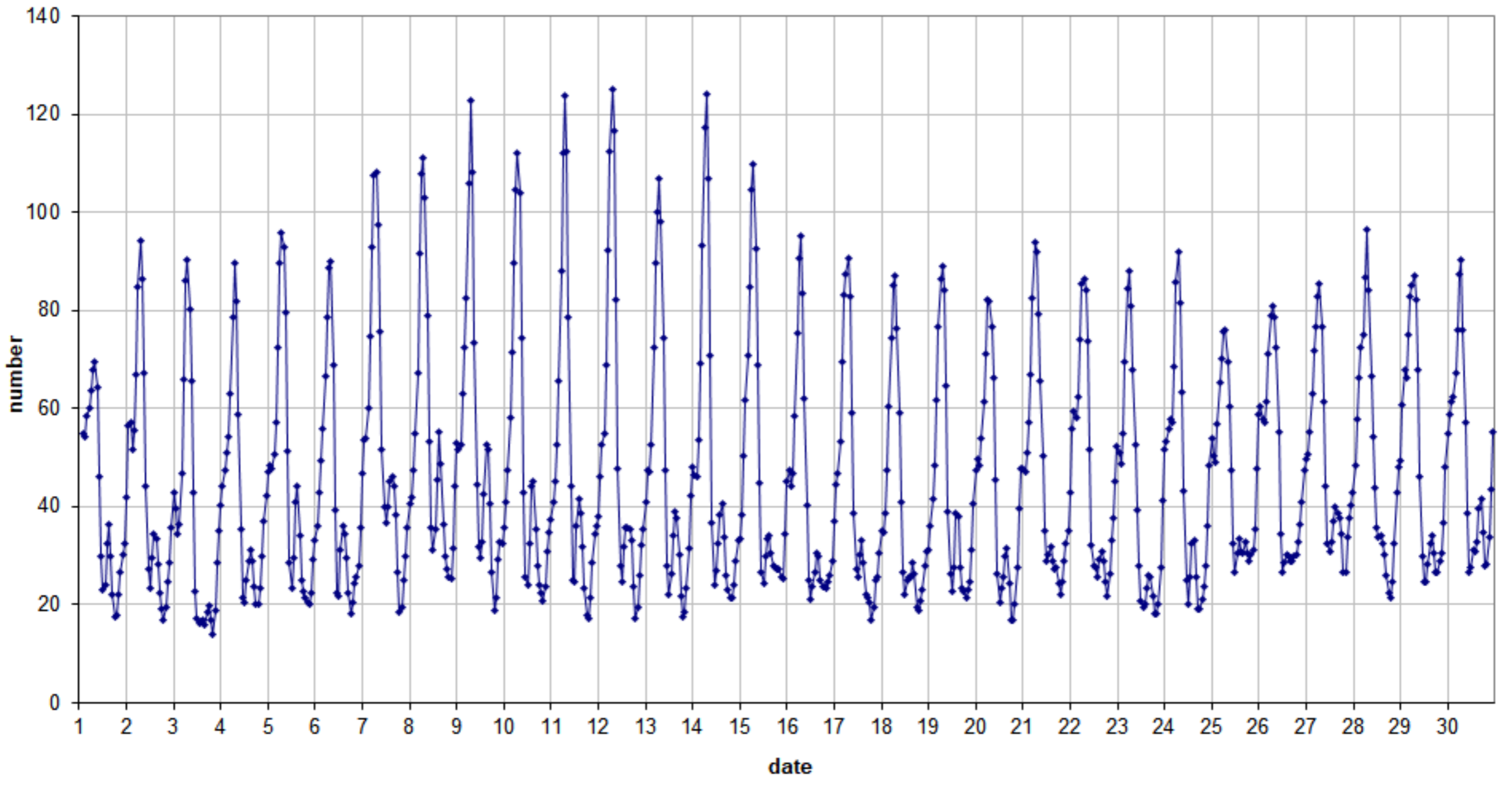
49.99 MHz - RadioMeteors June 2022 number of "all" reflections per hour (weighted average) (automatic count_Mettel5_7Hz) Felix Verbelen (Kamphenhout)
