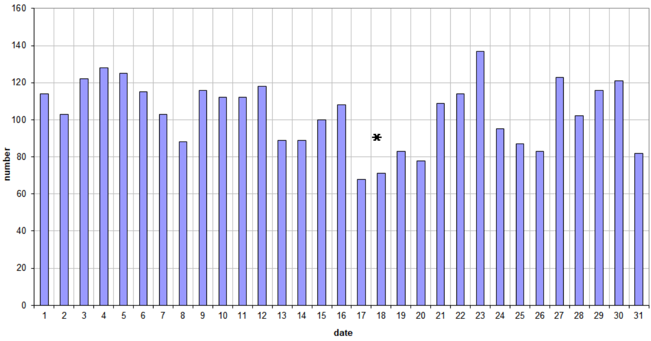
49.99MHz - RadioMeteors July 2022 daily totals of all overdense reflections Felix Verbelen (Kamphenhout)
