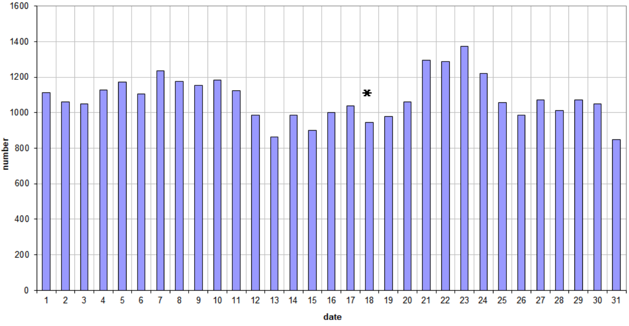
49.99MHz - RadioMeteors July 2022 daily totals of "all" reflections (automatic count_Mettel5_7Hz) Felix Verbelen (Kamphenhout)
