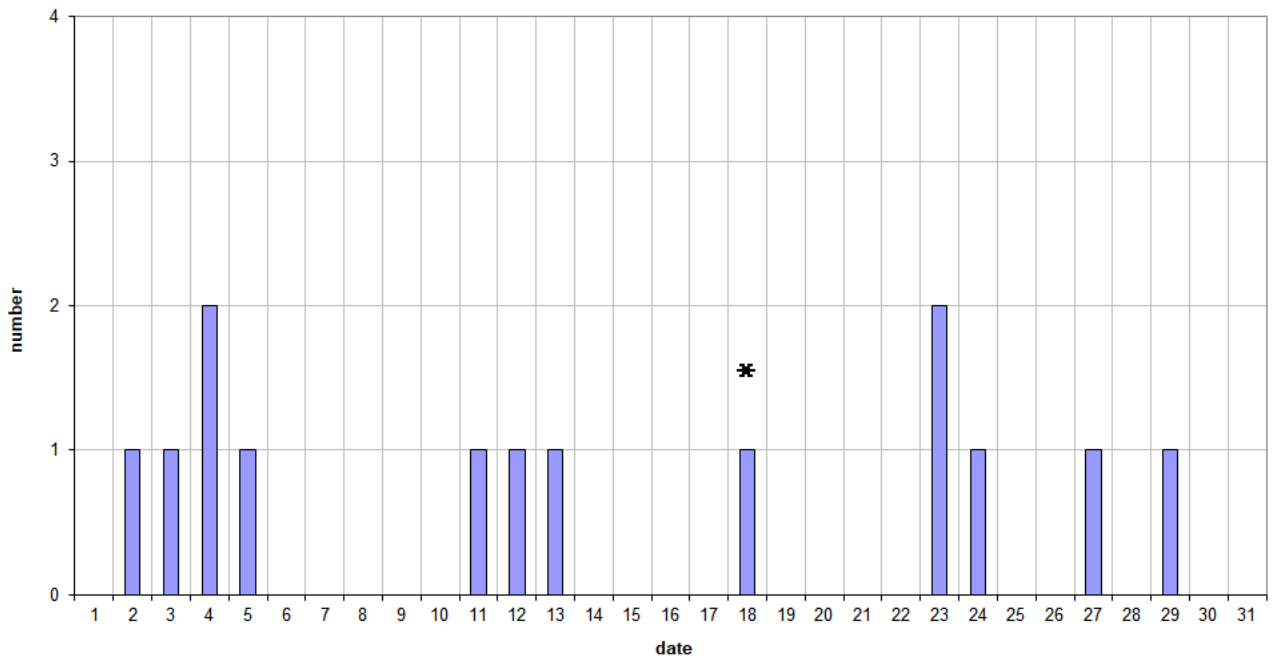
49.99MHz - RadioMeteors July 2022 daily totals of reflections longer than 1 minute Felix Verbelen (Kamphenhout)
