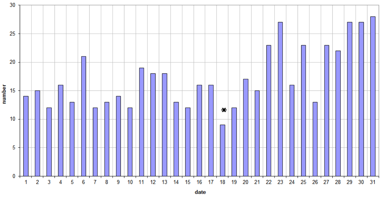
49.99MHz - RadioMeteors July 2022 daily totals of reflections longer than 10 seconds Felix Verbelen (Kamphenhout)
