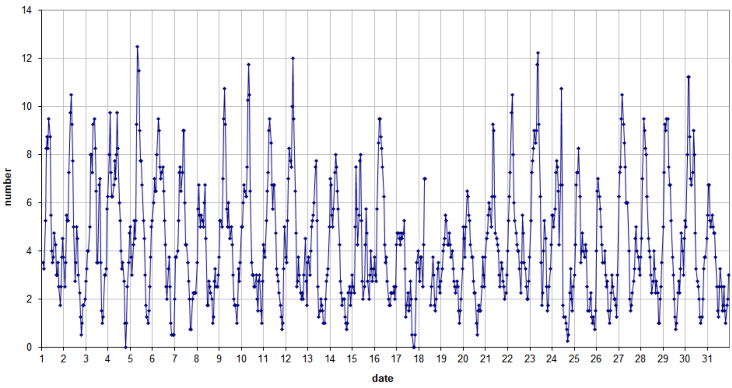
49.99MHz - RadioMeteors July 2022 number of overdense reflections per hour (weighted average) Felix Verbelen (Kamphenhout)
