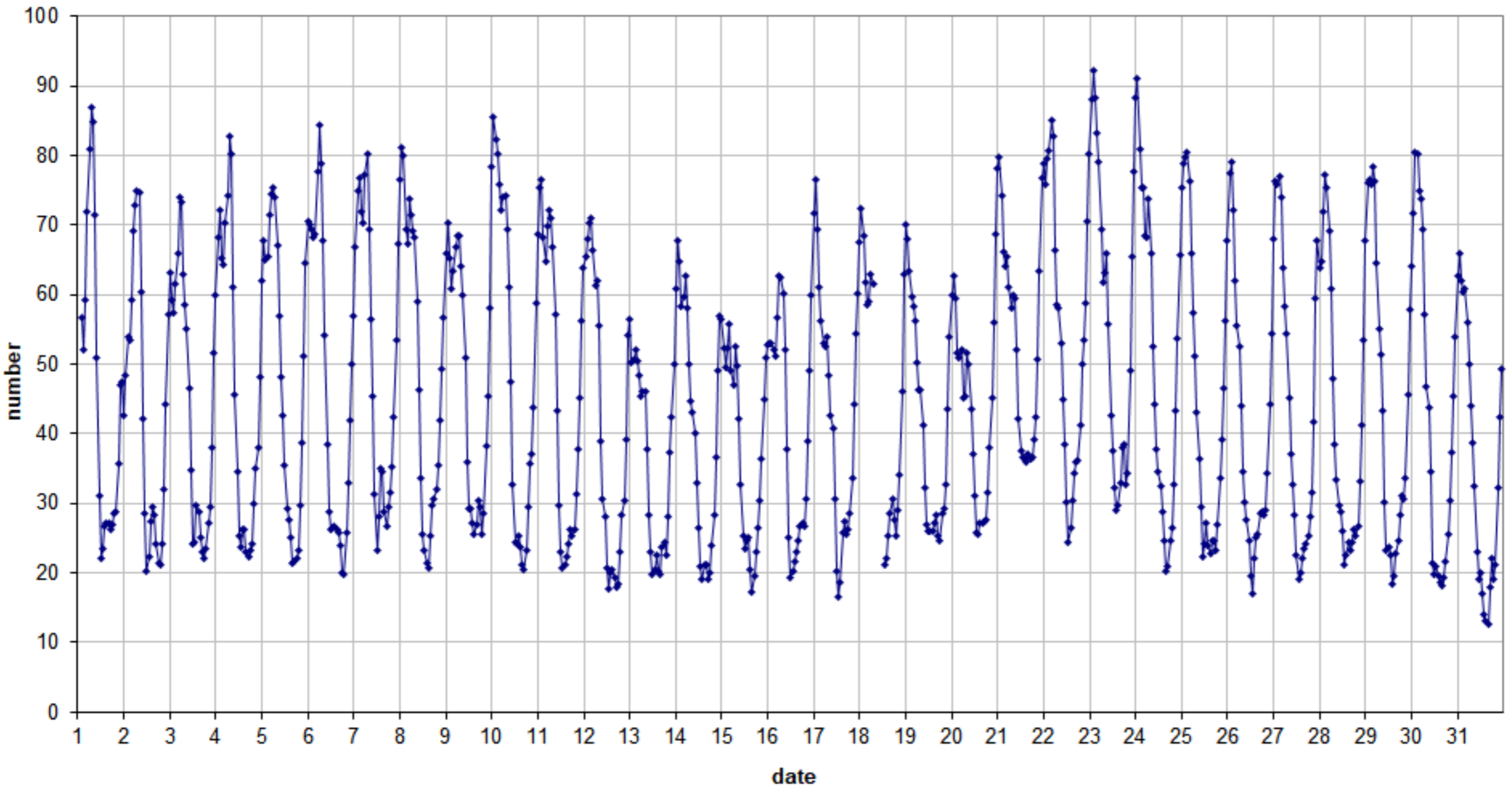
49.99 MHz - RadioMeteors July 2022 number of "all" reflections per hour (weighted average) (automatic count_Mette15_7Hz) Felix Verbelen (Kamphenhout)
