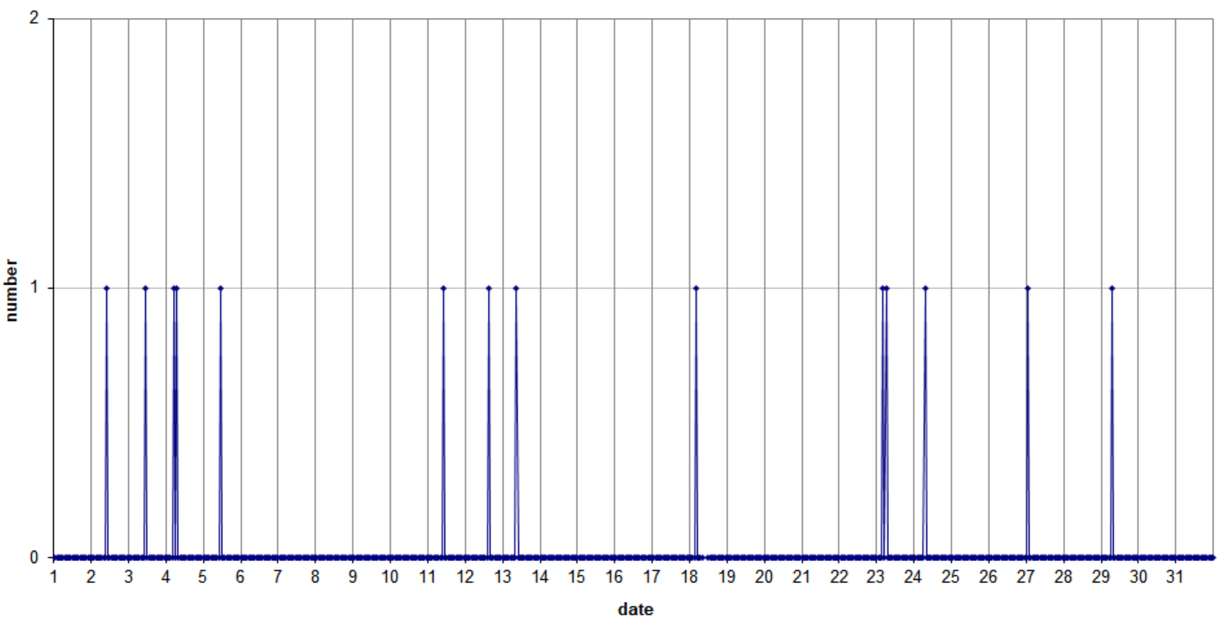
49.99MHz - RadioMeteors July 2022 hourly totals of overdense reflections longer than 1 minute Felix Verbelen (Kamphenhout/BE)
