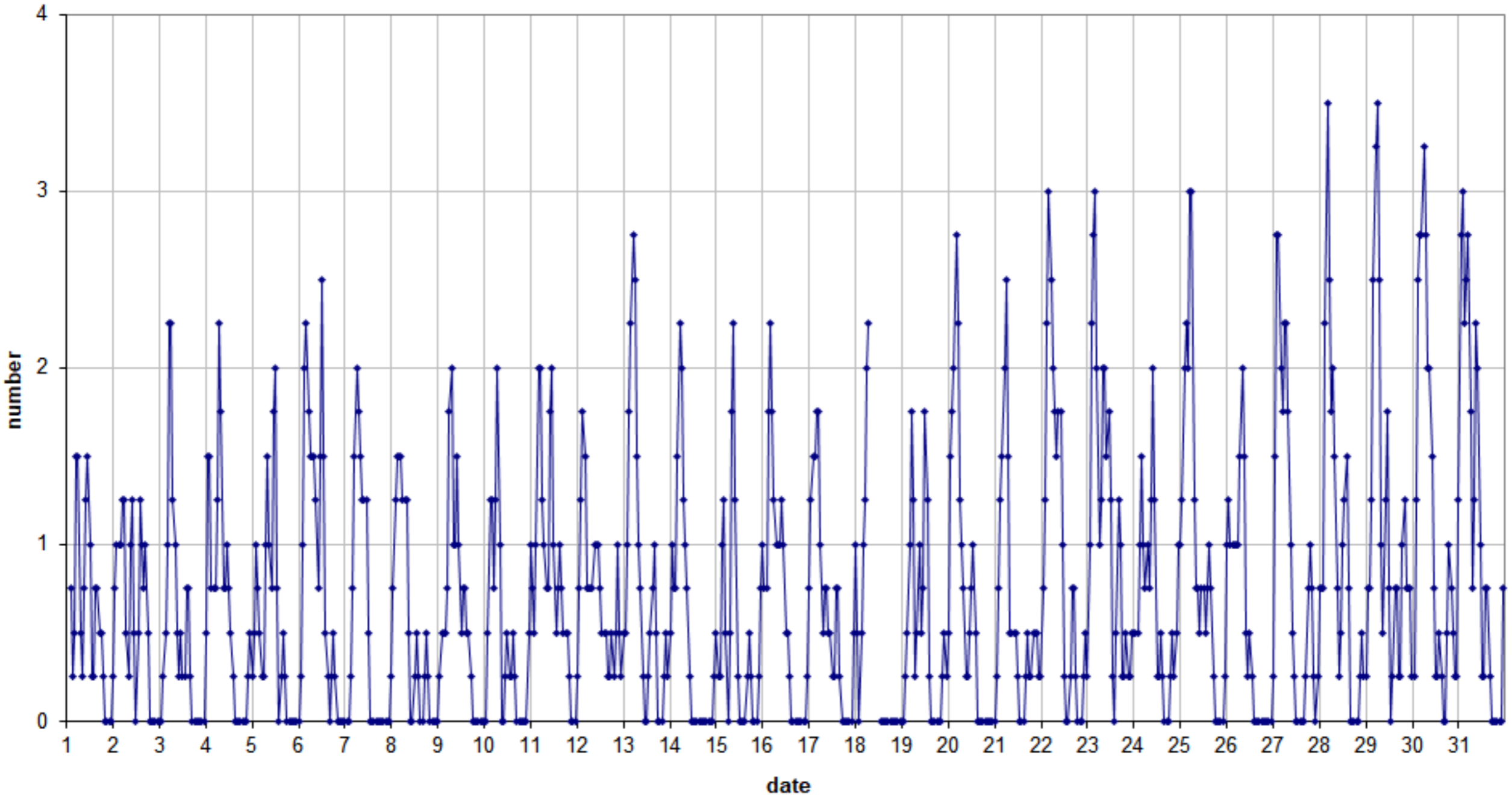
49.99MHz - RadioMeteors July 2022 number of reflections >10 seconds per hour (weighted average) Felix Verbelen (Kamphenhout)
