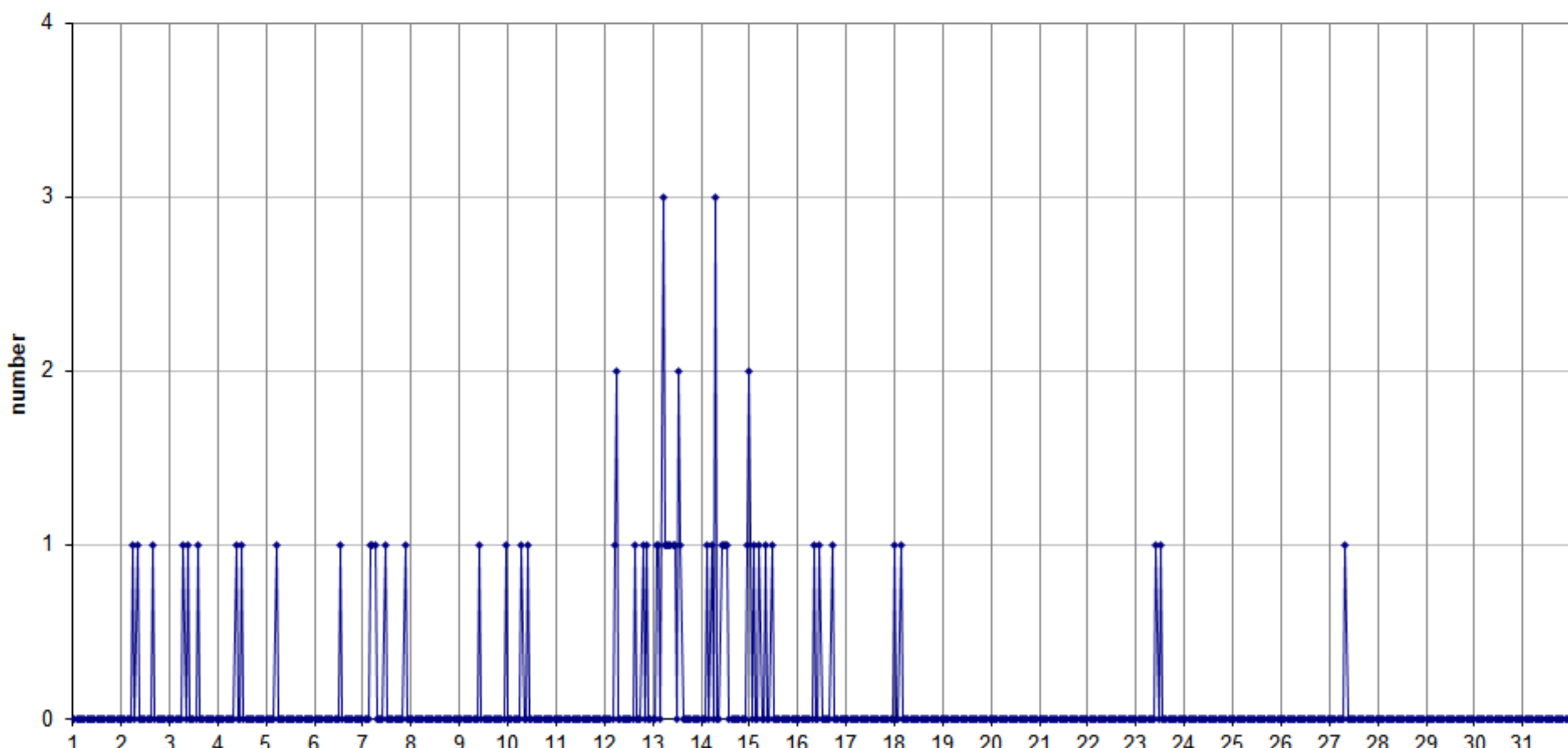
49.99MHz - RadioMeteors August 2022 hourly totals of overdense reflections longer than 1 minute Felix Verbelen (Kampenhout/BE)
