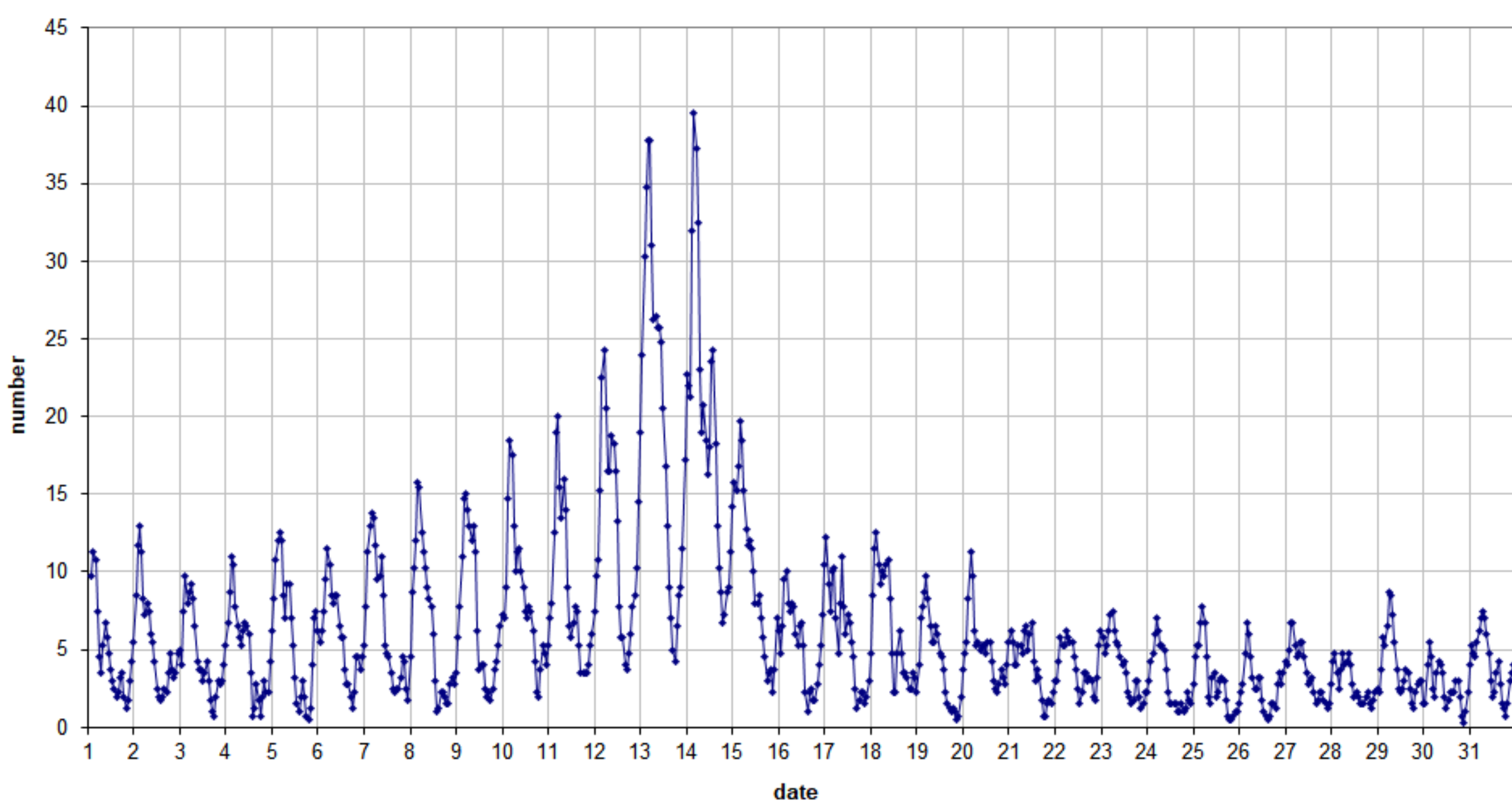
49.99MHz - RadioMeteors August 2022 number of overdense reflections per hour (weighted average) Felix Verbelen (Kampenhout)
