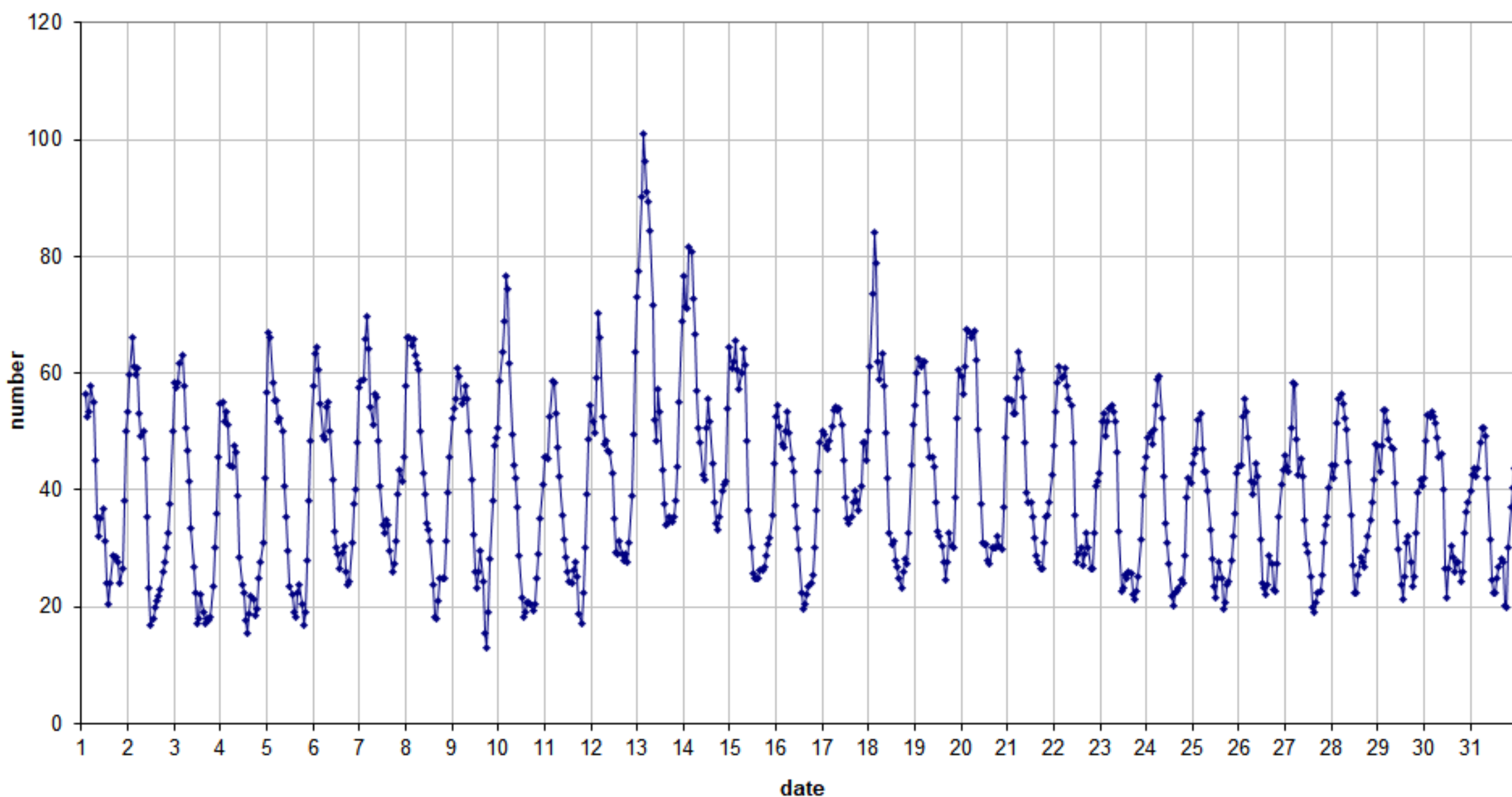
49.99 MHz - RadioMeteors August 2022 number of "all" reflections per hour (weighted average) (automatic count_Mettel5_7Hz) Felix Verbelen (Kampenhout)
