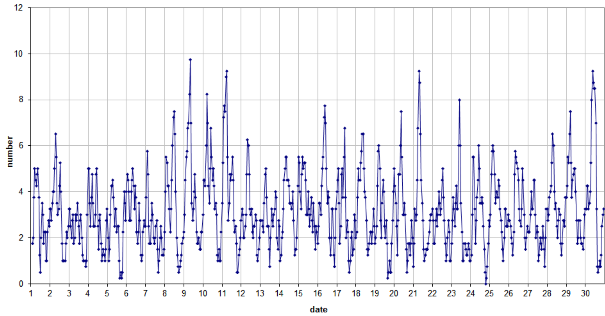
49.99MHz - RadioMeteors September 2022 number of overdense reflections per hour (weighted average) Felix Verbelen (Kamphenhout)
