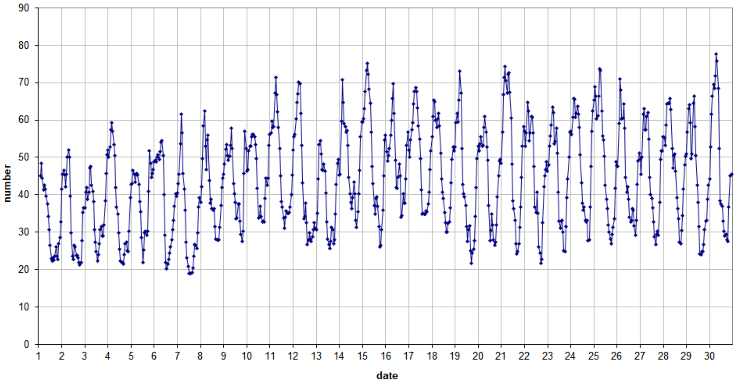
49.99 MHz - RadioMeteors September 2022 number of "all" reflections per hour (weighted average) (automatic count_Mette15_7Hz) Felix Verbelen (Kamphenhout)
