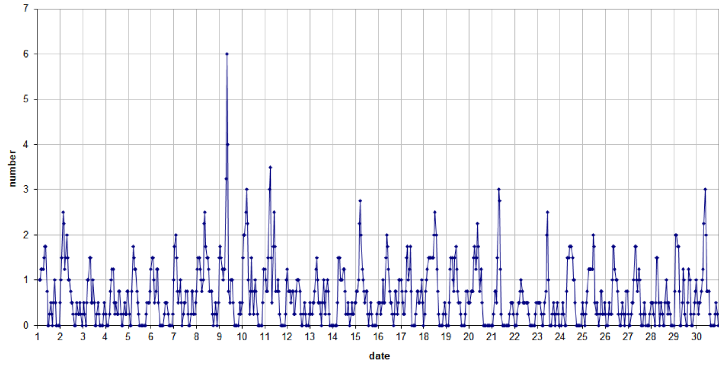
49.99MHz - RadioMeteors September 2022 number of reflections >10 seconds per hour (weighted average) Felix Verbelen (Kamphenhout)
