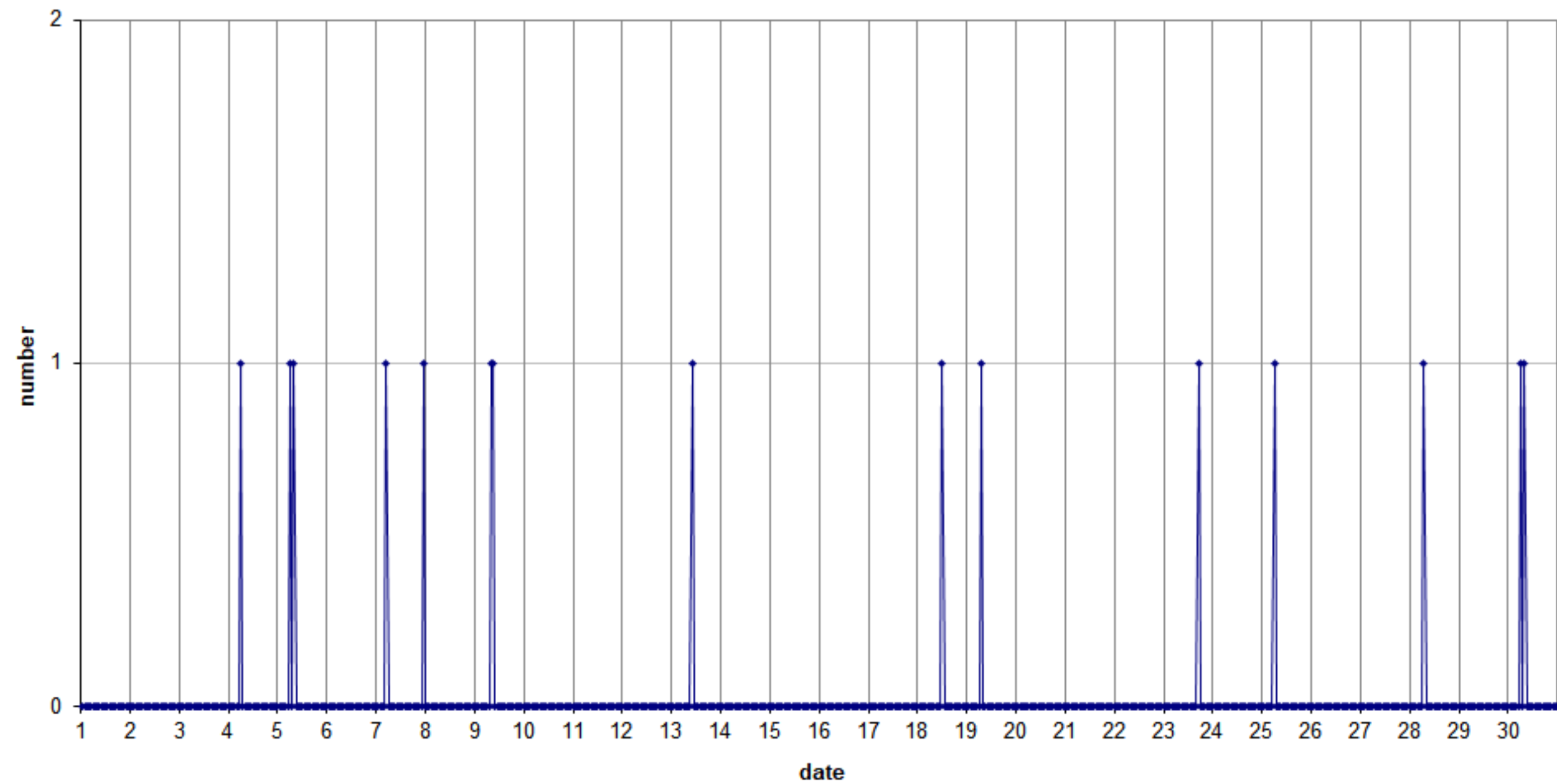
49.99MHz - RadioMeteors September 2022 hourly totals of overdense reflections longer than 1 minute Felix Verbelen (Kamphenhout/BE)
