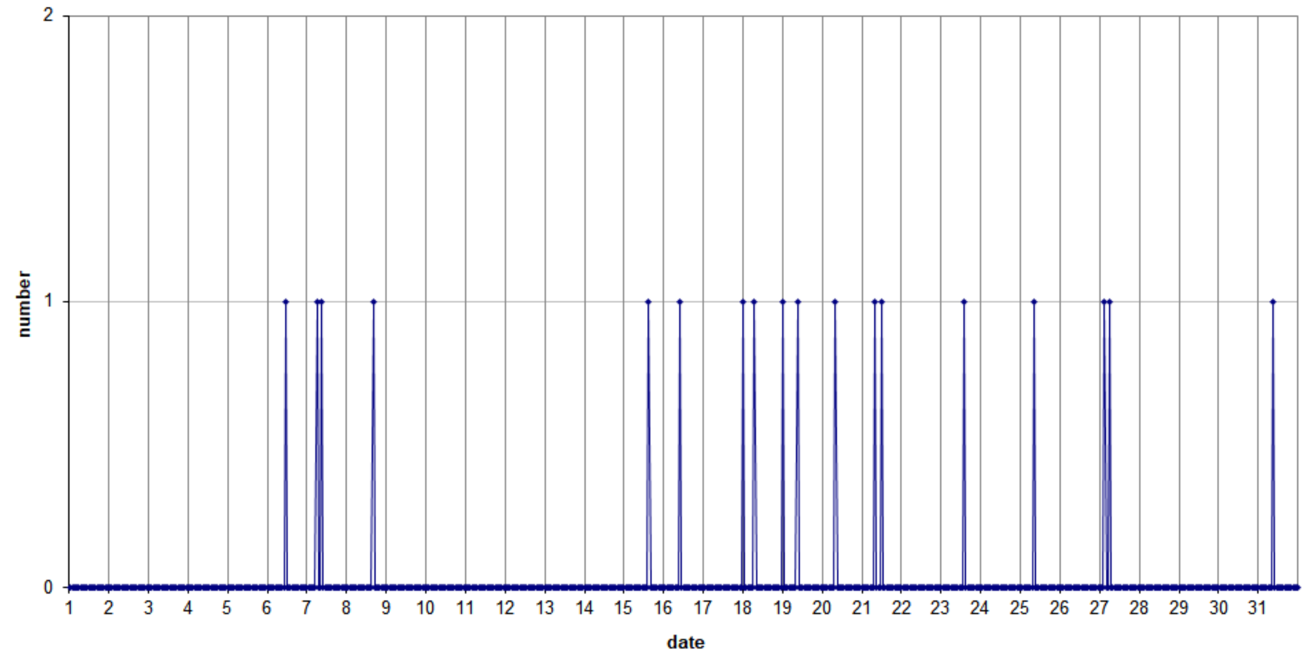
49.99MHz - RadioMeteors October 2022 hourly totals of overdense reflections longer than 1 minute Felix Verbelen (Kampenhout/BE)
