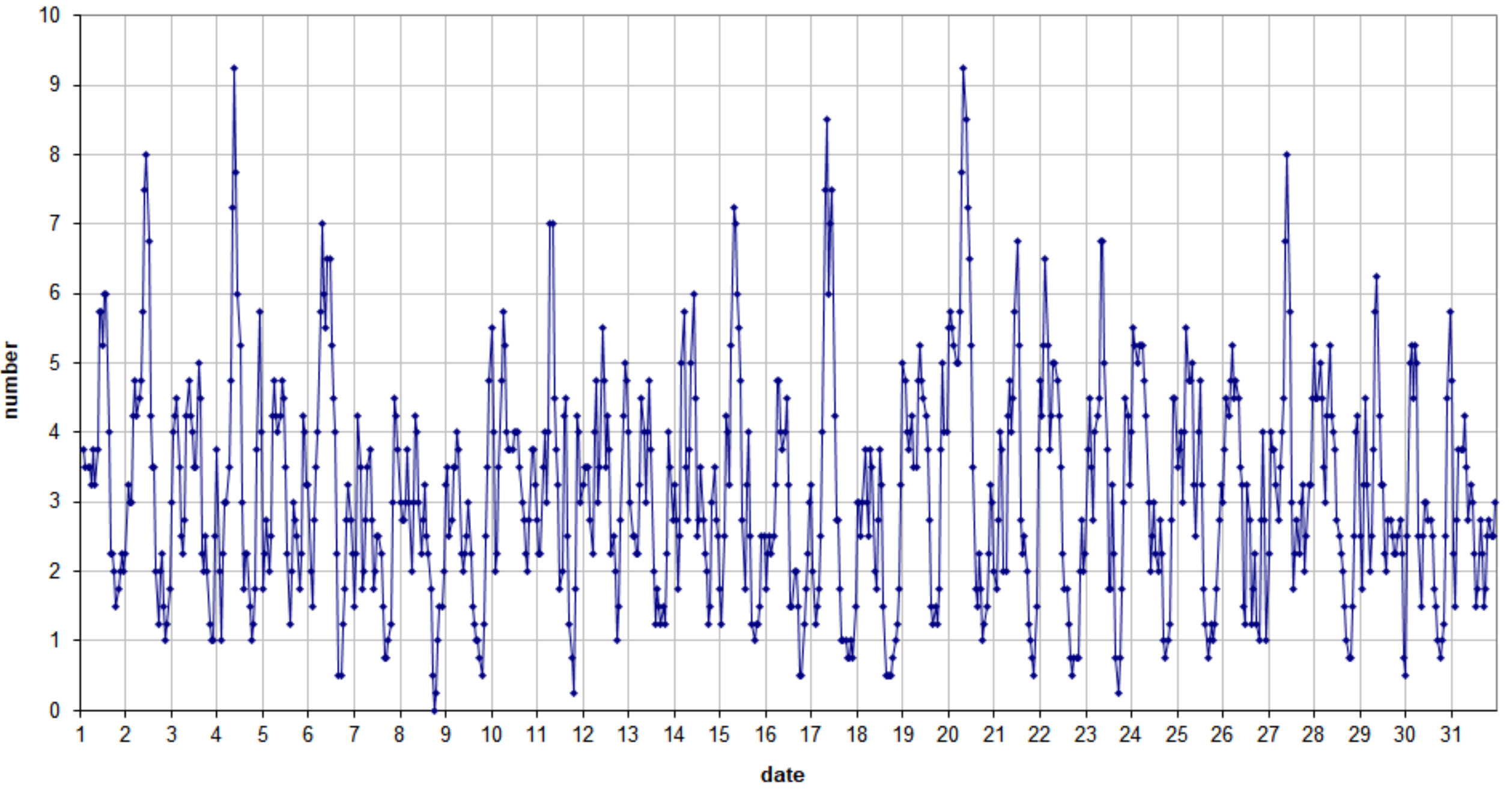
49.99MHz - RadioMeteors October 2022 number of overdense reflections per hour (weighted average) Felix Verbelen (Kampenhout)
