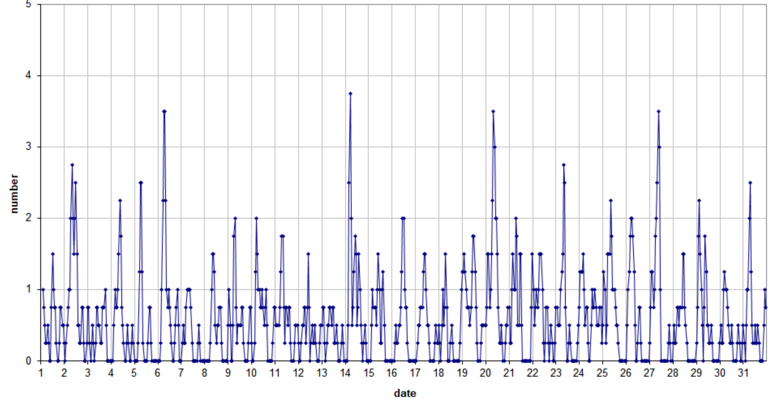
49.99MHz - RadioMeteors October 2022 number of reflections >10 seconds per hour (weighted average) Felix Verbelen (Kampenhout)
