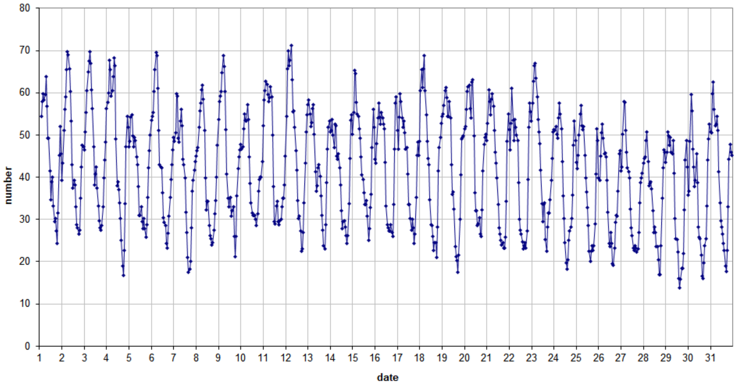
49.99 MHz - RadioMeteors October 2022 number of "all" reflections per hour (weighted average) (automatic count_Mette15_7Hz) Felix Verbelen (Kampenhout)
