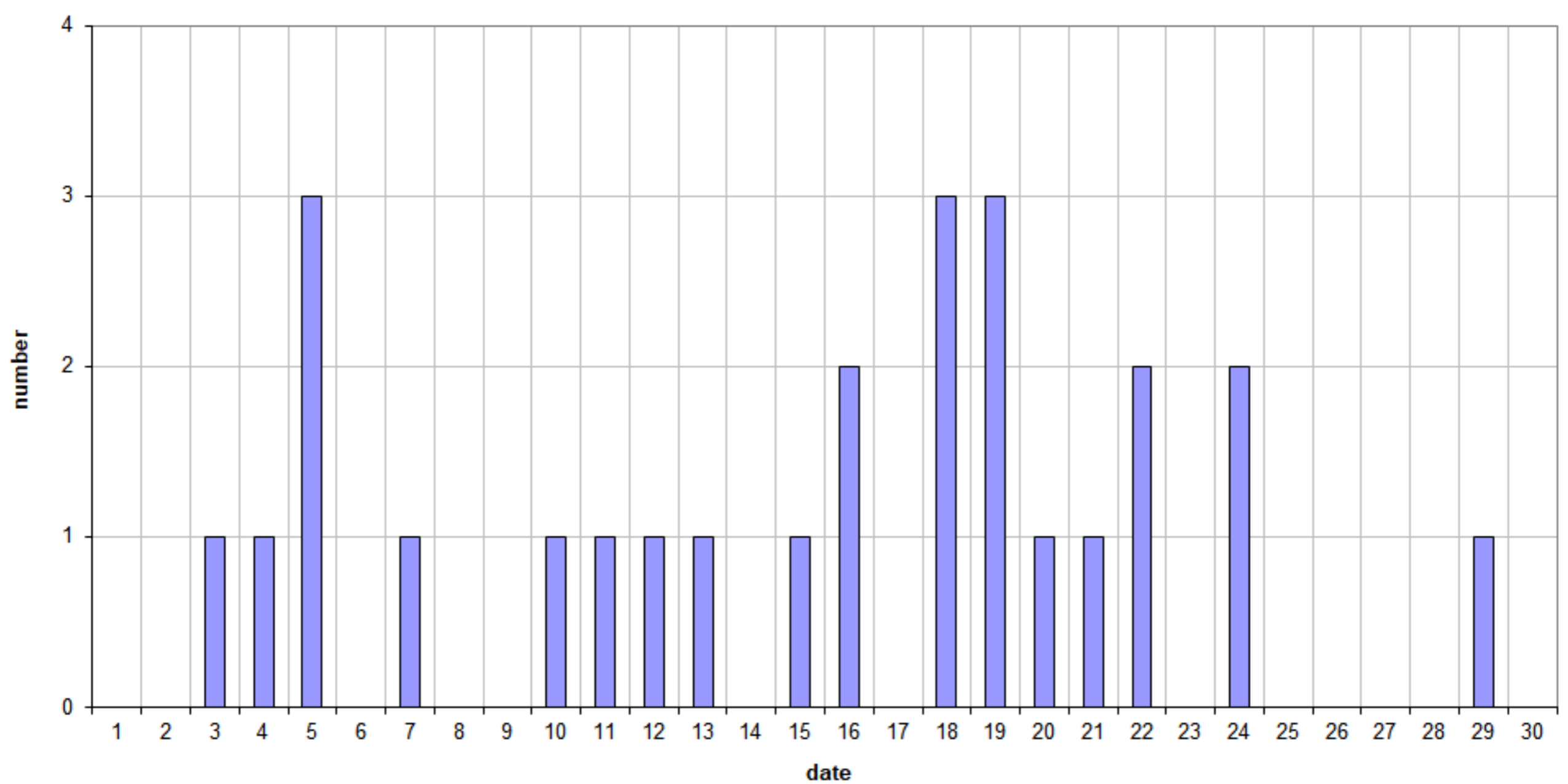
49.99MHz - RadioMeteors November 2022 daily totals of reflections longer than 1 minute Felix Verbelen (Kampenhout)
