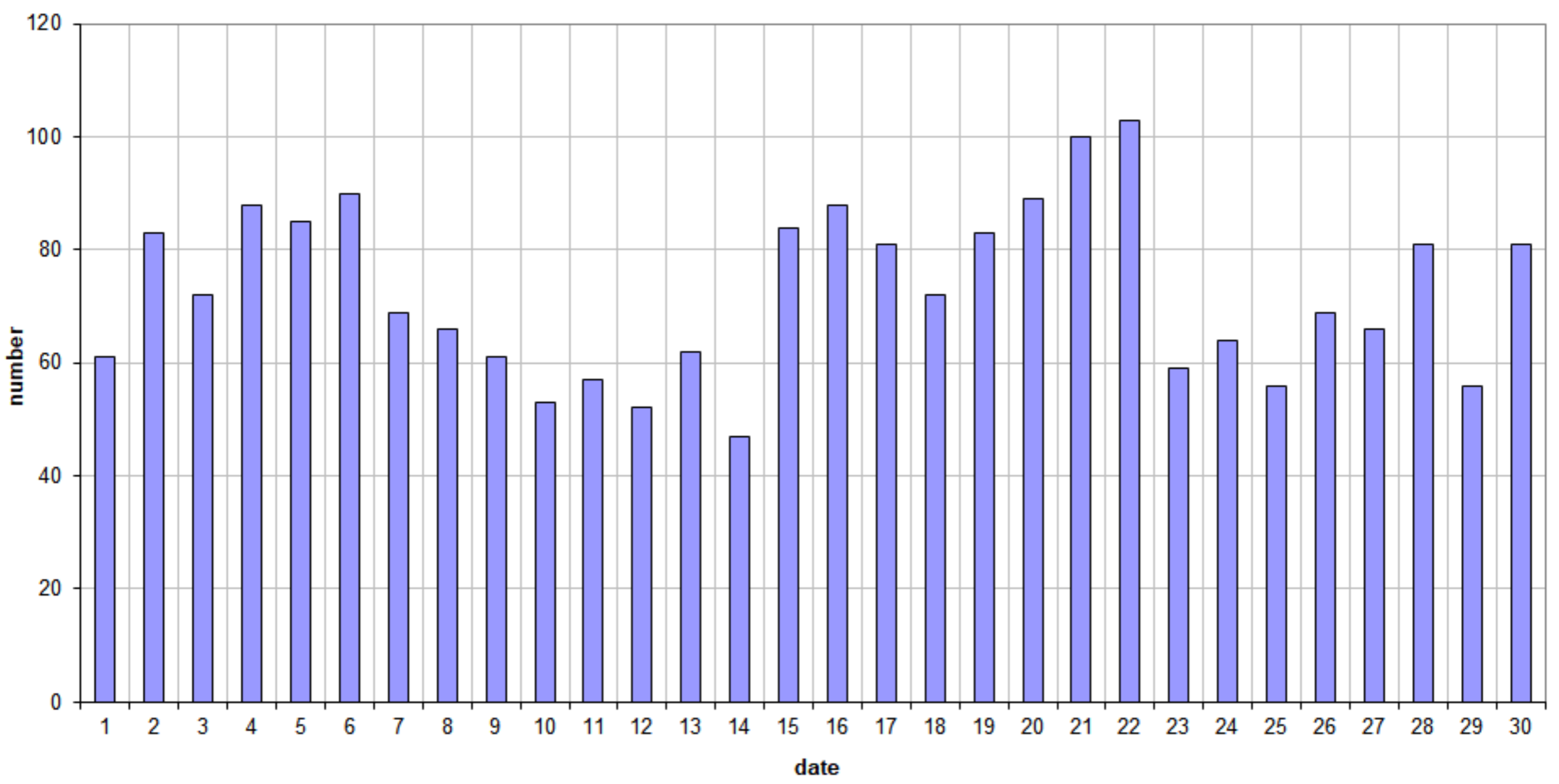
49.99MHz - RadioMeteors November 2022 daily totals of all overdense reflections Felix Verbelen (Kampenhout)
