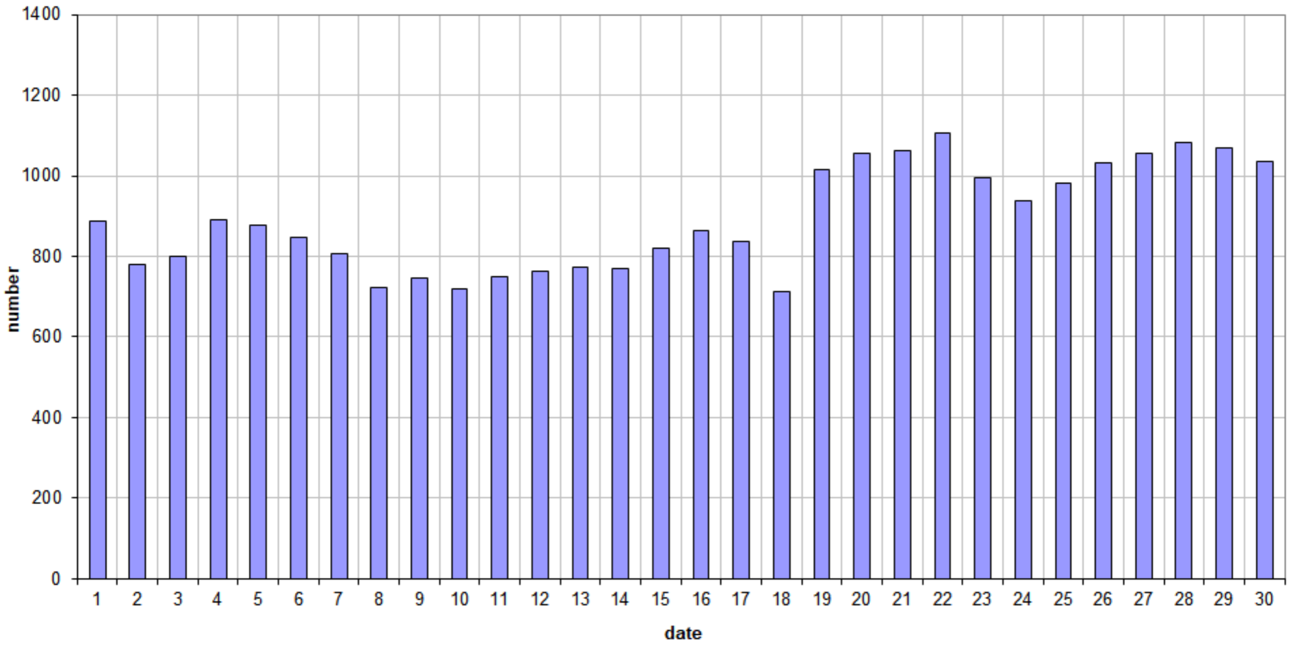
49.99MHz - RadioMeteors November 2022 daily totals of "all" reflections (automatic count_Mettel5_7Hz) Felix Verbelen (Kampenhout)
