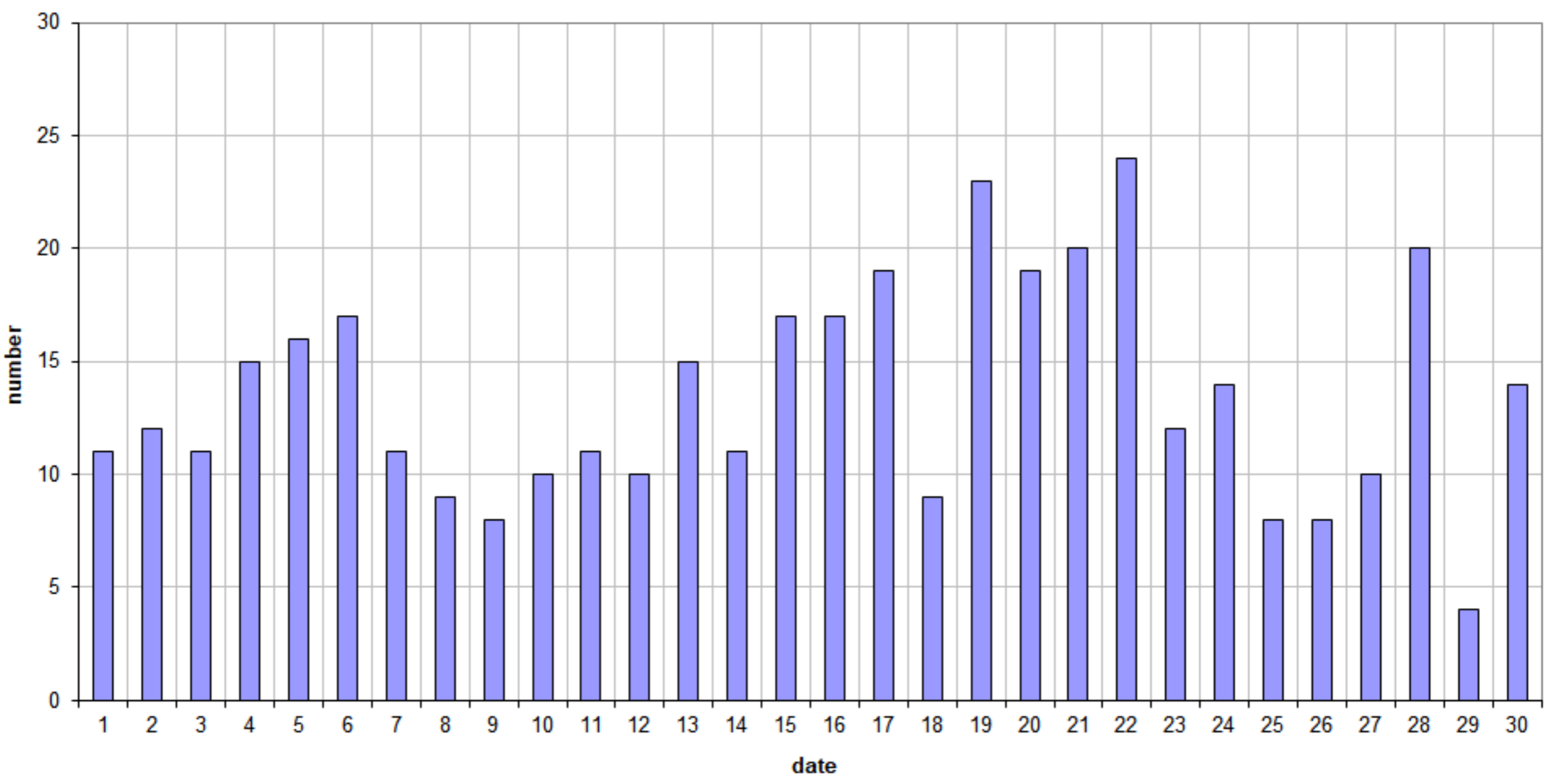
49.99MHz - RadioMeteors November 2022 daily totals of reflections longer than 10 seconds Felix Verbelen (Kampenhout)
