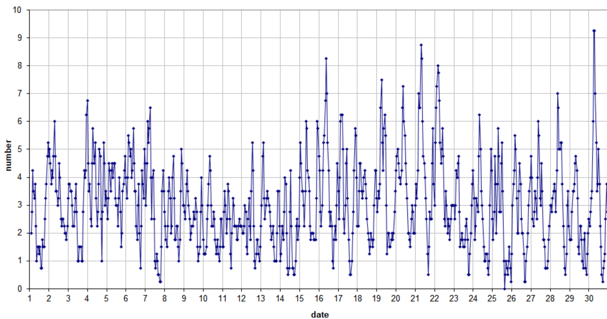
49.99MHz - RadioMeteors November 2022 number of overdense reflections per hour (weighted average) Felix Verbelen (Kamphenhout)
