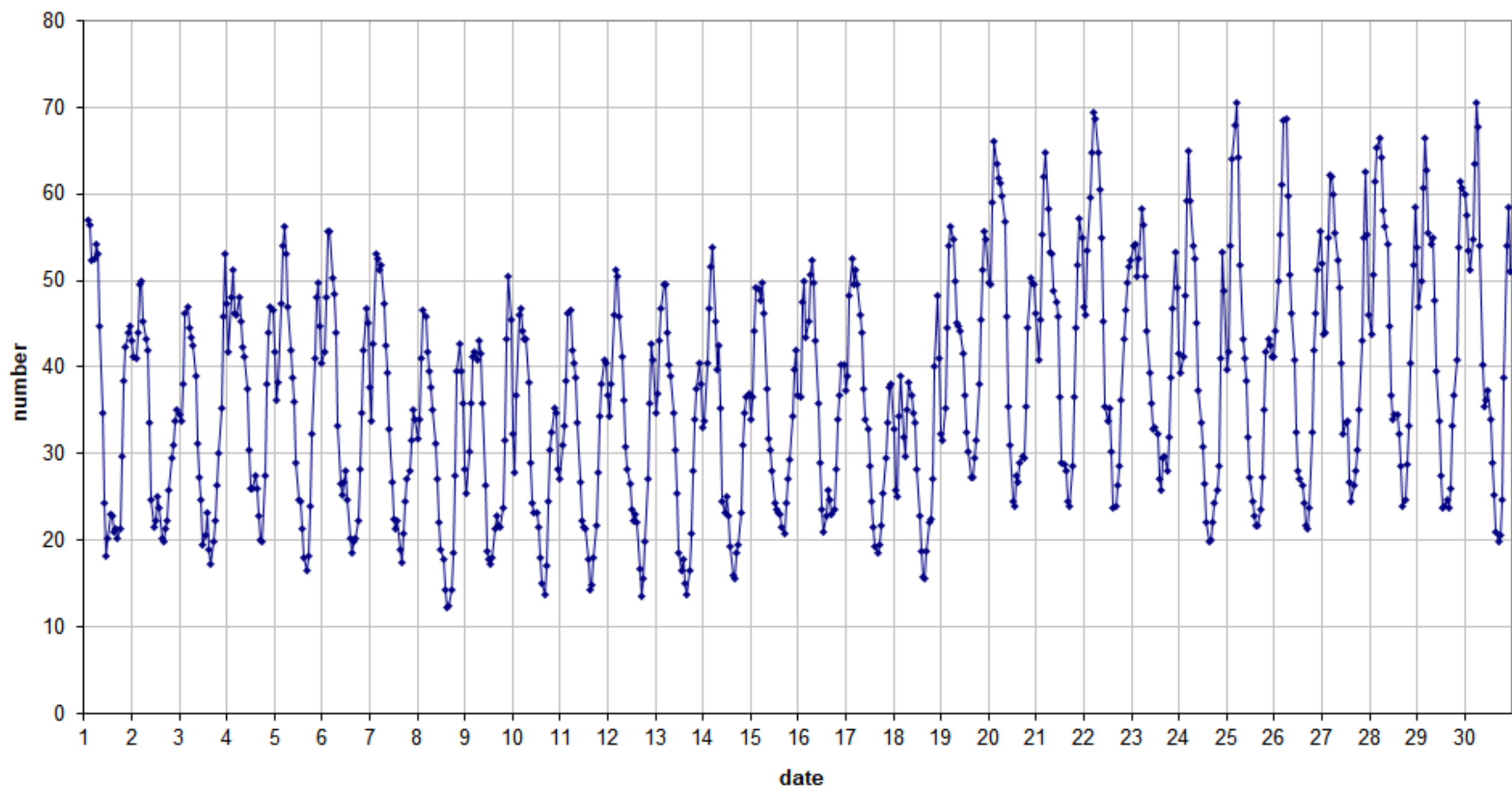
49.99 MHz - RadioMeteors November 2022 number of "all" reflections per hour (weighted average) (automatic count_Mettel5_7Hz) Felix Verbelen (Kamphenhout)
