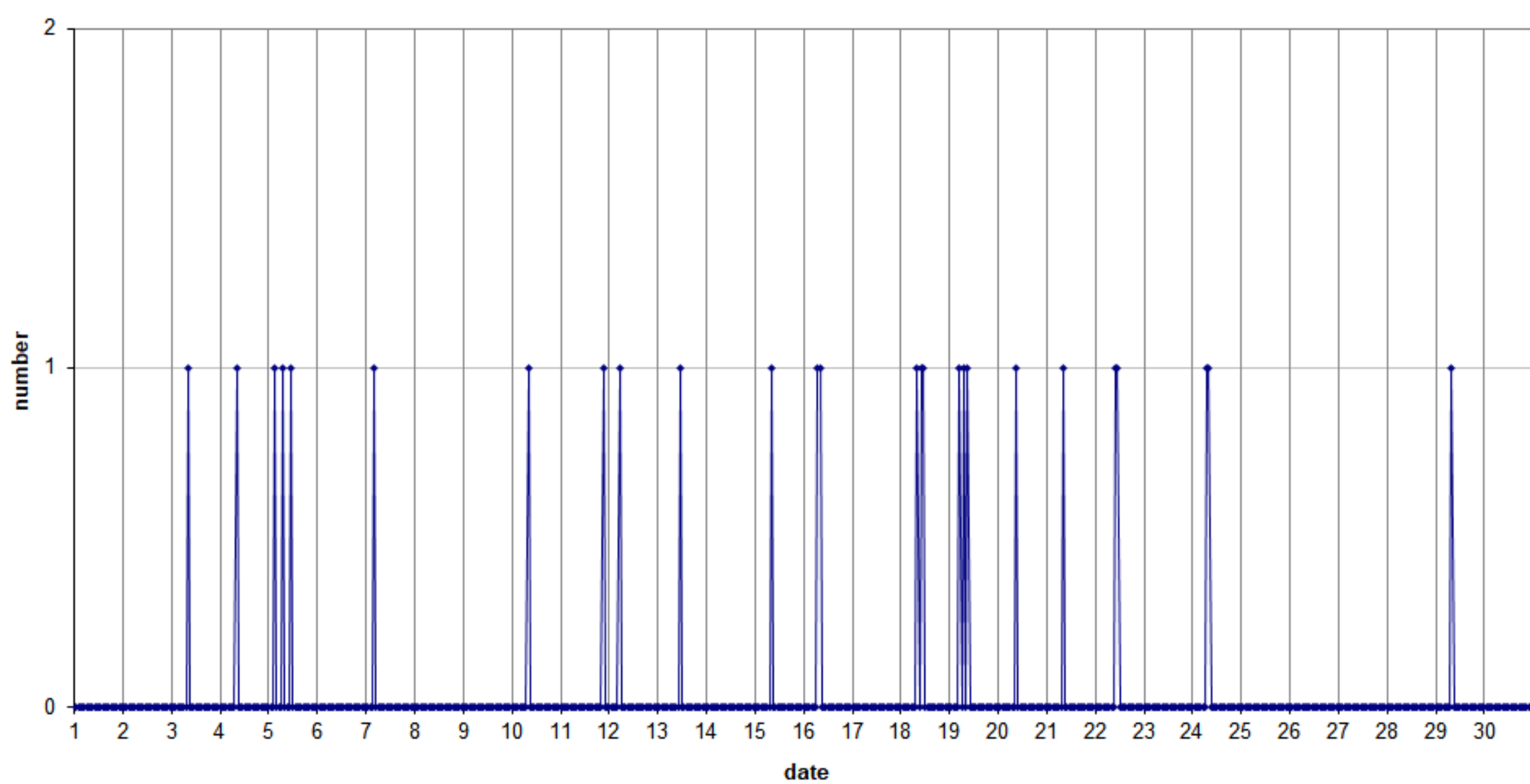
49.99MHz - RadioMeteors November 2022 hourly totals of overdense reflections longer than 1 minute Felix Verbelen (Kamphenhout/BE)
