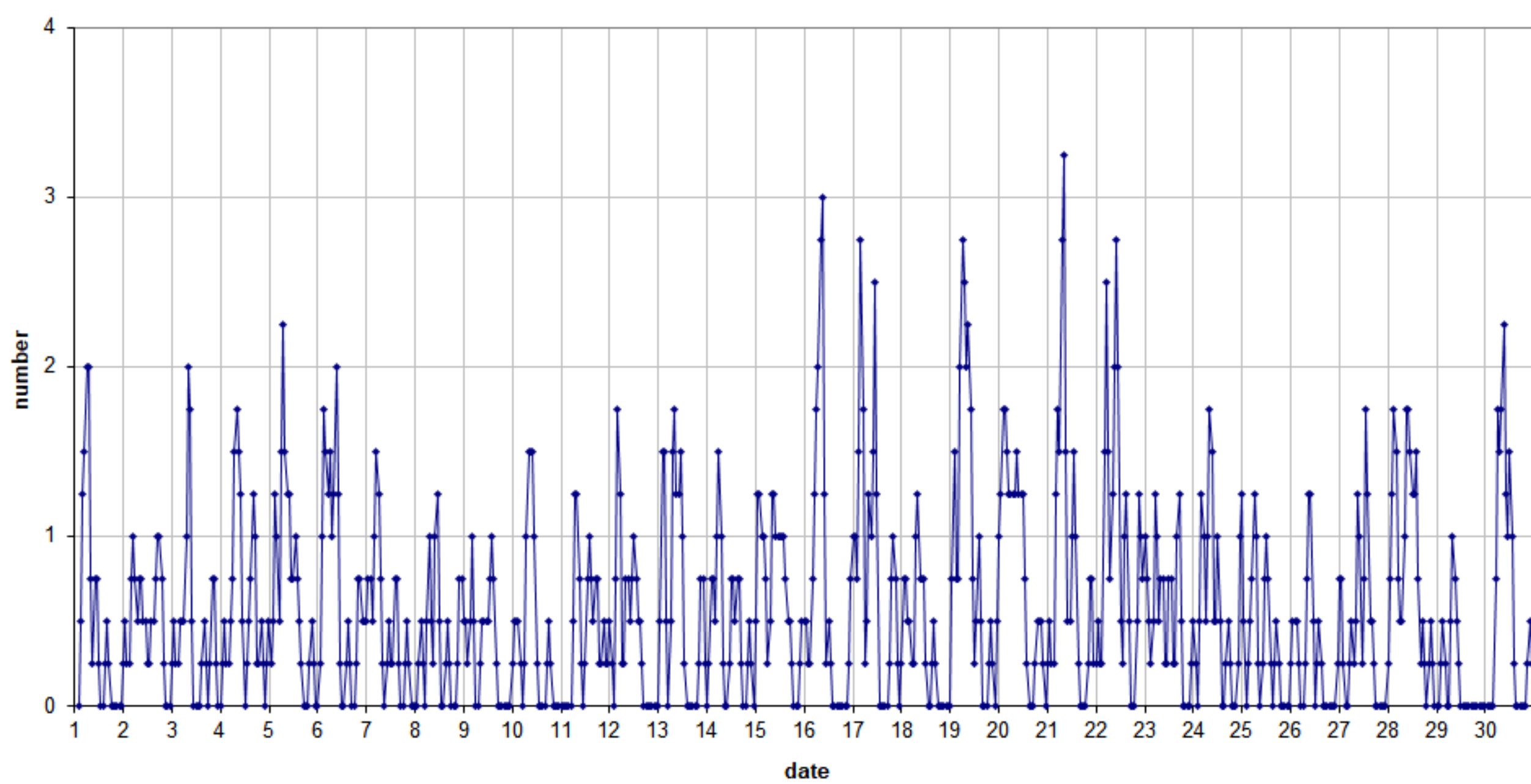
49.99MHz - RadioMeteors November 2022 number of reflections >10 seconds per hour (weighted average) Felix Verbelen (Kamphenhout)
