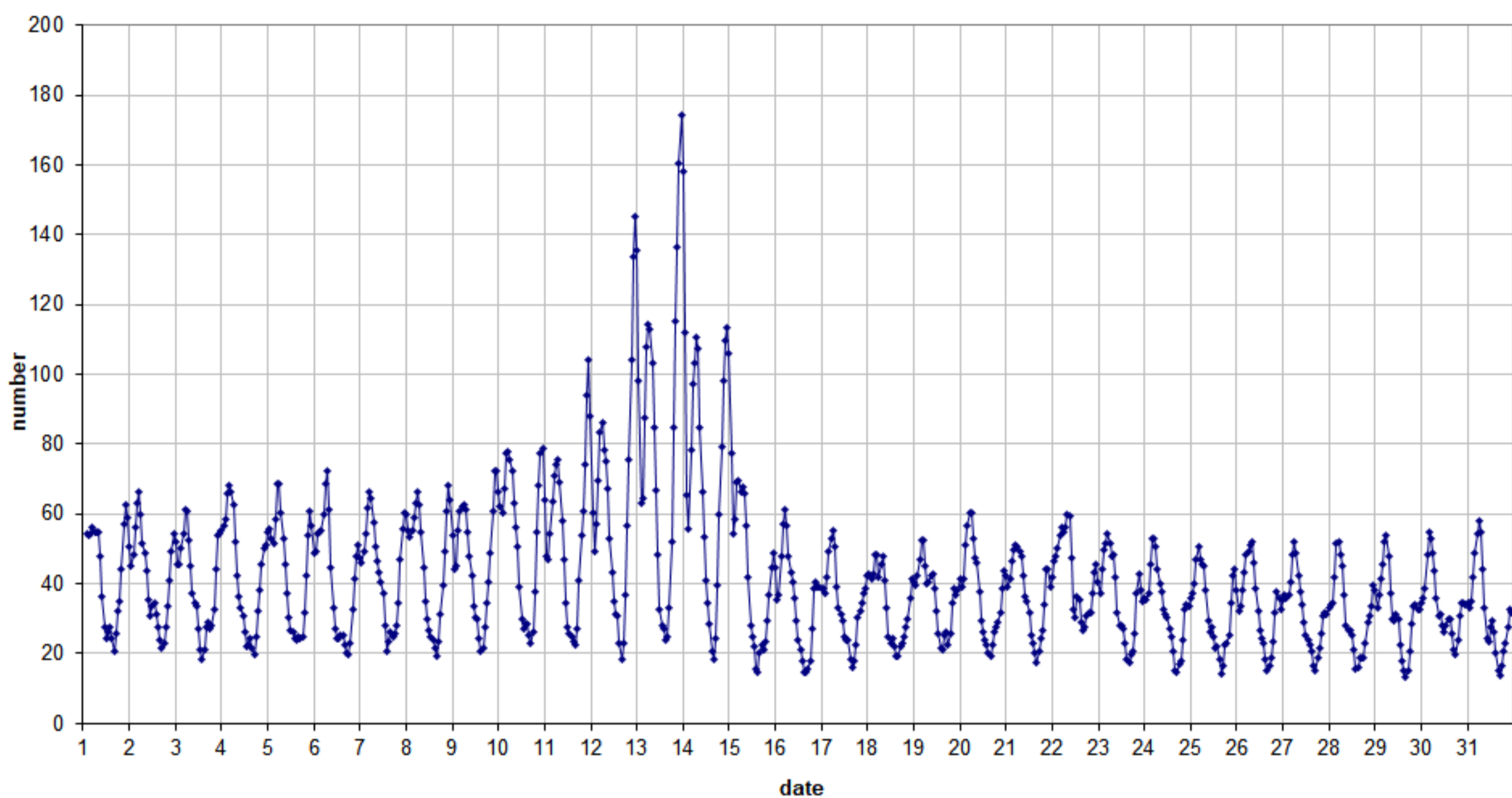
49.99 MHz - RadioMeteors December 2022 number of "all" reflections per hour (weighted average) (automatic count_Mettel5_7Hz) Felix Verbelen (Kamphenhout)
