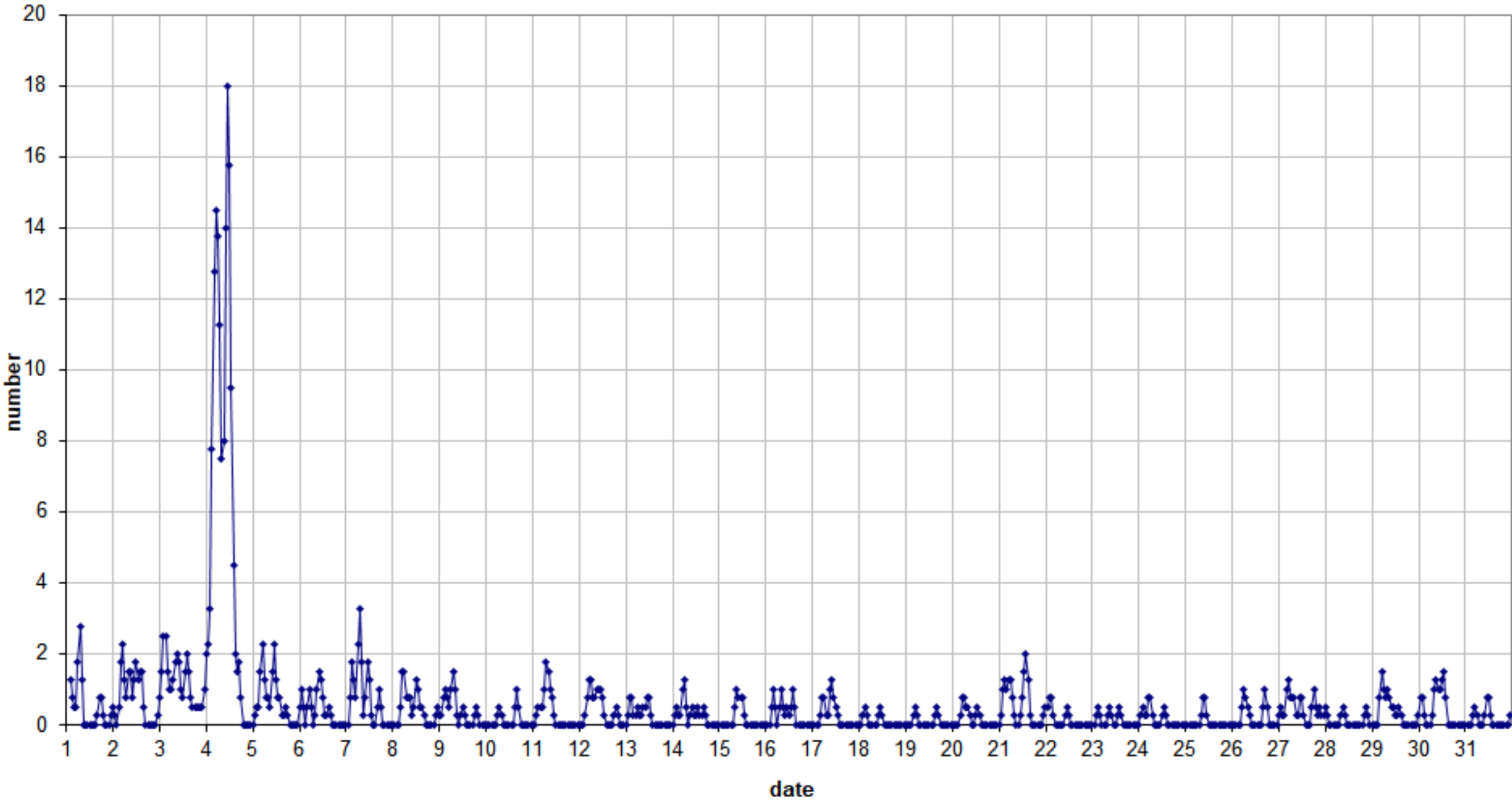
49.99MHz - RadioMeteors January 2023 number of reflections >10 seconds per hour (weighted average) Felix Verbelen (Kampenhout)
