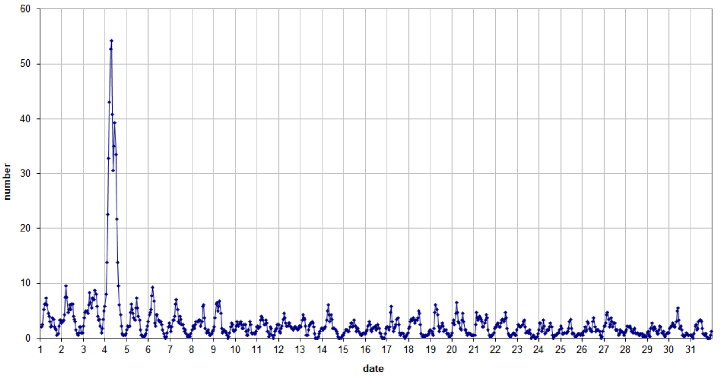
49.99MHz - RadioMeteors January 2023 number of overdense reflections per hour (weighted average) Felix Verbelen (Kampenhout)
