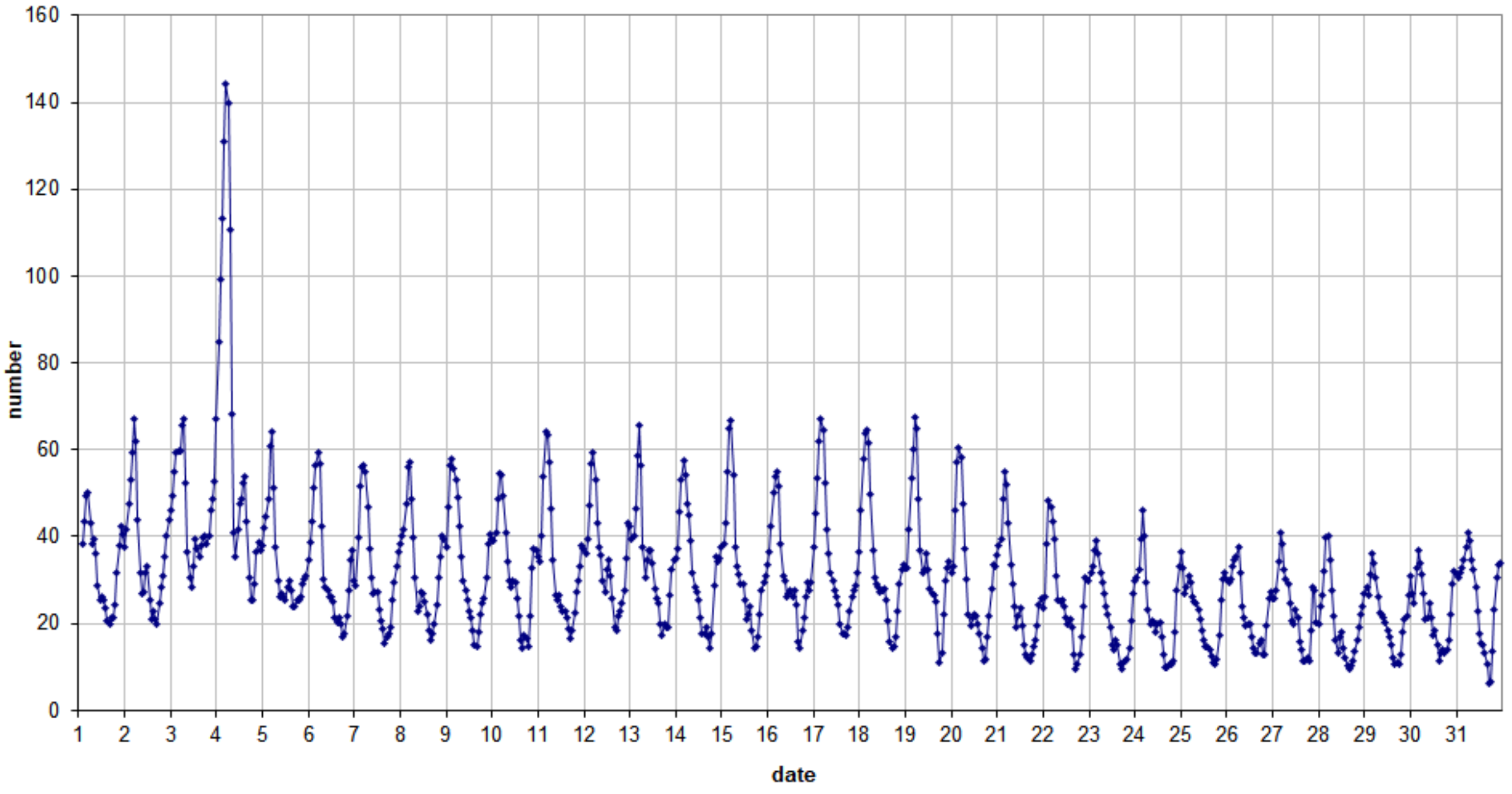
49.99 MHz - RadioMeteors January 2023 number of "all" reflections per hour (weighted average) (automatic count_Mettel5_7Hz) Felix Verbelen (Kampenhout)
