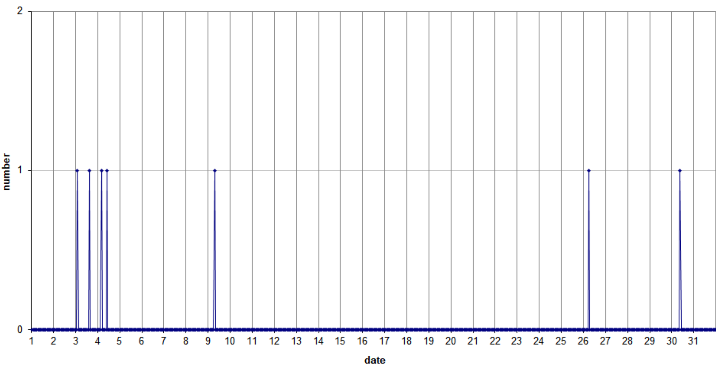
49.99MHz - RadioMeteors January 2023 hourly totals of overdense reflections longer than 1 minute Felix Verbelen (Kampenhout/BE)
