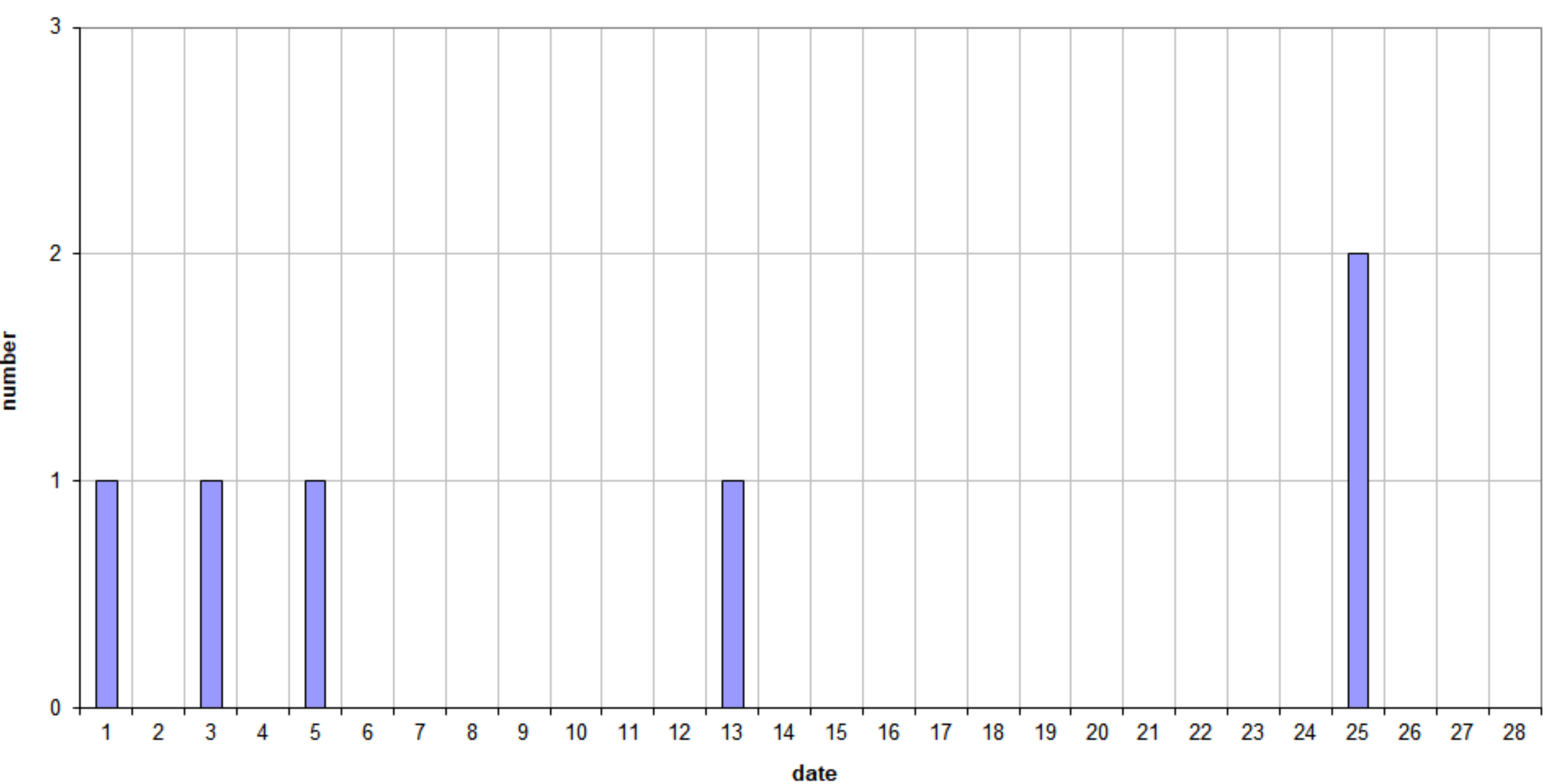
49.99MHz - RadioMeteors February 2023 daily totals of reflections longer than 1 minute Felix Verbelen (Kamphenhout)
