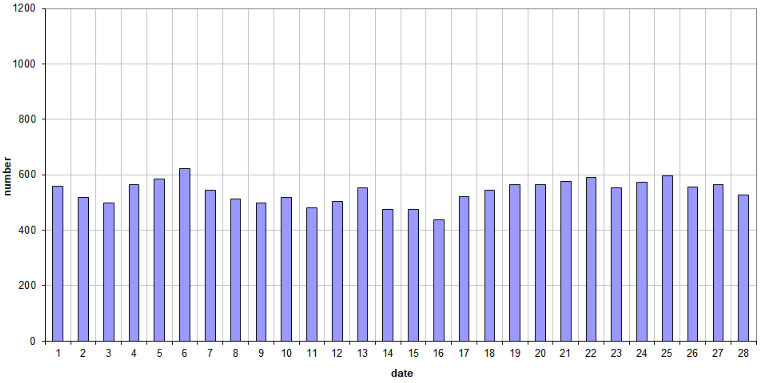
49.99MHz - RadioMeteors February 2023 daily totals of "all" reflections (automatic count_Mettel5_7Hz) Felix Verbelen (Kamphenhout)
