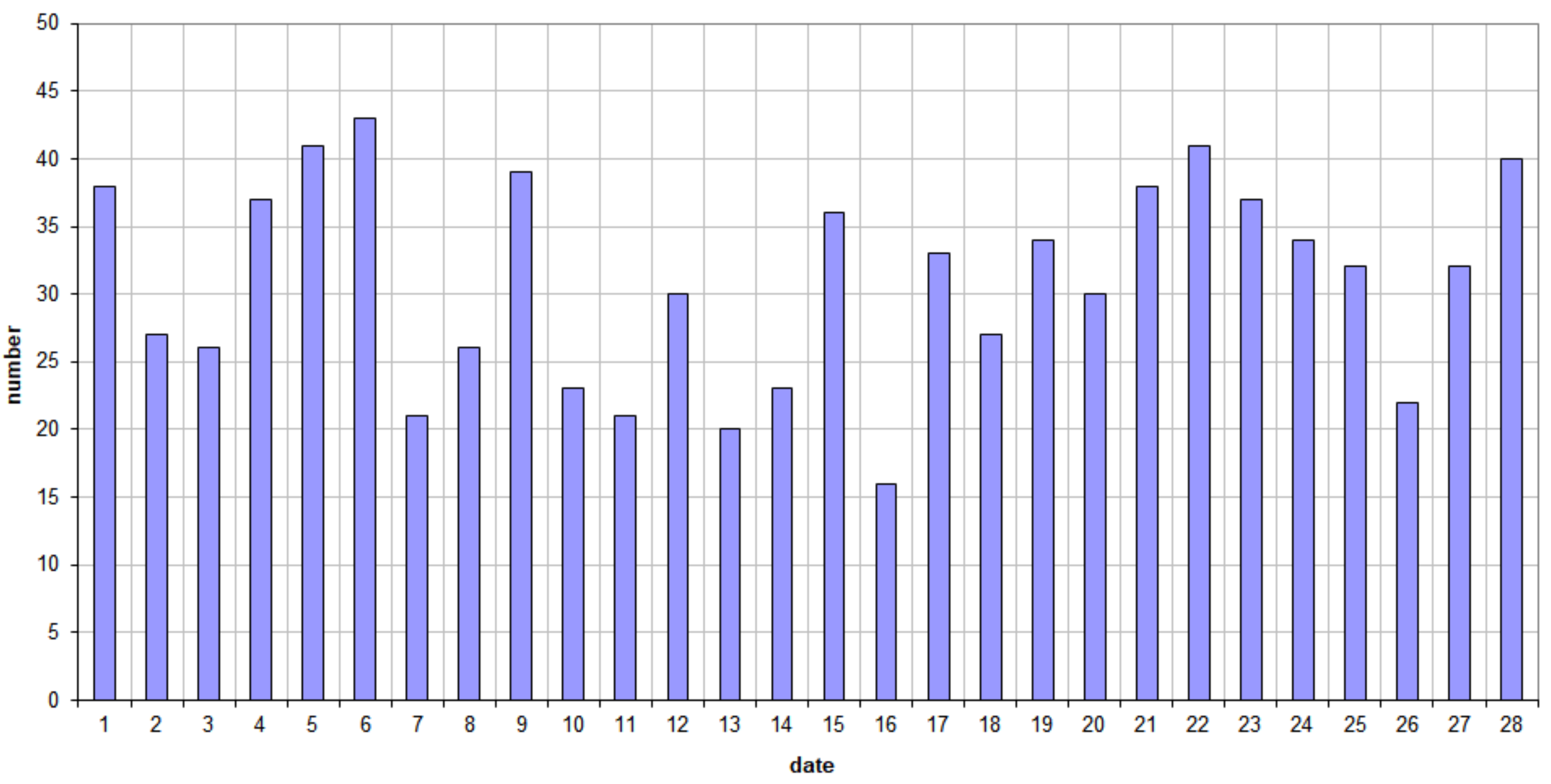
49.99MHz - RadioMeteors February 2023 daily totals of all overdense reflections Felix Verbelen (Kamphenhout)
