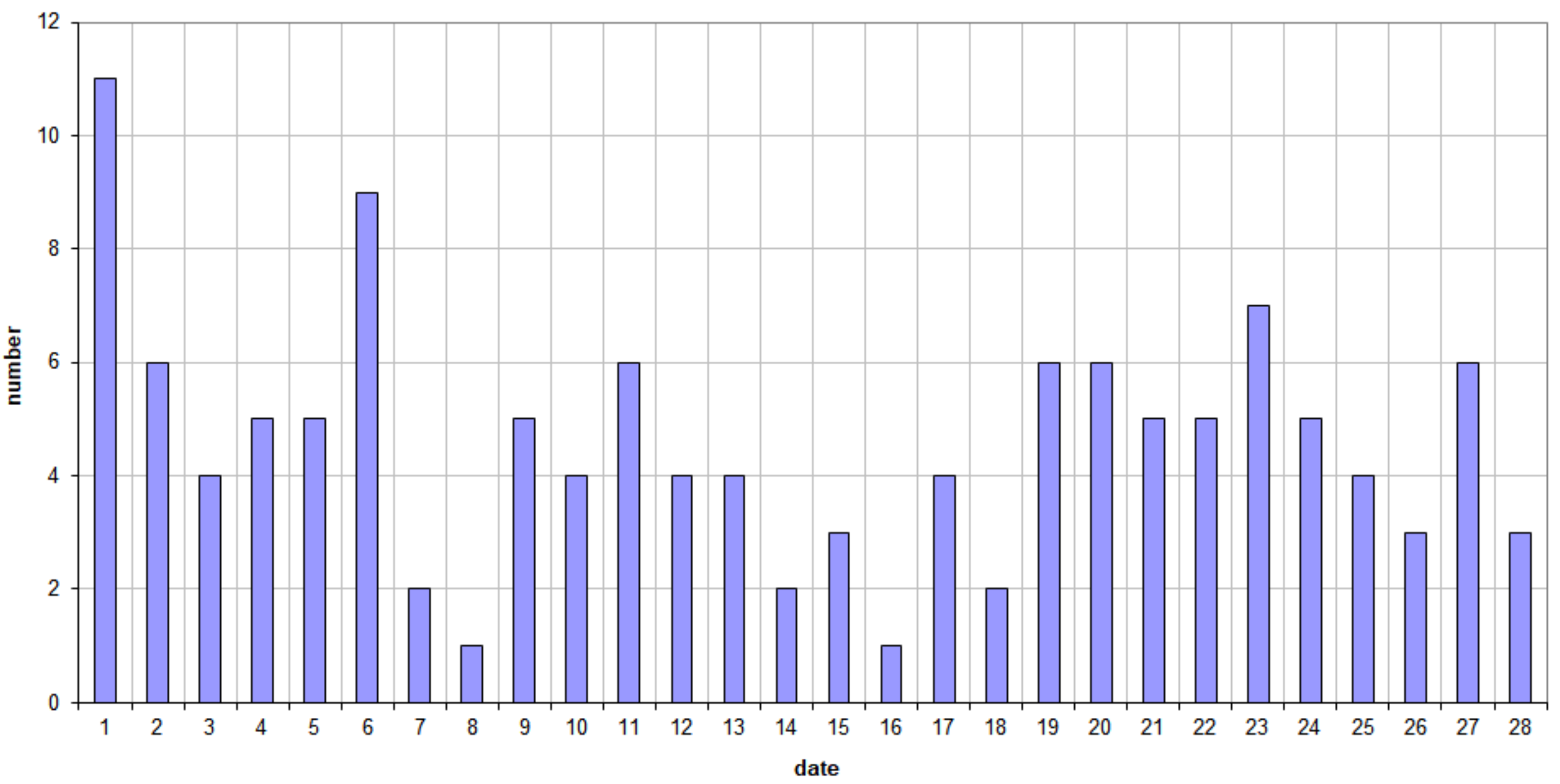
49.99MHz - RadioMeteors February 2023 daily totals of reflections longer than 10 seconds Felix Verbelen (Kamphenhout)
