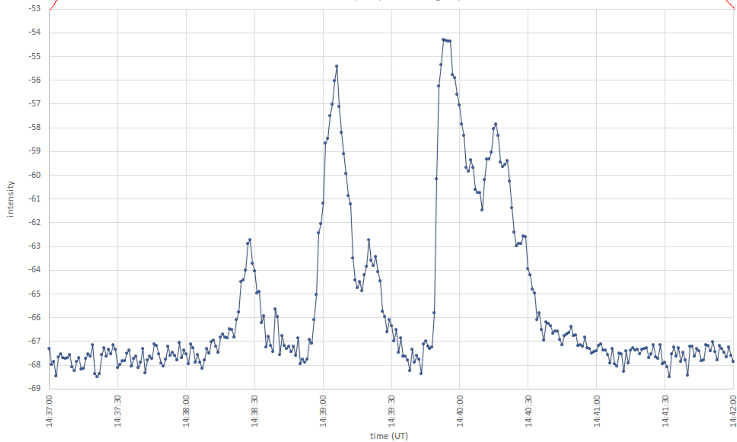
20230304_14:37-14:42 UT_49.99 MHz_noise Felix Verbelen (Kampenhout/Belgium)
