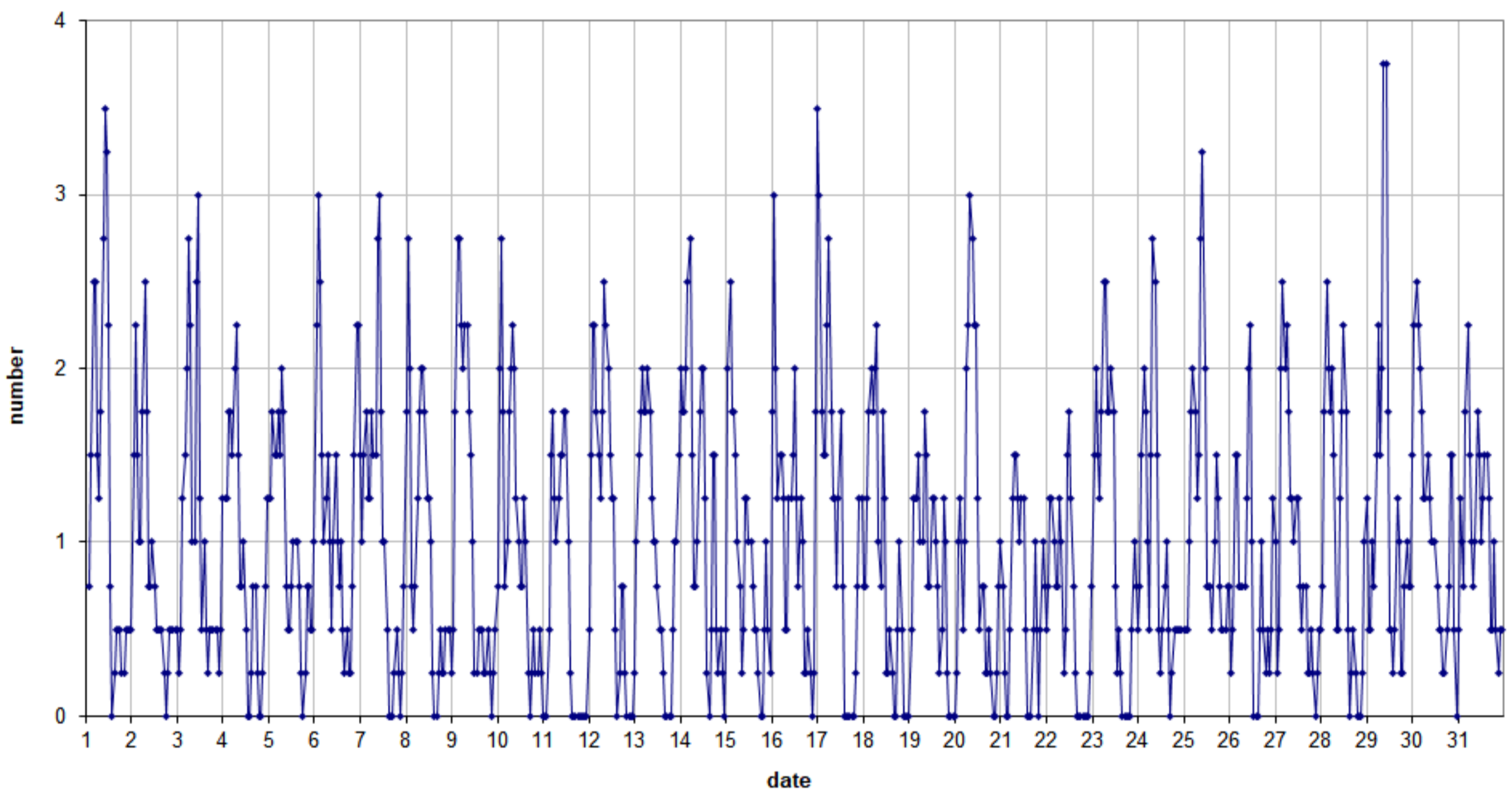
49.99MHz - RadioMeteors March 2023 number of overdense reflections per hour (weighted average) Felix Verbelen (Kamphenhout)
