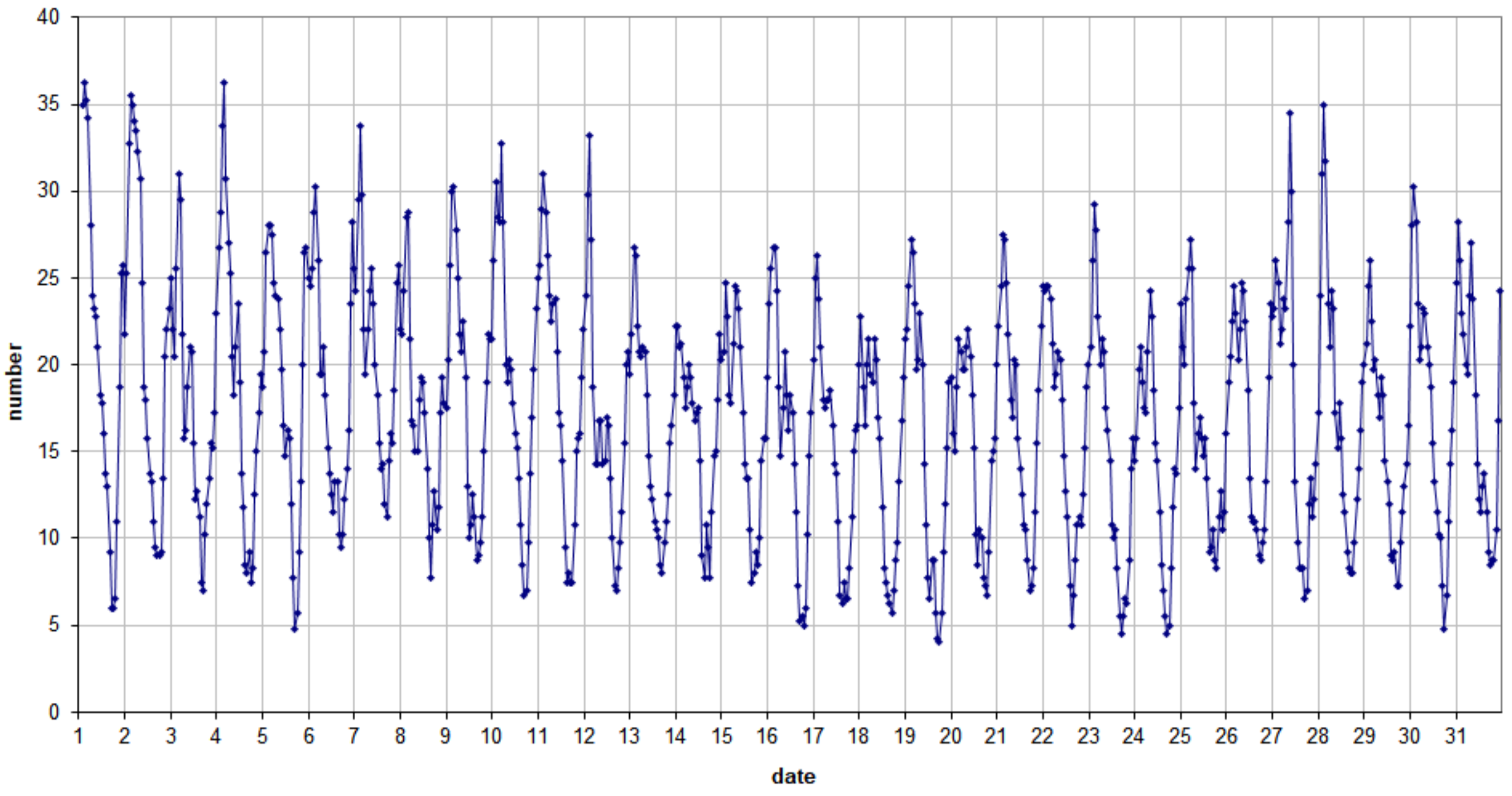
49.99 MHz - RadioMeteors March 2023 number of "all" reflections per hour (weighted average) (automatic count_Mettel5_7Hz) Felix Verbelen (Kamphenhout)
