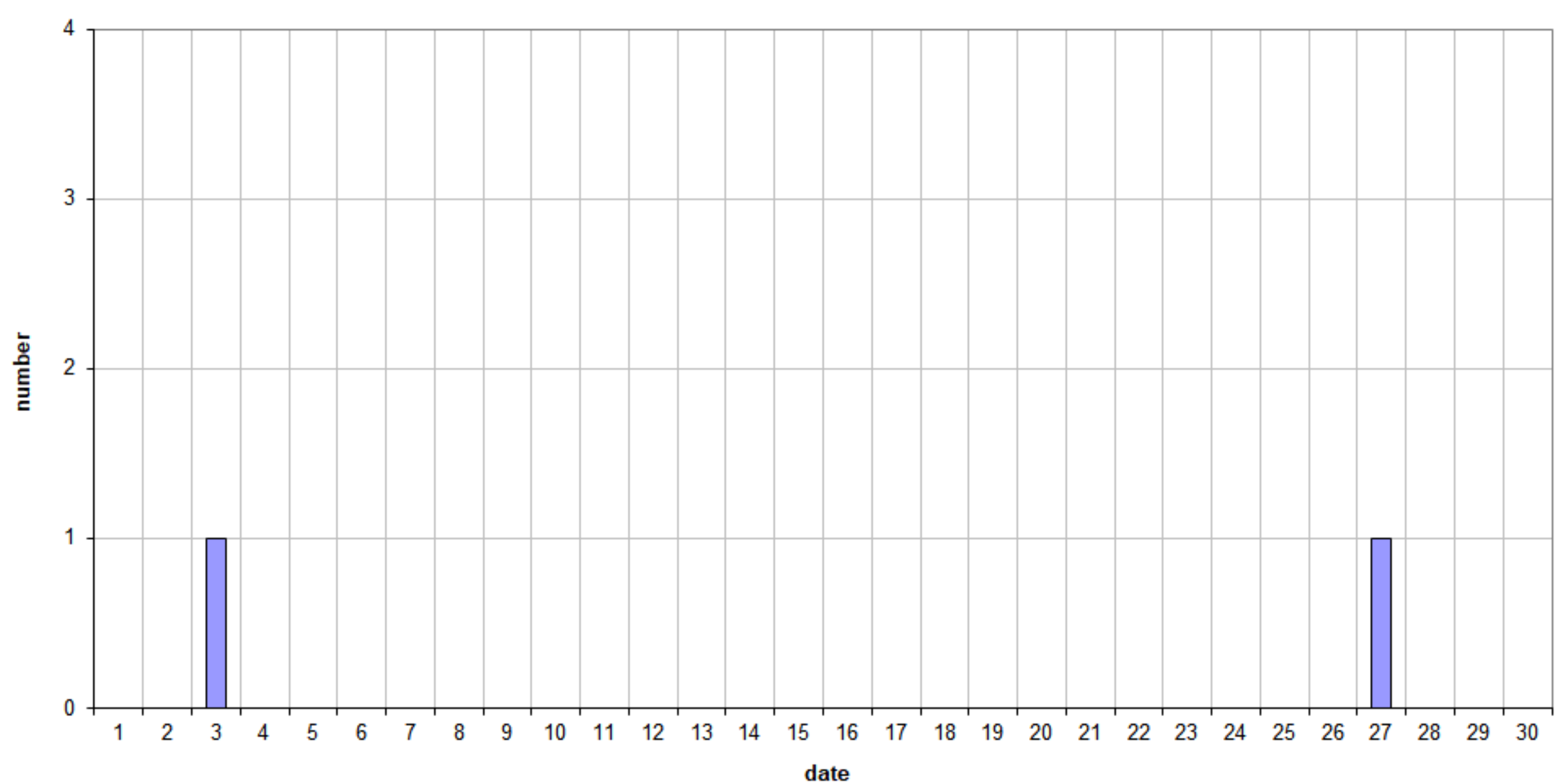
49.99MHz - RadioMeteors April 2023 daily totals of reflections longer than 1 minute Felix Verbelen (Kampenhout)
