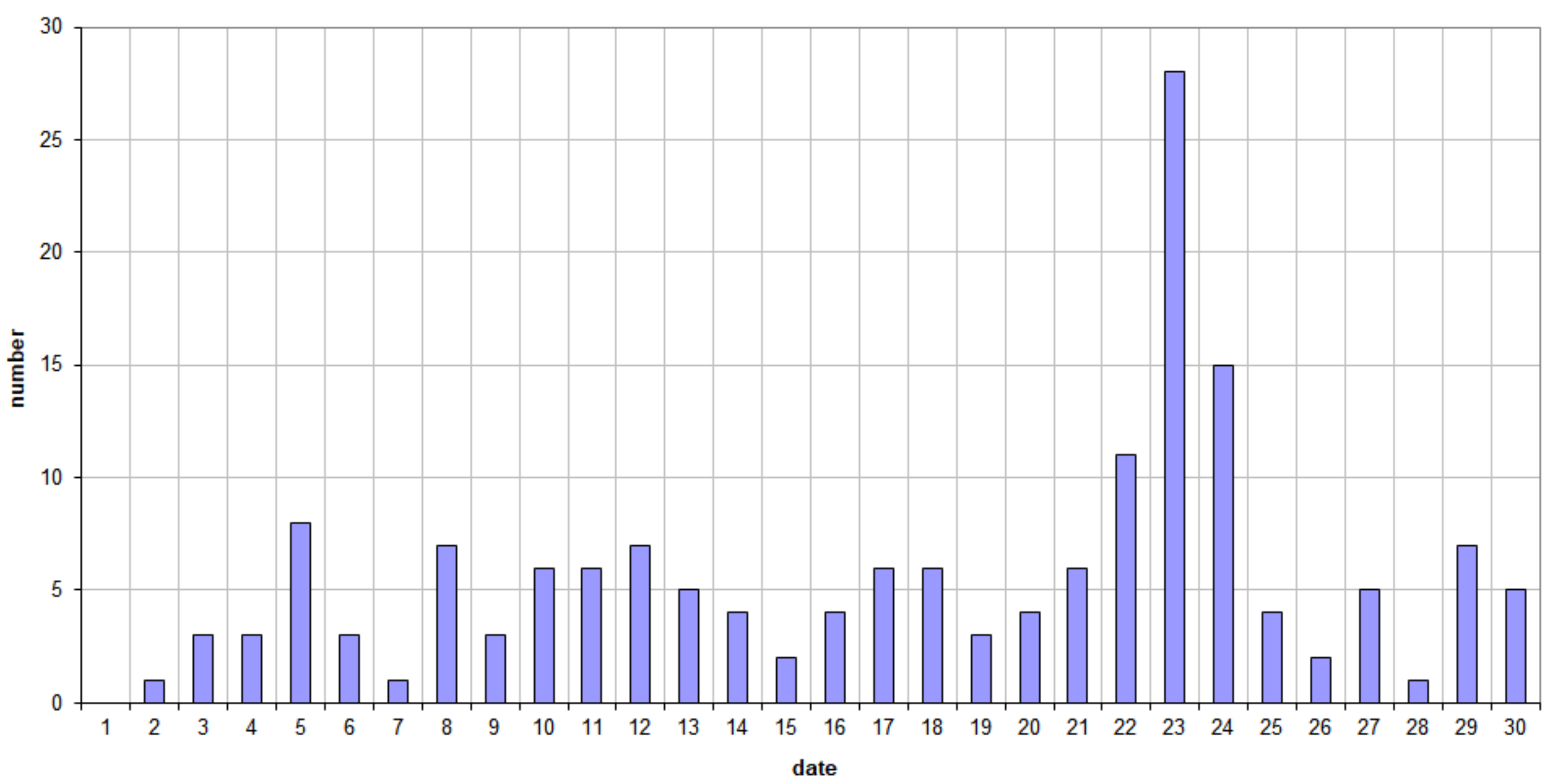
49.99MHz - RadioMeteors April 2023 daily totals of reflections longer than 10 seconds Felix Verbelen (Kampenhout)
