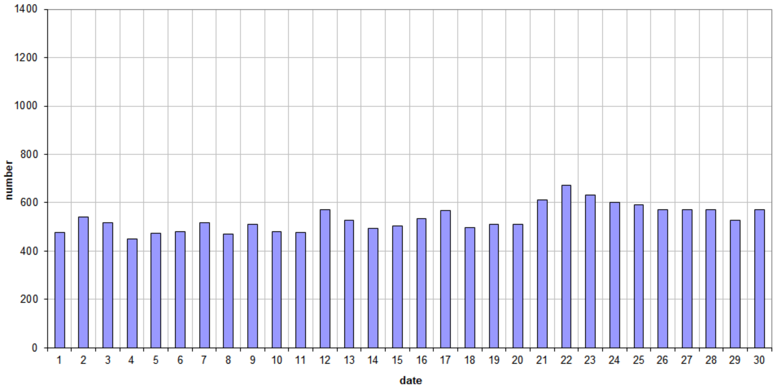
49.99MHz - RadioMeteors April 2023 daily totals of "all" reflections (automatic count_Mette15_7Hz) Felix Verbelen (Kampenhout)
