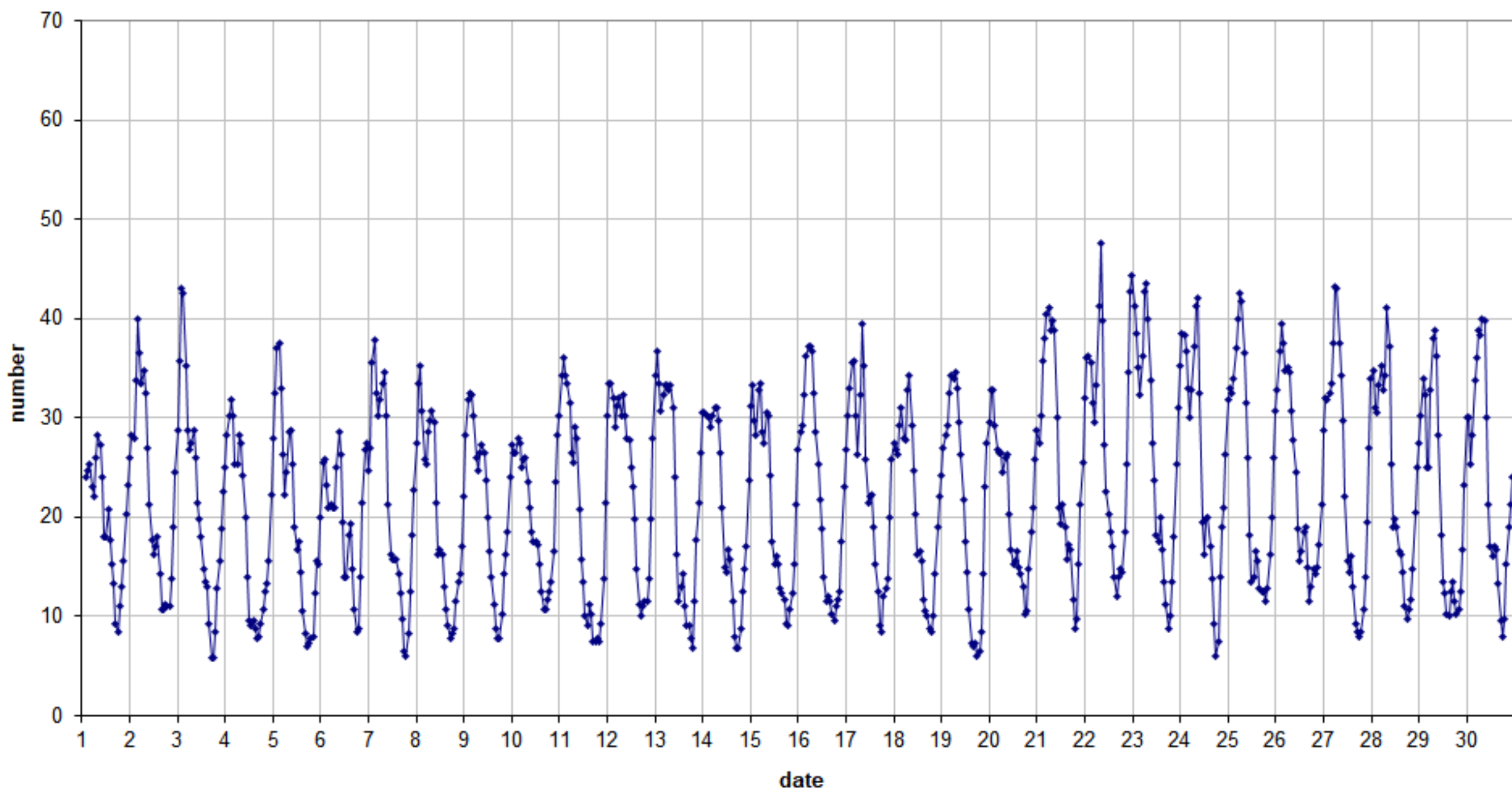
49.99 MHz - RadioMeteors April 2023 number of "all" reflections per hour (weighted average) (automatic count_Mette15_7Hz) Felix Verbelen (Kampenhout)
