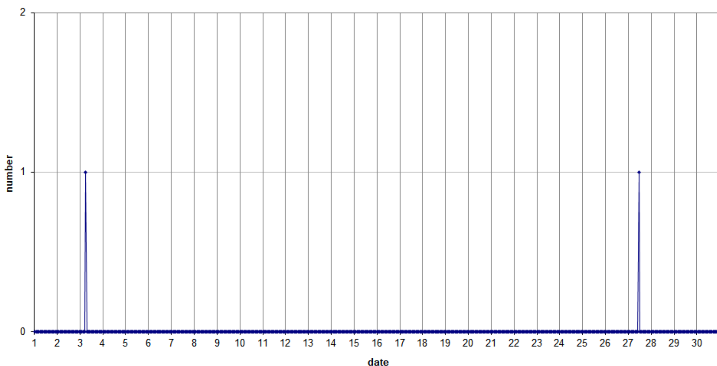
49.99MHz - RadioMeteors April 2023 hourly totals of overdense reflections longer than 1 minute Felix Verbelen (Kampenhout/BE)
