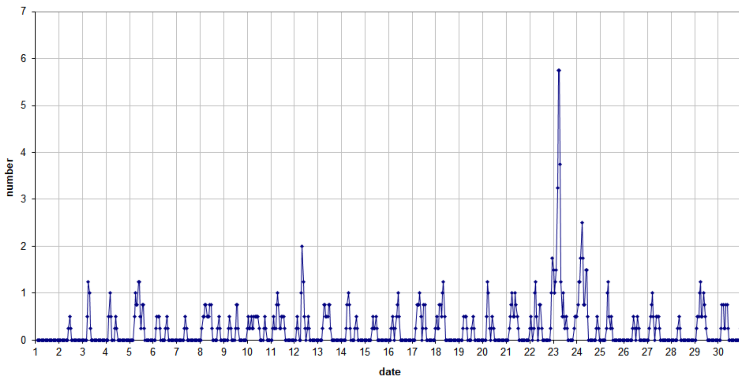
49.99MHz - RadioMeteors April 2023 number of reflections >10 seconds per hour (weighted average) Felix Verbelen (Kampenhout)
