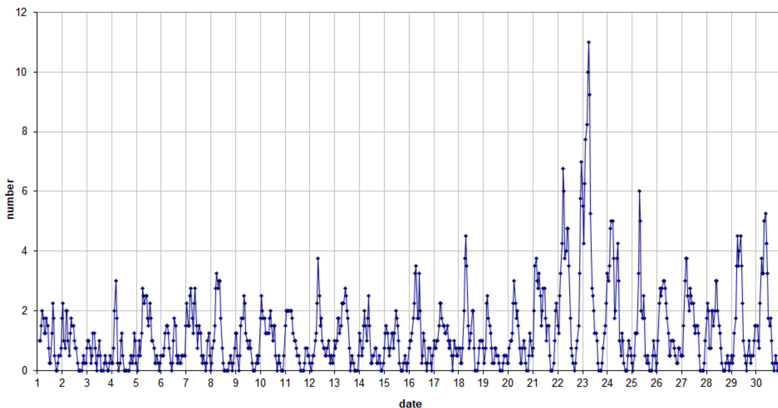
49.99MHz - RadioMeteors April 2023 number of overdense reflections per hour (weighted average) Felix Verbelen (Kampenhout)
