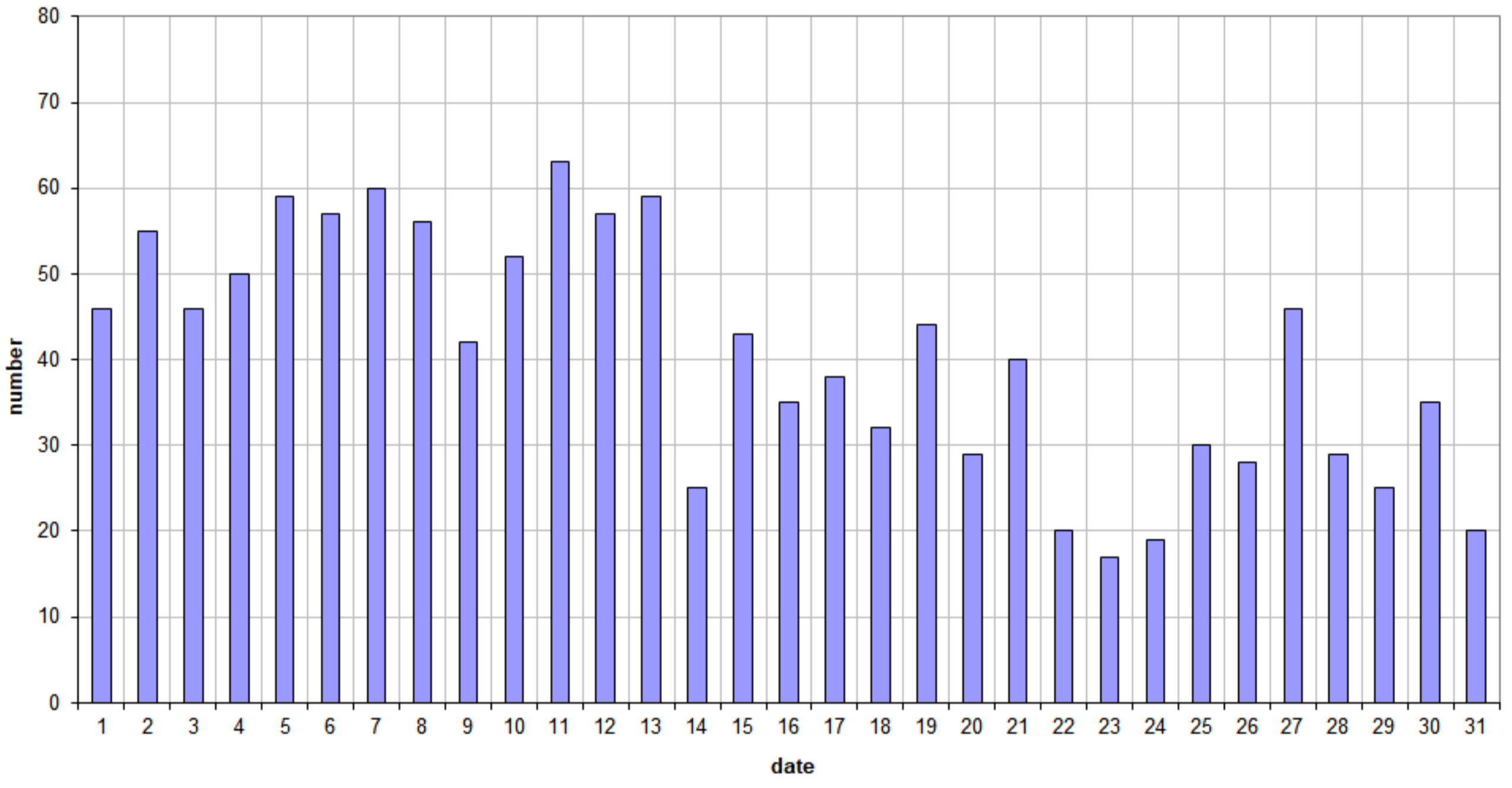
49.99MHz - RadioMeteors May 2023 daily totals of all overdense reflections Felix Verbelen (Kamphenhout)
