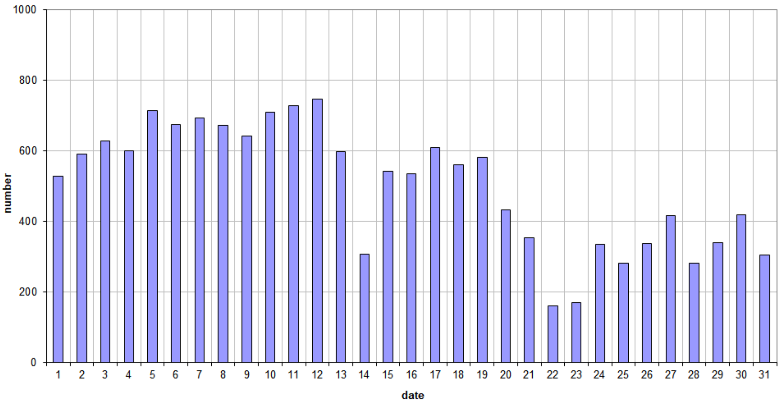
49.99MHz - RadioMeteors May 2023 daily totals of "all" reflections (automatic count_Mettel5_7Hz) Felix Verbelen (Kamphenhout)
