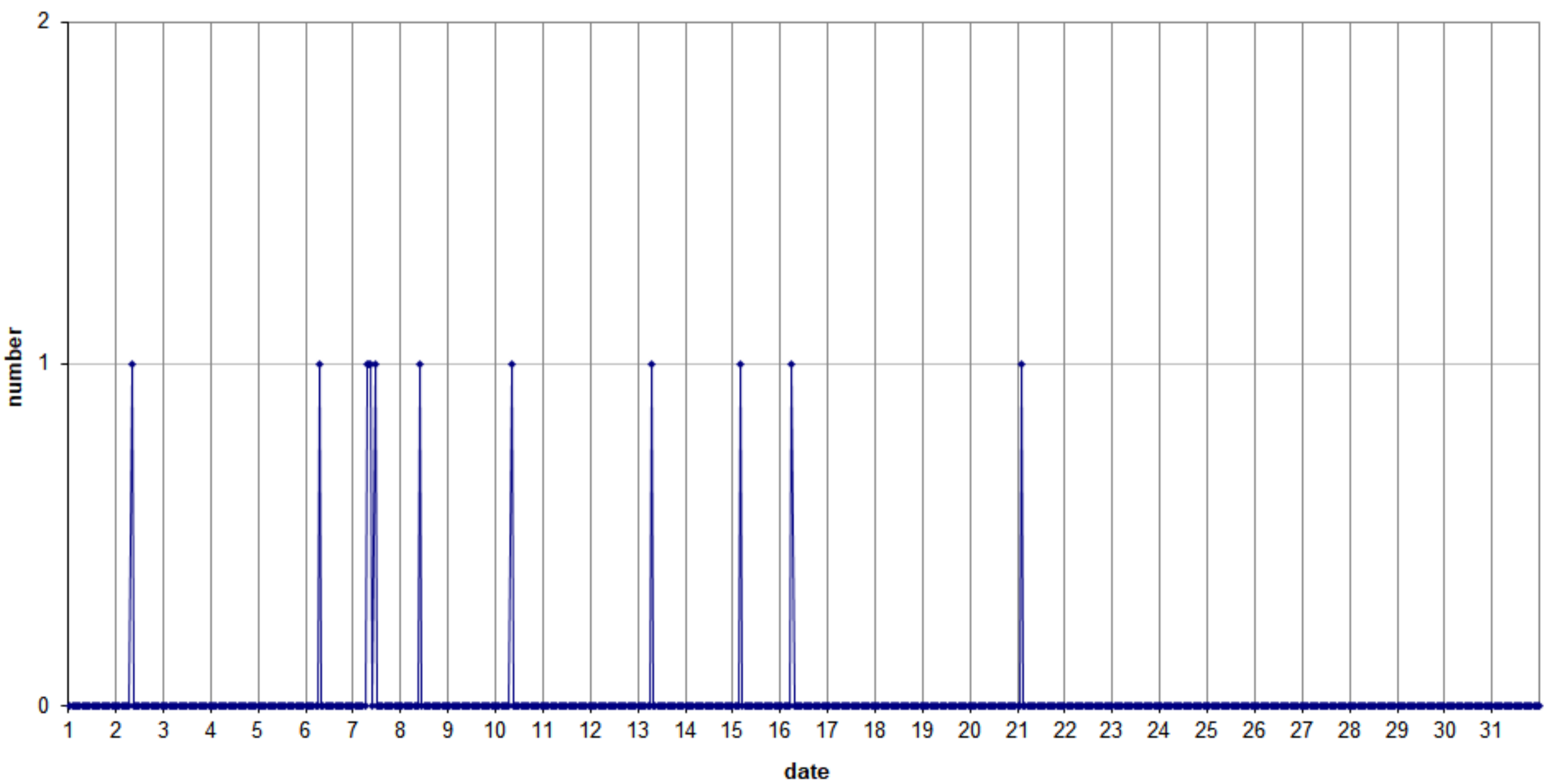
49.99MHz - RadioMeteors May 2023 hourly totals of overdense reflections longer than 1 minute Felix Verbelen (Kampenhout/BE)
