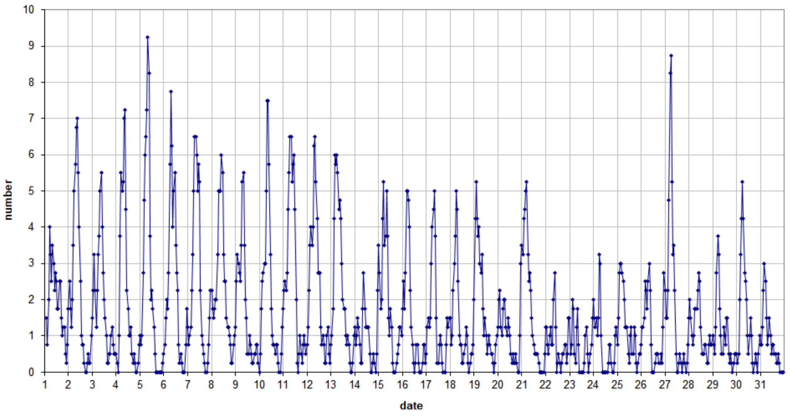
49.99MHz - RadioMeteors May 2023 number of overdense reflections per hour (weighted average) Felix Verbelen (Kampenhout)
