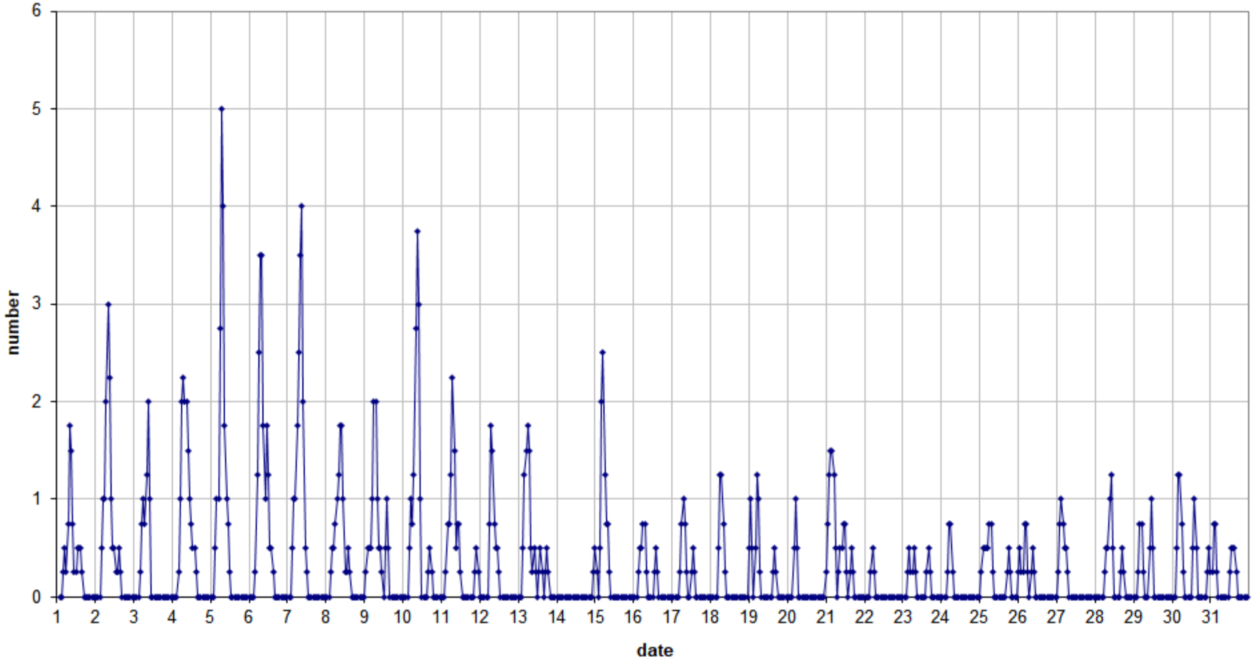
49.99MHz - RadioMeteors May 2023 number of reflections >10 seconds per hour (weighted average) Felix Verbelen (Kampenhout)
