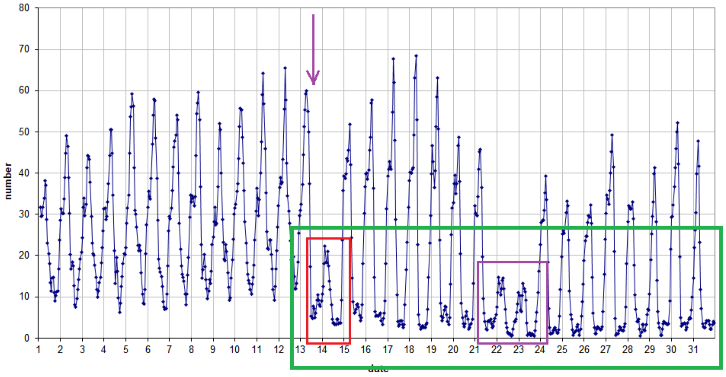
49.99 MHz - RadioMeteors May 2023 number of "all" reflections per hour (weighted average) (automatic count_Mettel5_7Hz) Felix Verbelen (Kampenhout)
