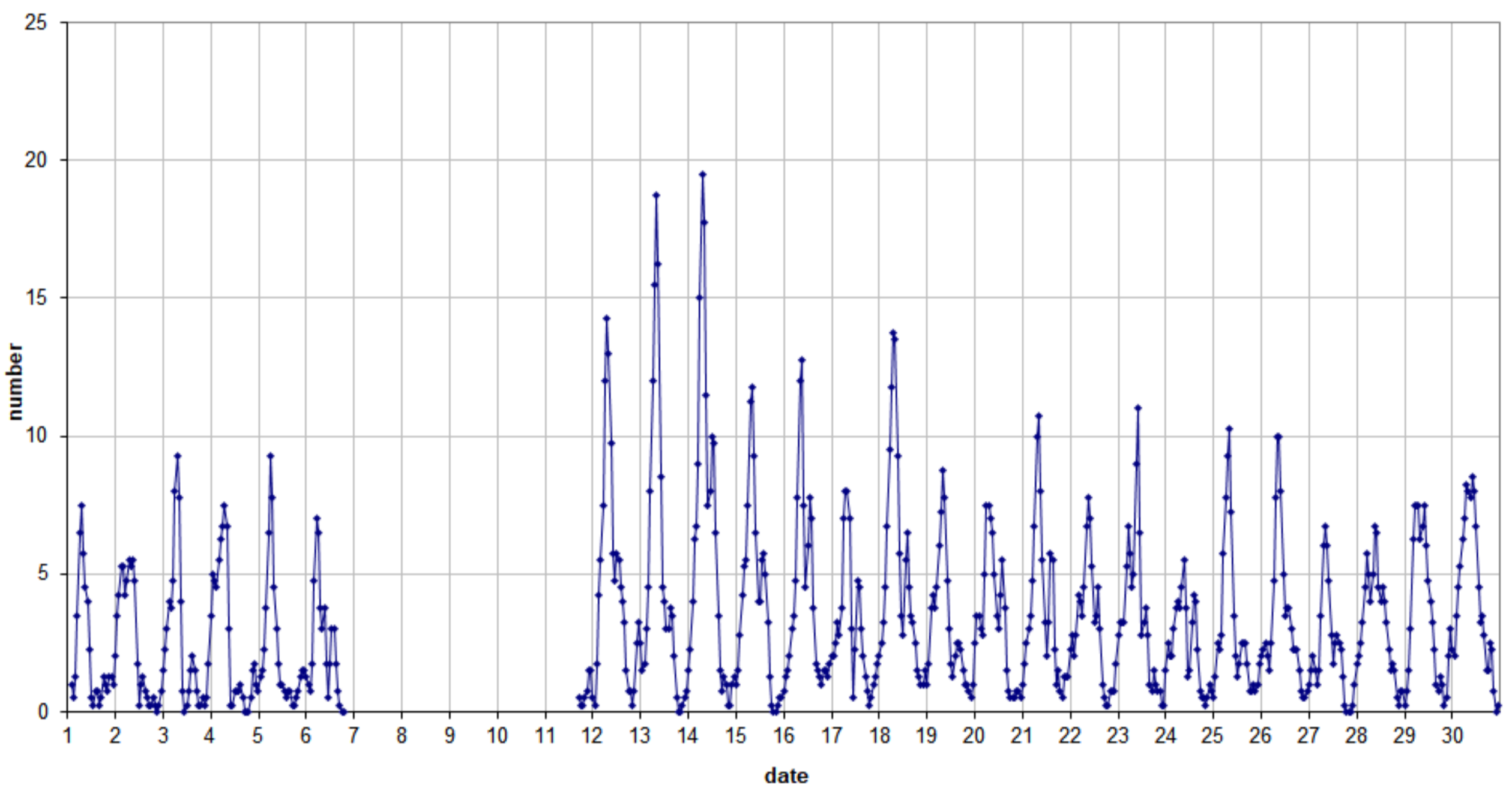
49.99MHz - RadioMeteors June 2023 number of overdense reflections per hour (weighted average) Felix Verbelen (Kampenhout)
