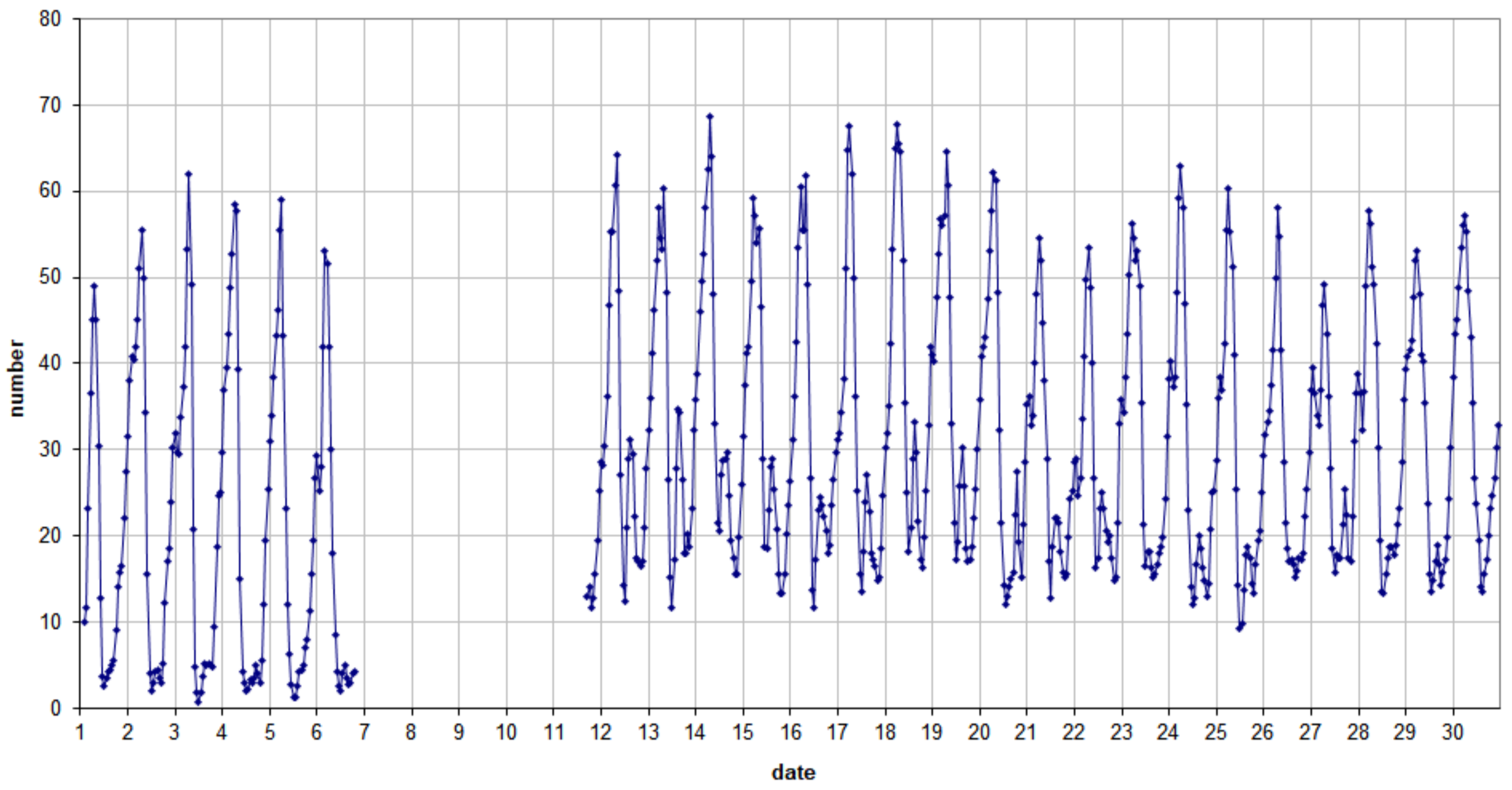
49.99 MHz - RadioMeteors June 2023 number of "all" reflections per hour (weighted average) (automatic count_Mettel5_7Hz) Felix Verbelen (Kampenhout)
