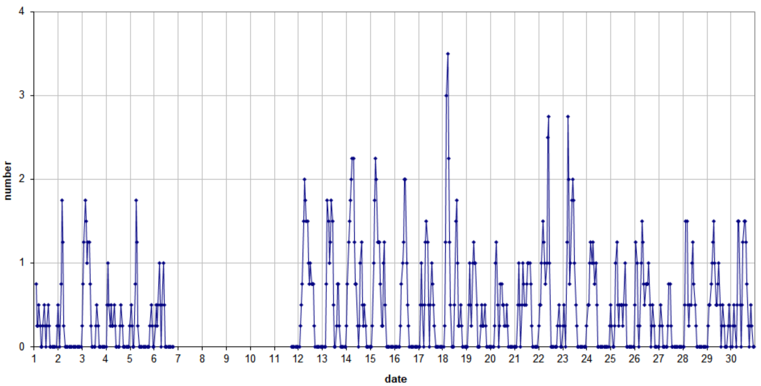
49.99MHz - RadioMeteors June 2023 number of reflections >10 seconds per hour (weighted average) Felix Verbelen (Kampenhout)
