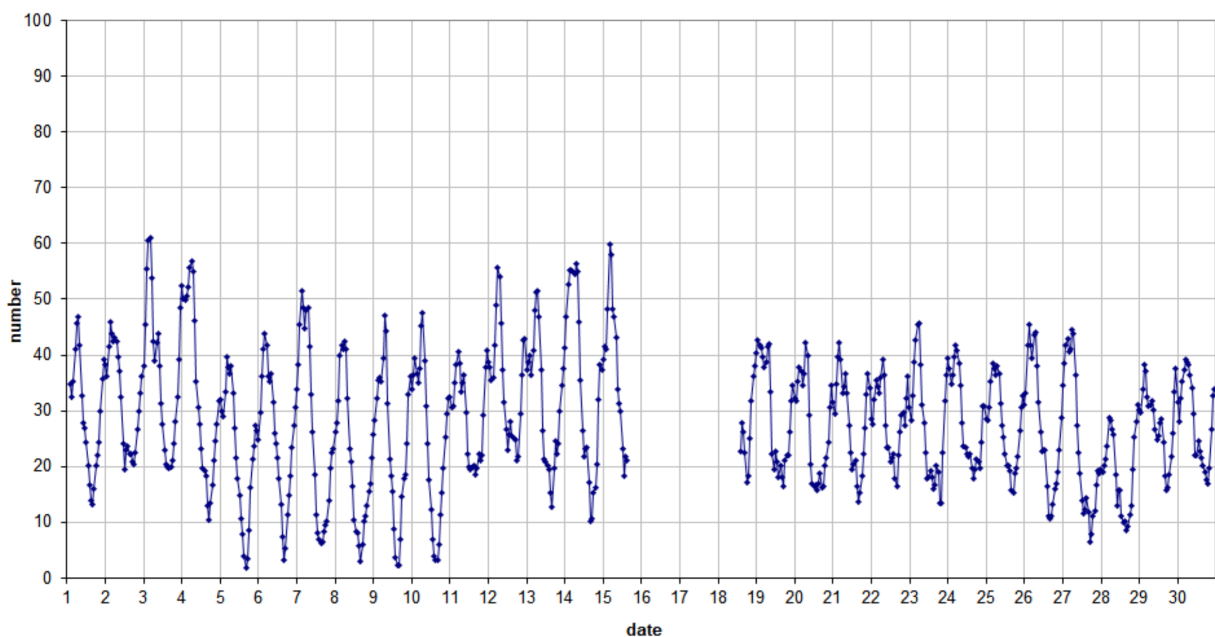
49.99 MHz - RadioMeteors September 2023 number of "all" reflections per hour (weighted average) (automatic count_Mettel5_7Hz) Felix Verbelen (Kampenhout)
