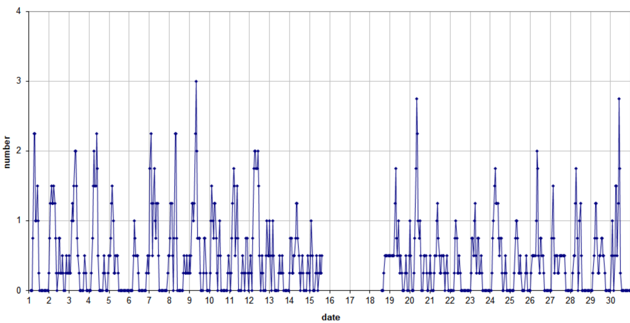
49.99MHz - RadioMeteors September 2023 number of reflections >10 seconds per hour (weighted average) Felix Verbelen (Kampenhout)
