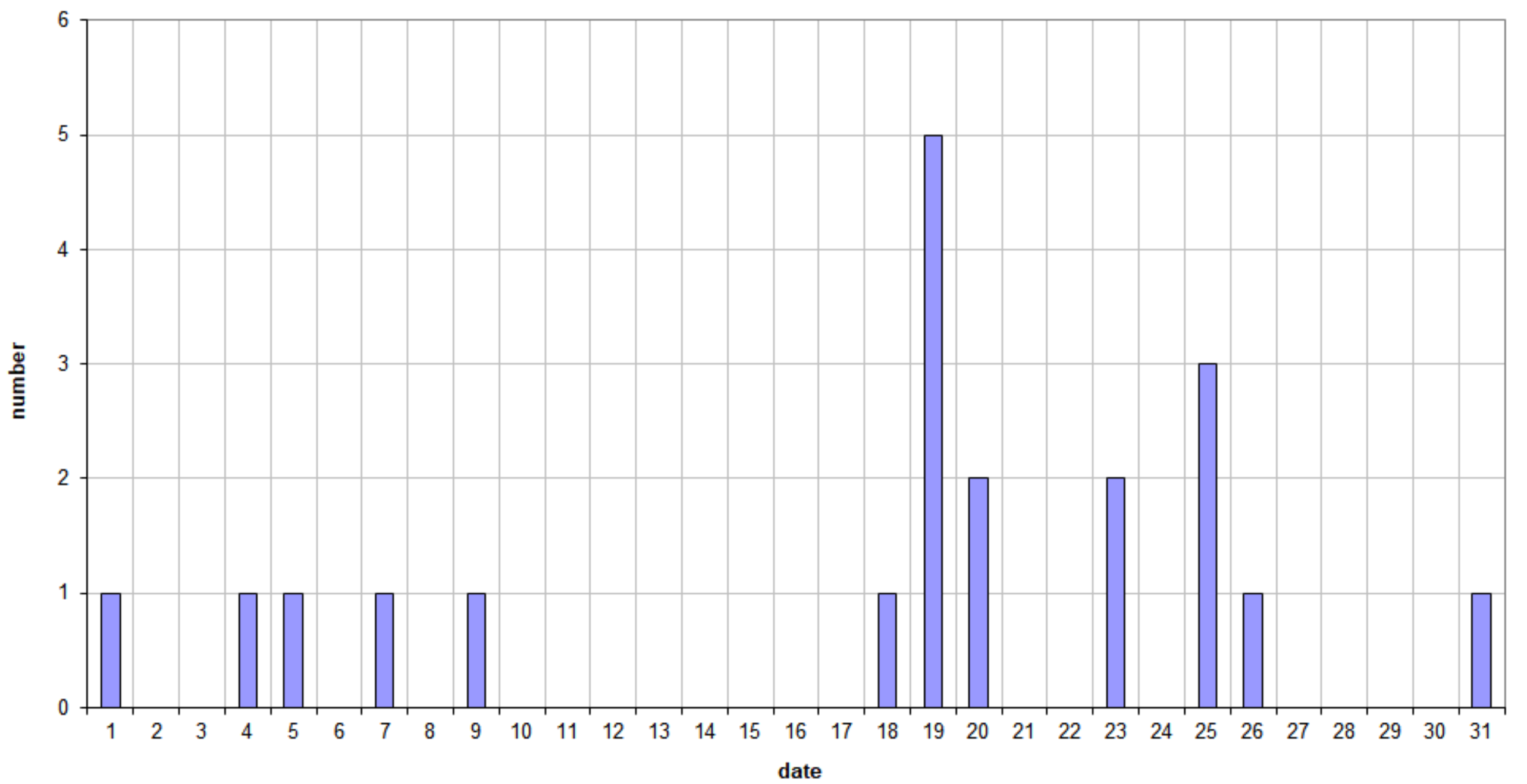
49.99MHz - RadioMeteors October 2023 daily totals of reflections longer than 1 minute Felix Verbelen (Kampenhout)
