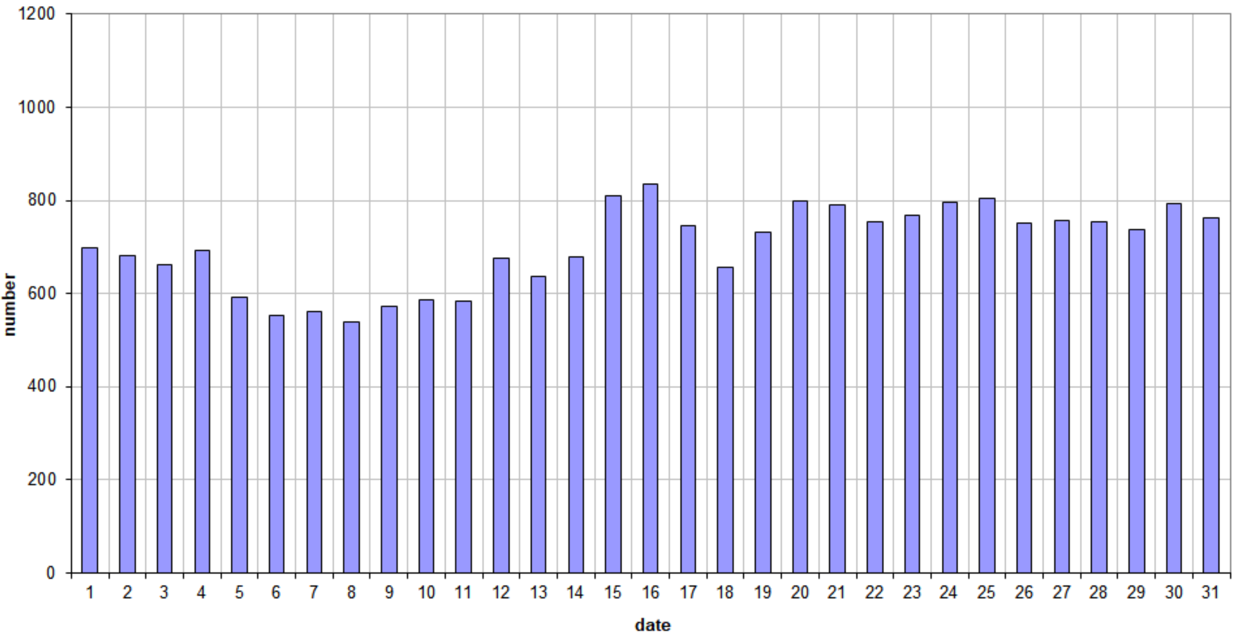
49.99MHz - RadioMeteors October 2023 daily totals of "all" reflections (automatic count_Mettel5_7Hz) Felix Verbelen (Kampenhout)
