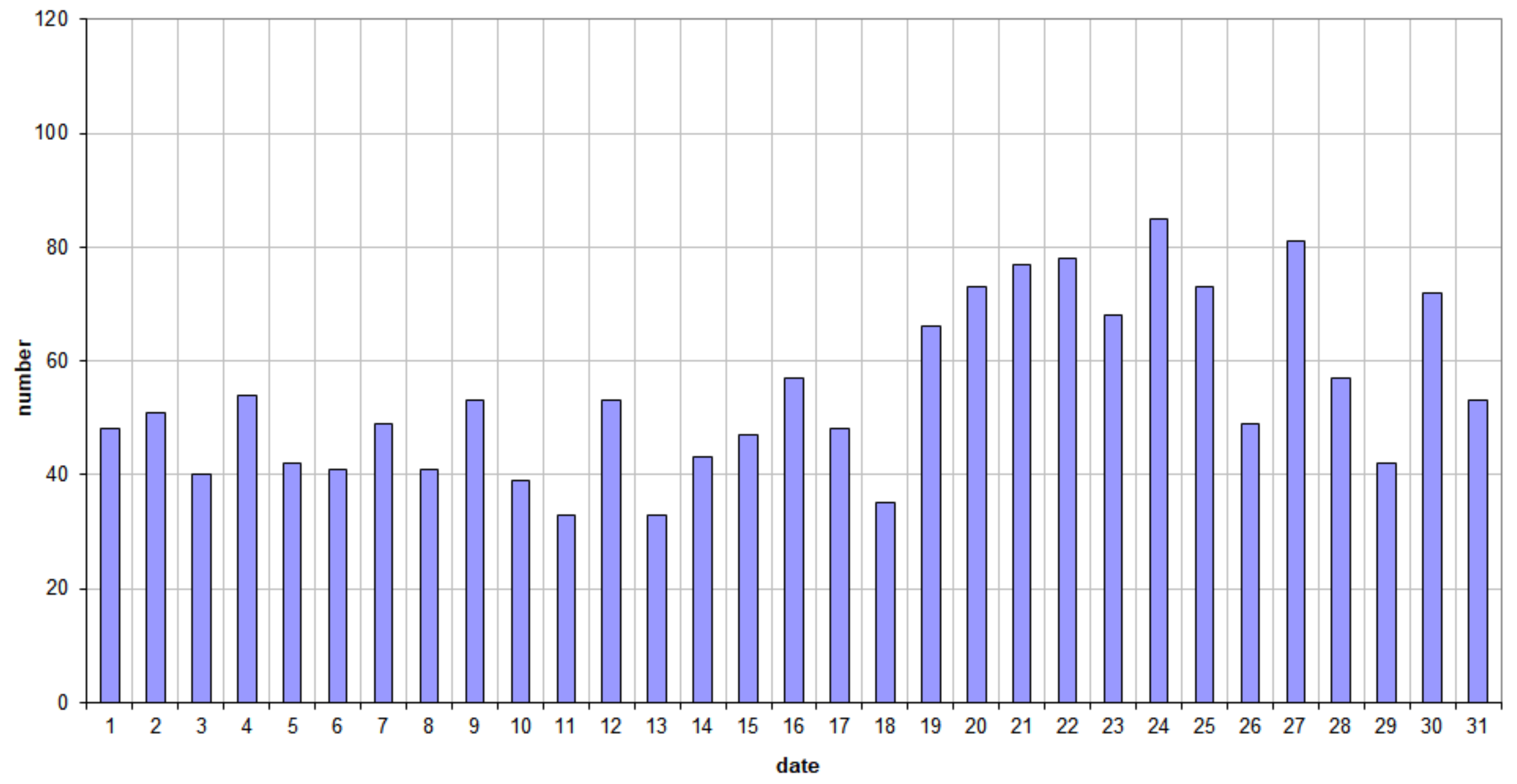
49.99MHz - RadioMeteors October 2023 daily totals of all overdense reflections Felix Verbelen (Kampenhout)
