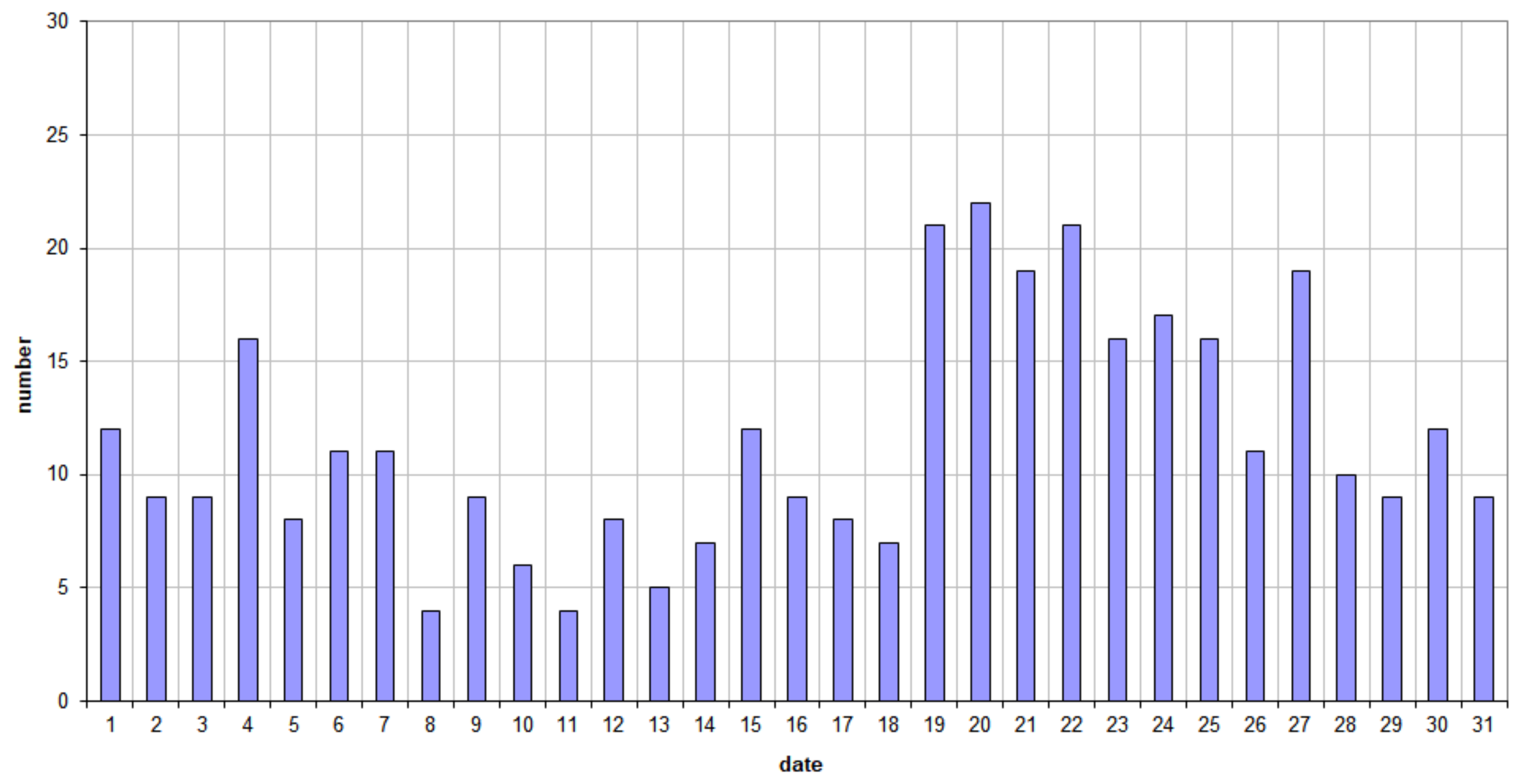
49.99MHz - RadioMeteors October 2023 daily totals of reflections longer than 10 seconds Felix Verbelen (Kampenhout)
