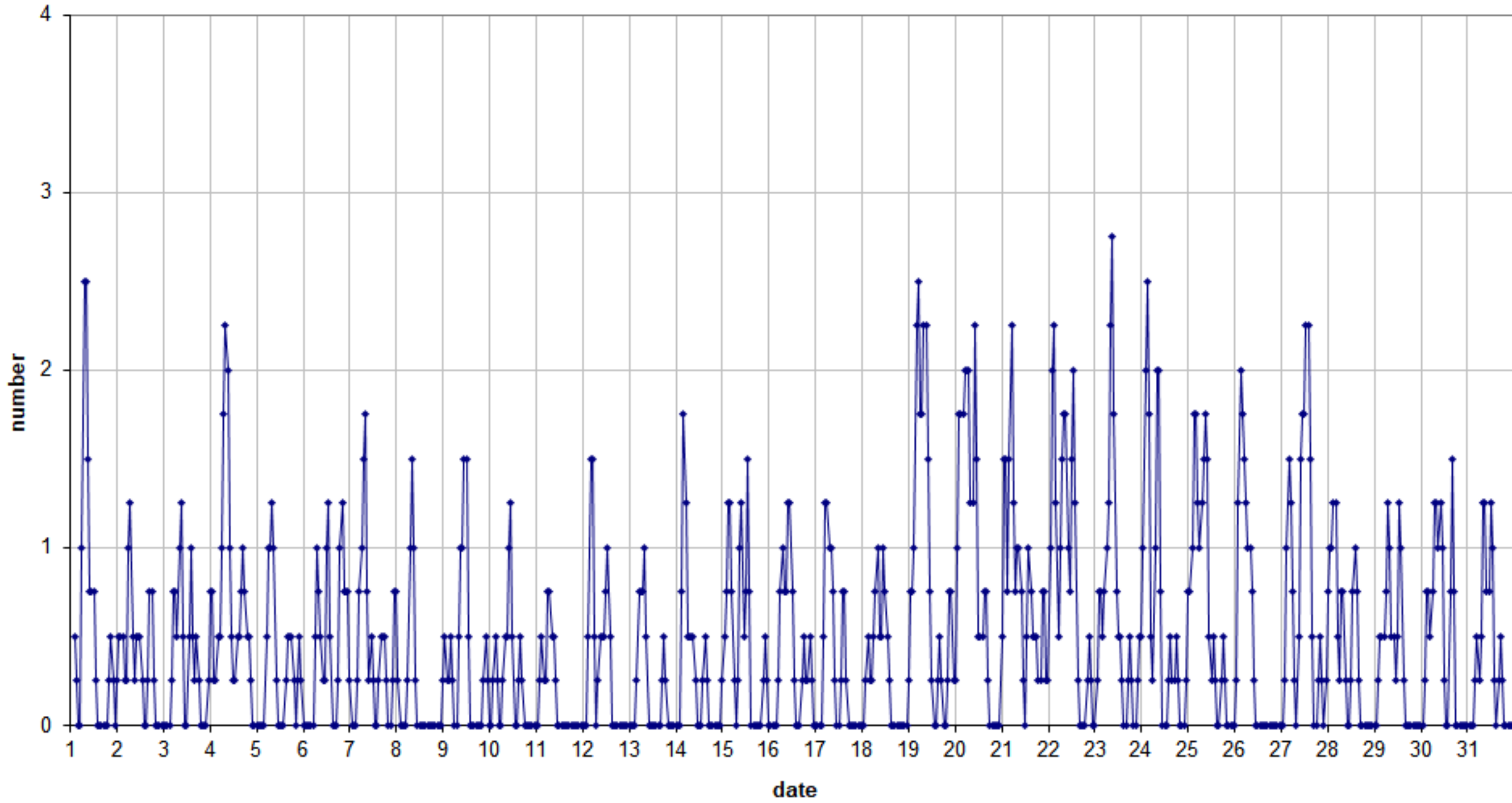
49.99MHz - RadioMeteors October 2023 number of reflections >10 seconds per hour (weighted average) Felix Verbelen (Kampanhout)
