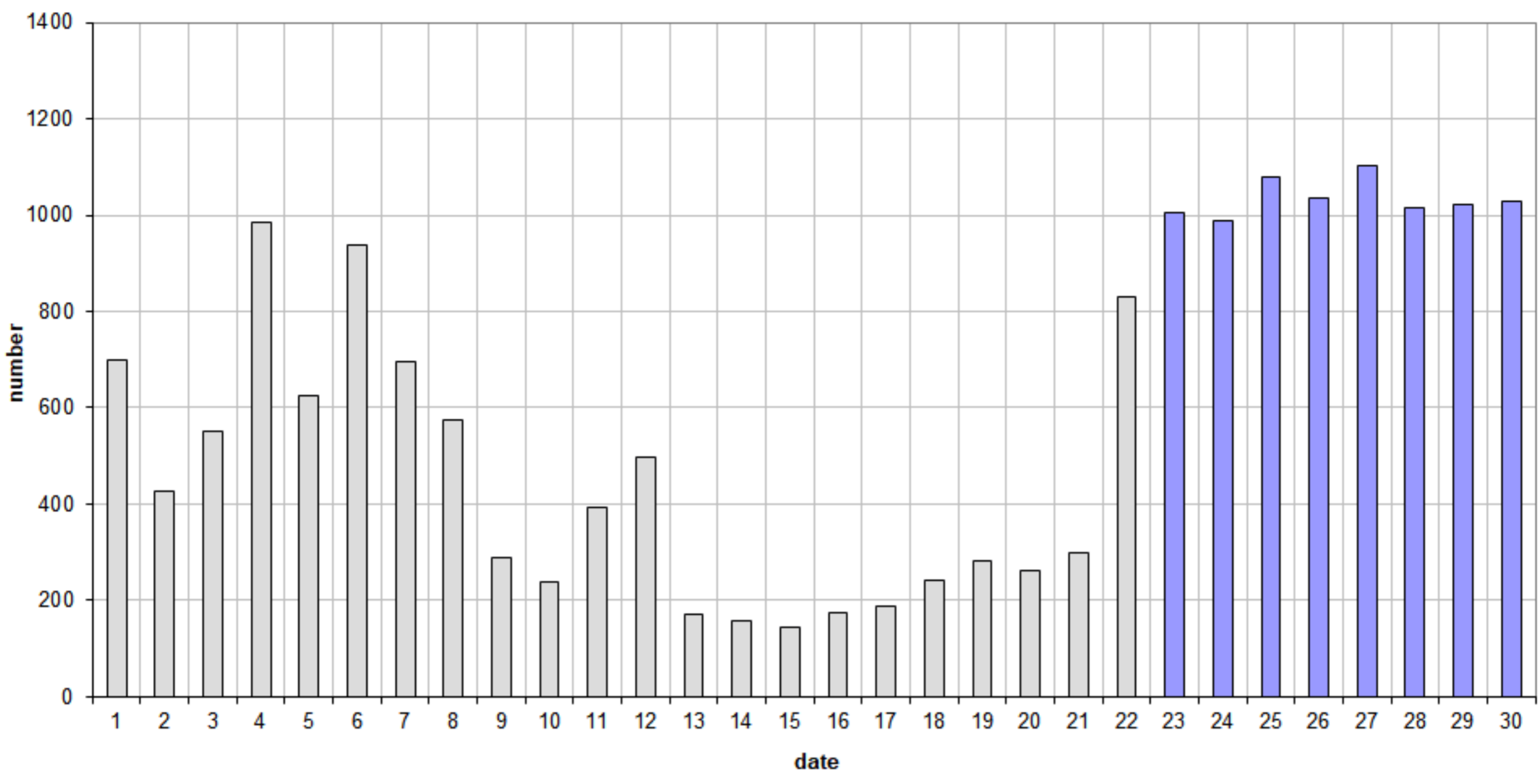
49.99MHz - RadioMeteors November 2023 daily totals of "all" reflections (automatic count_Mettel5_7Hz) Felix Verbelen (Kamphenhout)
