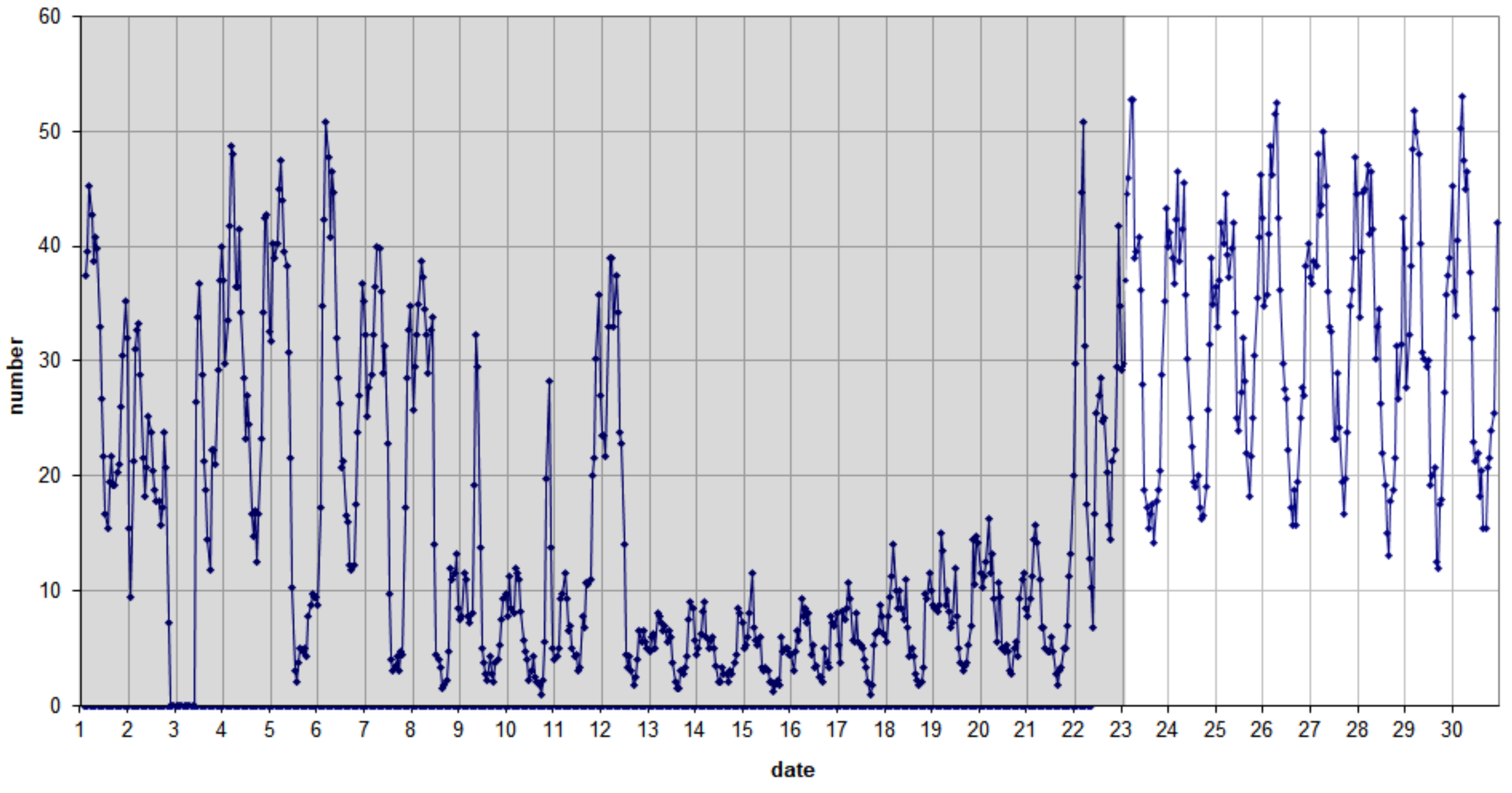
49.99 MHz - RadioMeteors November 2023 number of "all" reflections per hour (weighted average) (automatic count_MetteI5_7Hz) Felix Verbelen (Kampenhout)
