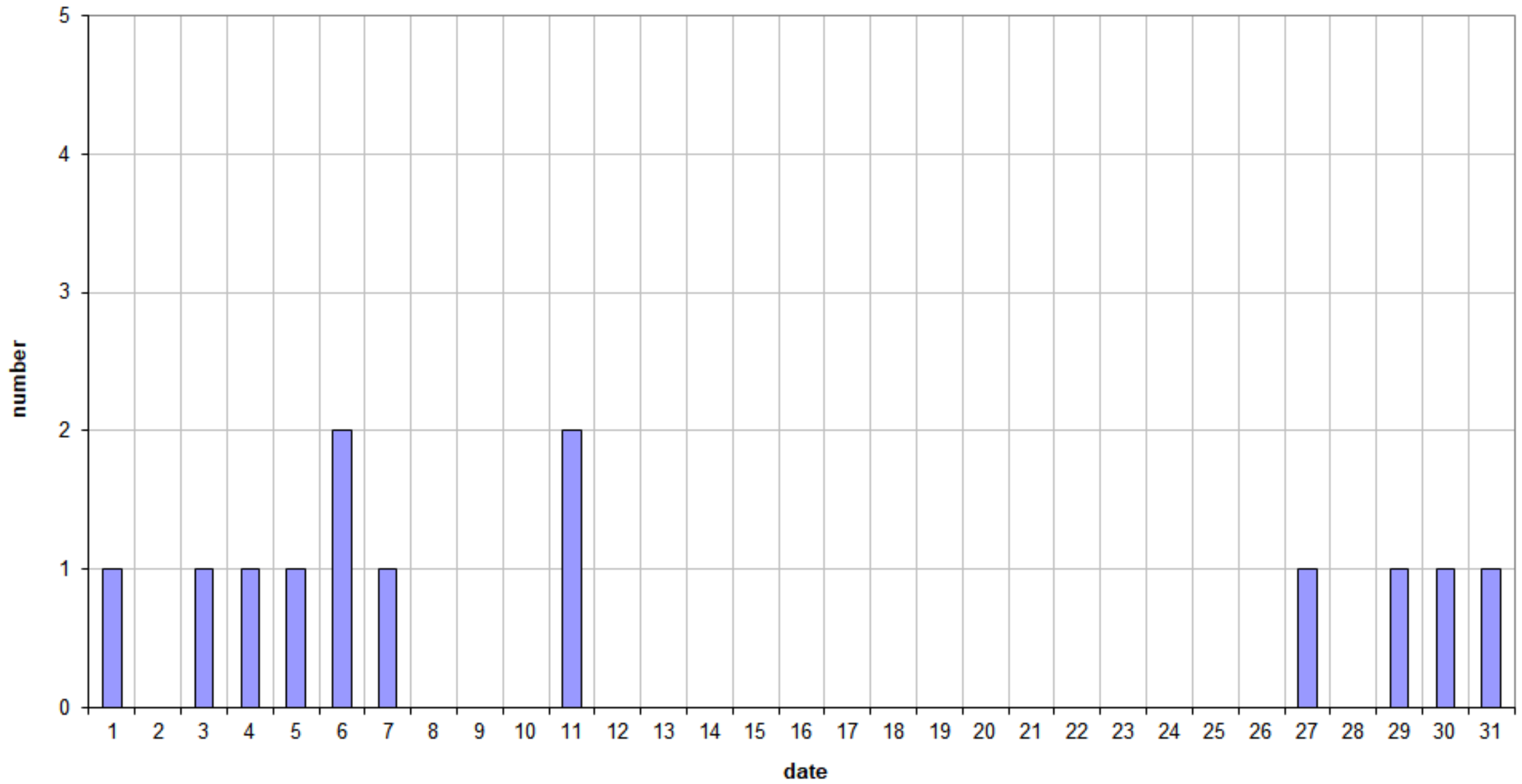
49.99MHz - RadioMeteors December 2023 daily totals of reflections longer than 1 minute Felix Verbelen (Kamphenhout)
