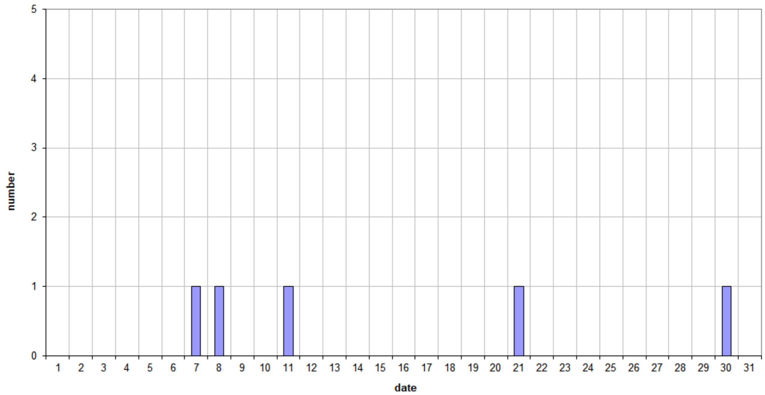
49.99MHz - RadioMeteors January 2024 daily totals of reflections longer than 1 minute Felix Verbelen (Kamphenhout)
