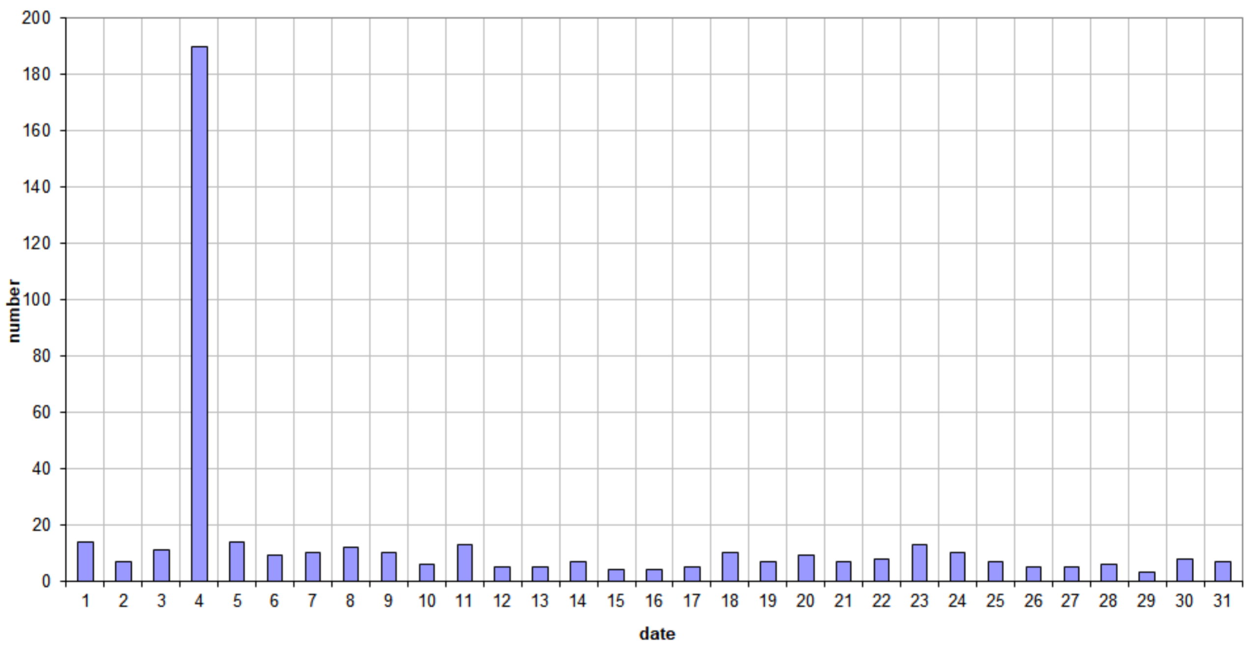
49.99MHz - RadioMeteors January 2024 daily totals of reflections longer than 10 seconds Felix Verbelen (Kamphenhout)
