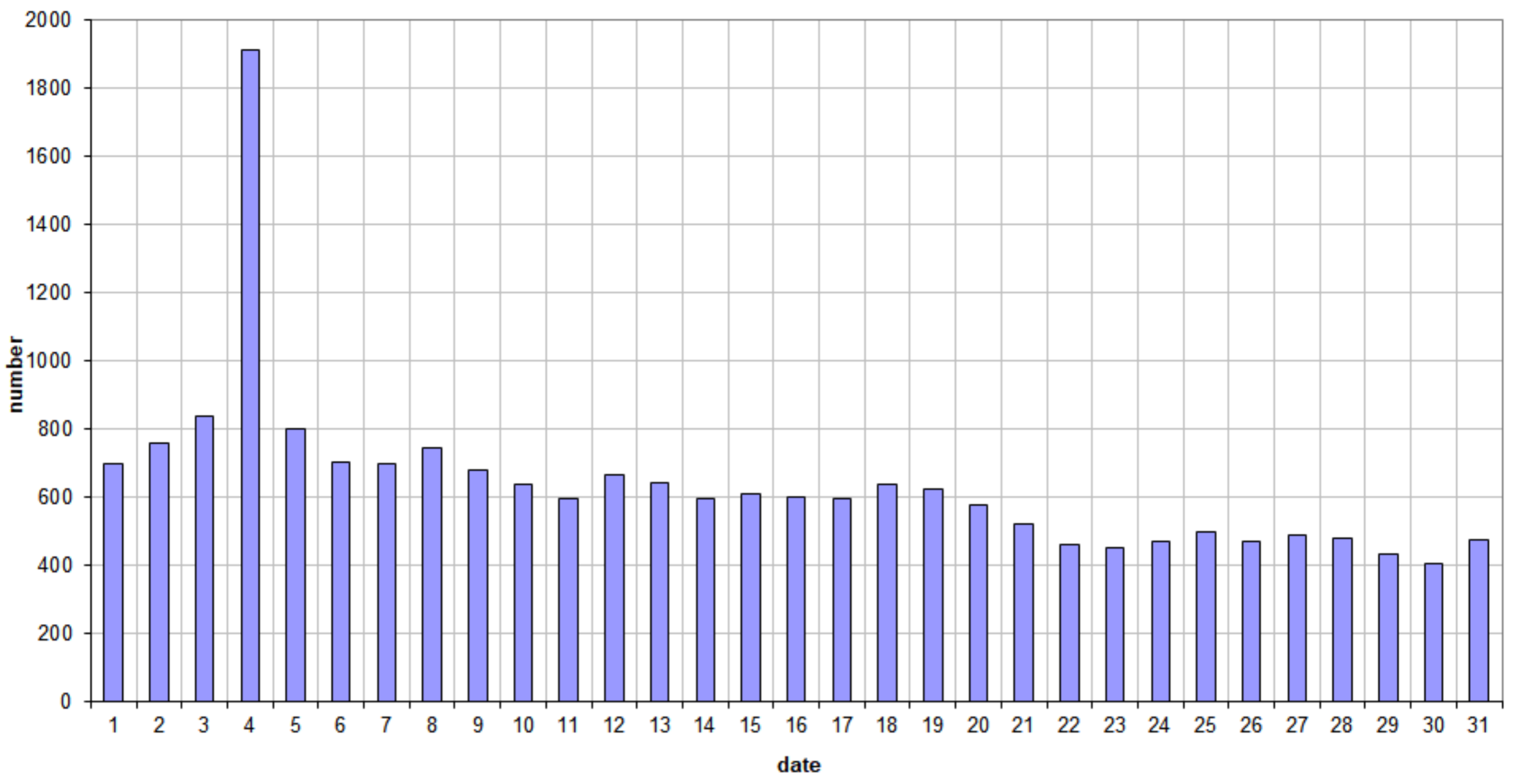
49.99MHz - RadioMeteors January 2024 daily totals of "all" reflections (automatic count_Mettel5_7Hz) Felix Verbelen (Kamphenhout)
