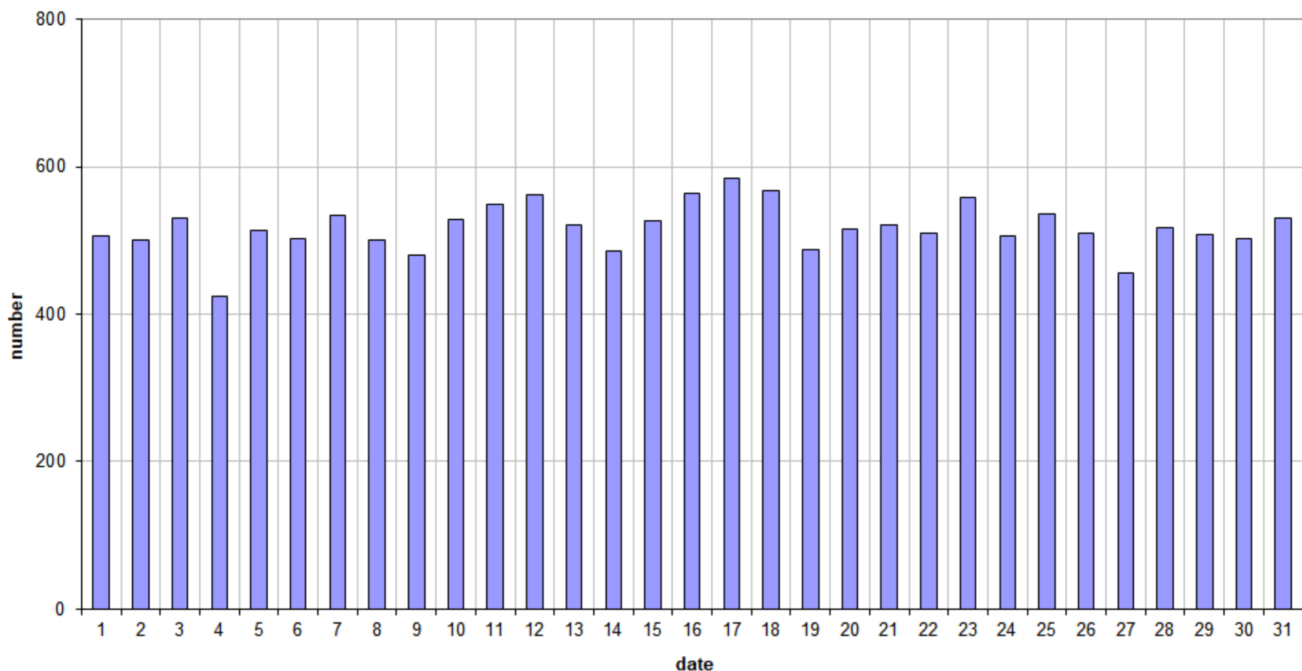
49.99MHz - RadioMeteors March 2024 daily totals of "all" reflections (automatic count_Mettel5_7Hz)
