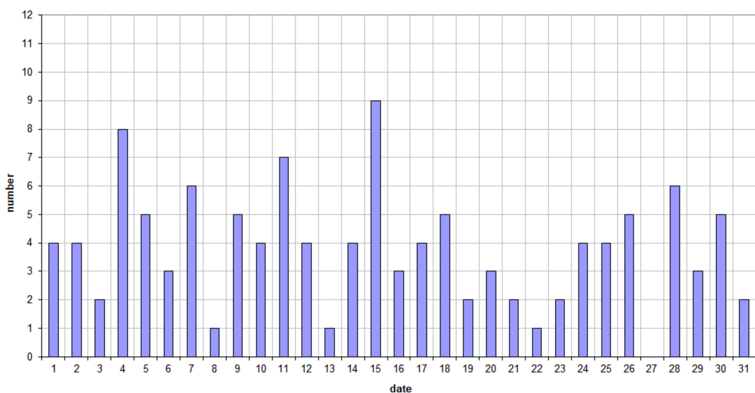
49.99MHz - RadioMeteors March 2024 daily totals of reflections longer than 10 seconds
