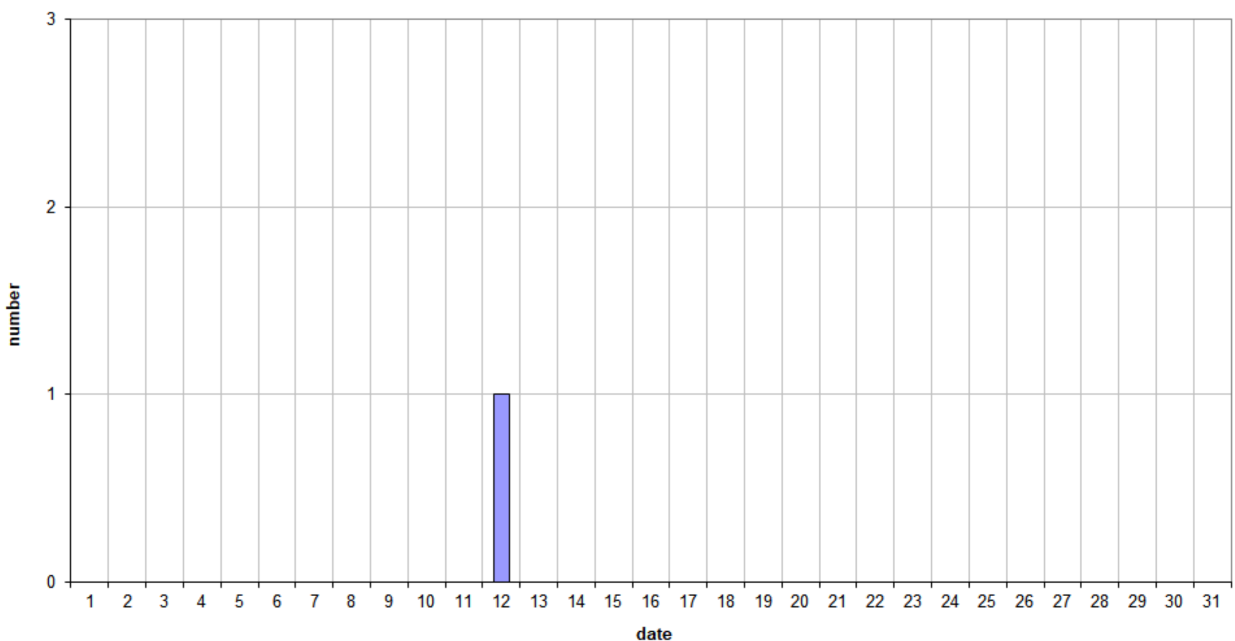
49.99MHz - RadioMeteors March 2024 daily totals of reflections longer than 1 minute
