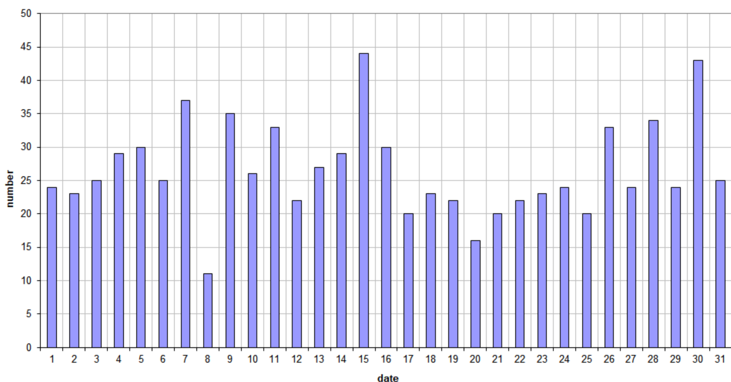
49.99MHz - RadioMeteors March 2024 daily totals of all overdense reflections
