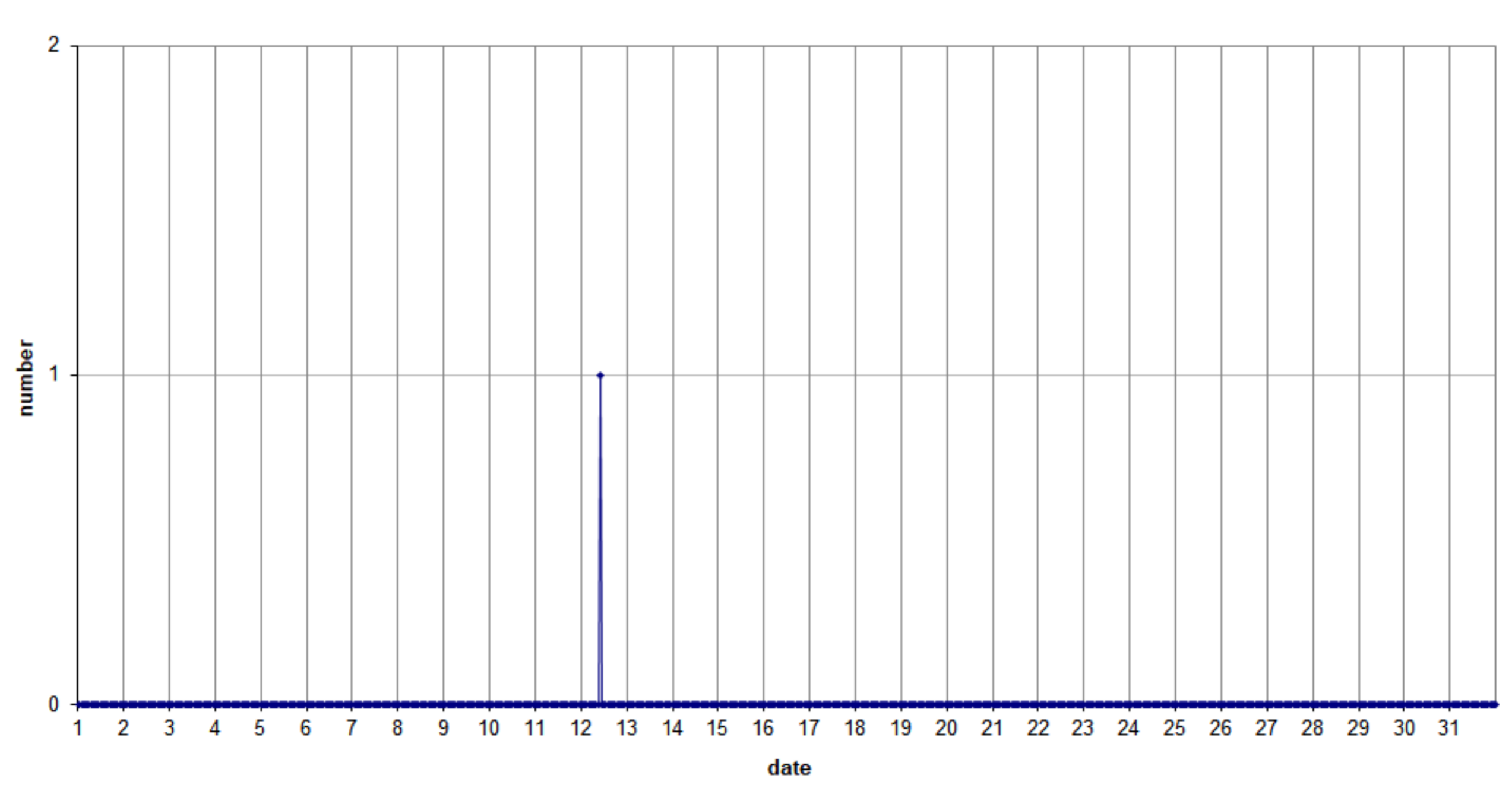
49.99MHz - RadioMeteors March 2024 hourly totals of overdense reflections longer than 1 minute Felix Verbelen (Kamphenhout/BE)
