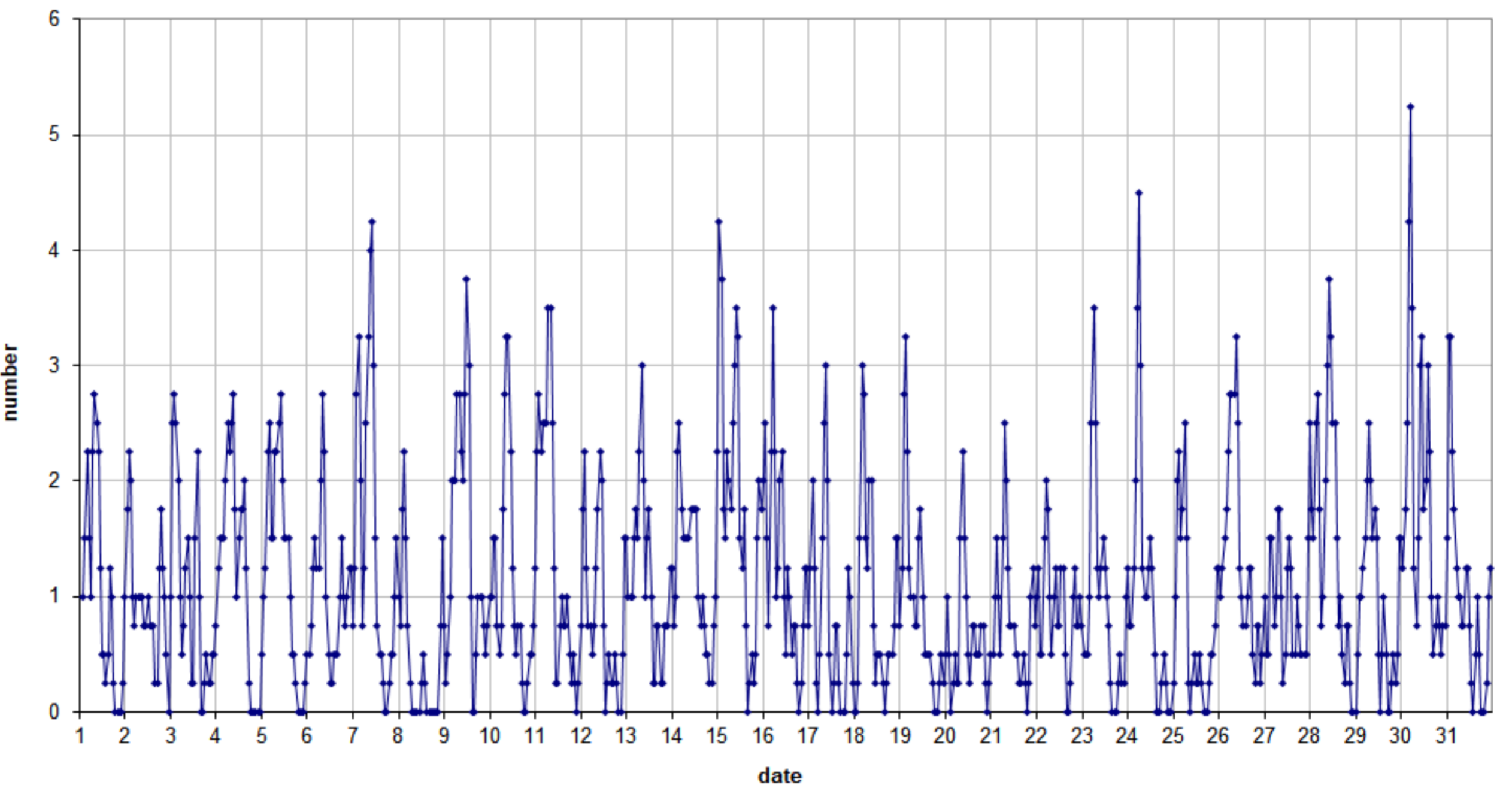
49.99MHz - RadioMeteors March 2024 number of overdense reflections per hour (weighted average) Felix Verbelen (Kamphenhout)
