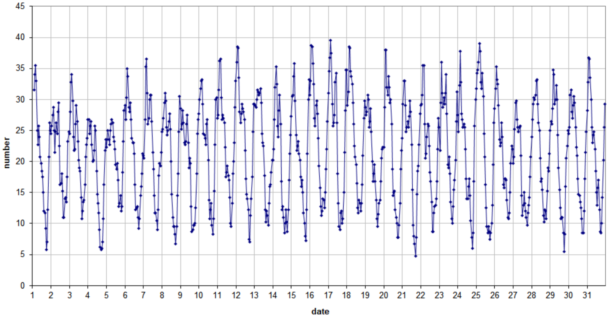
49.99 MHz - RadioMeteors March 2024 number of "all" reflections per hour (weighted average) (automatic count_Mettel5_7Hz) Felix Verbelen (Kamphenhout)
