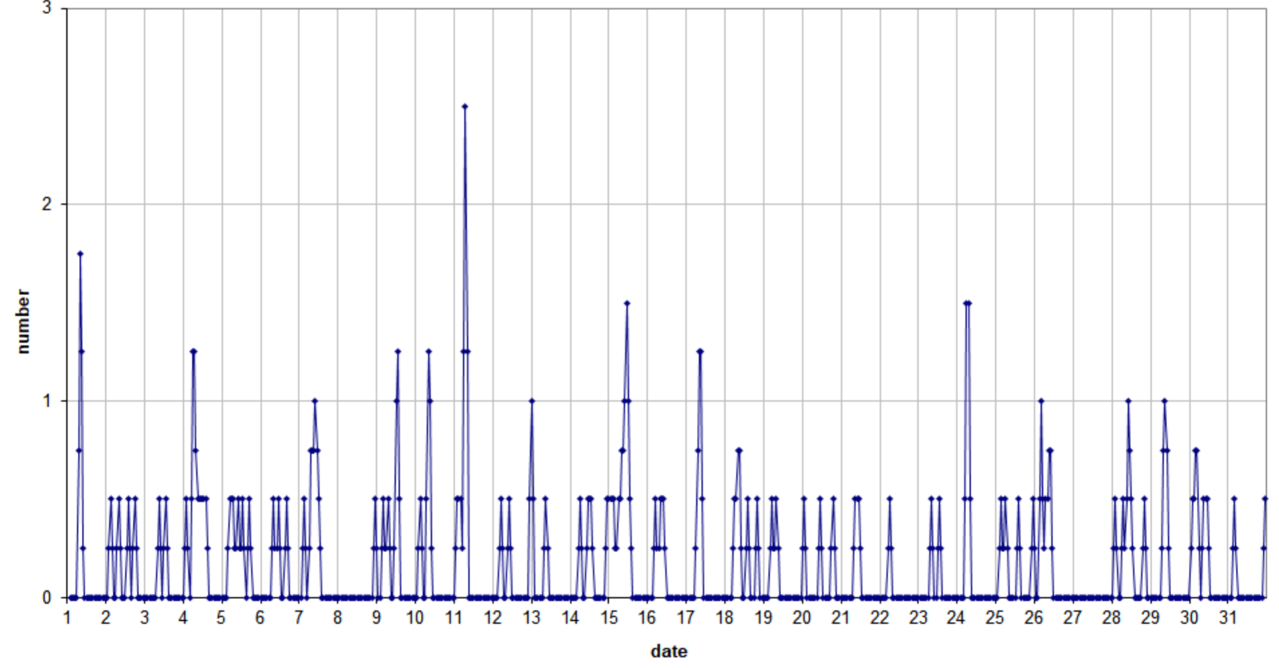
49.99MHz - RadioMeteors March 2024 number of reflections >10 seconds per hour (weighted average) Felix Verbelen (Kamphenhout)
