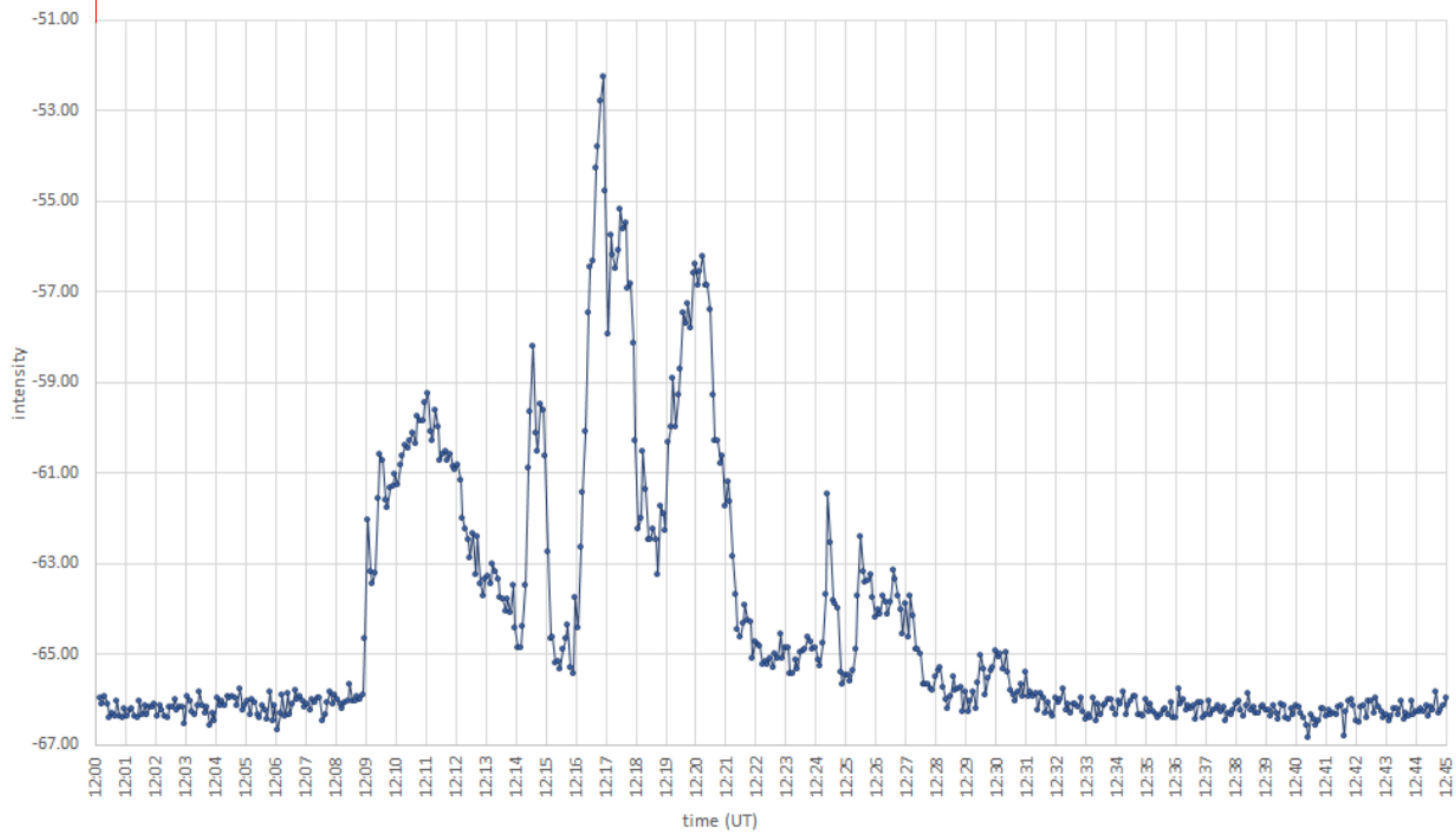
20240310_12:00-12:45 UT_49.99 MHz_noise raw data average per 5 seconds Felix Verbelen (Kamphenhout/Belgium)
