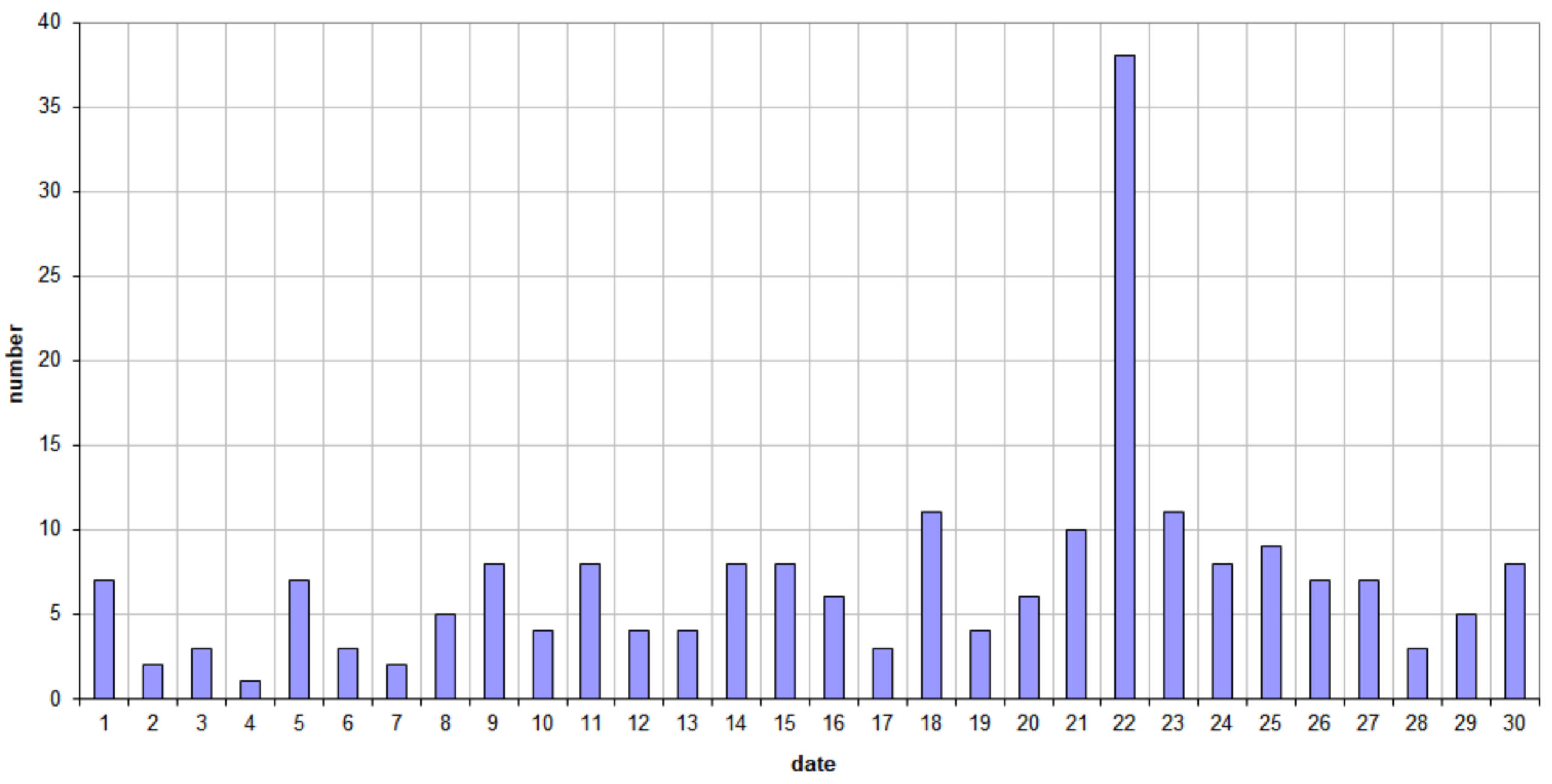
49.99MHz - RadioMeteors April 2024 daily totals of reflections longer than 10 seconds Felix Verbelen (Kampenhout)
