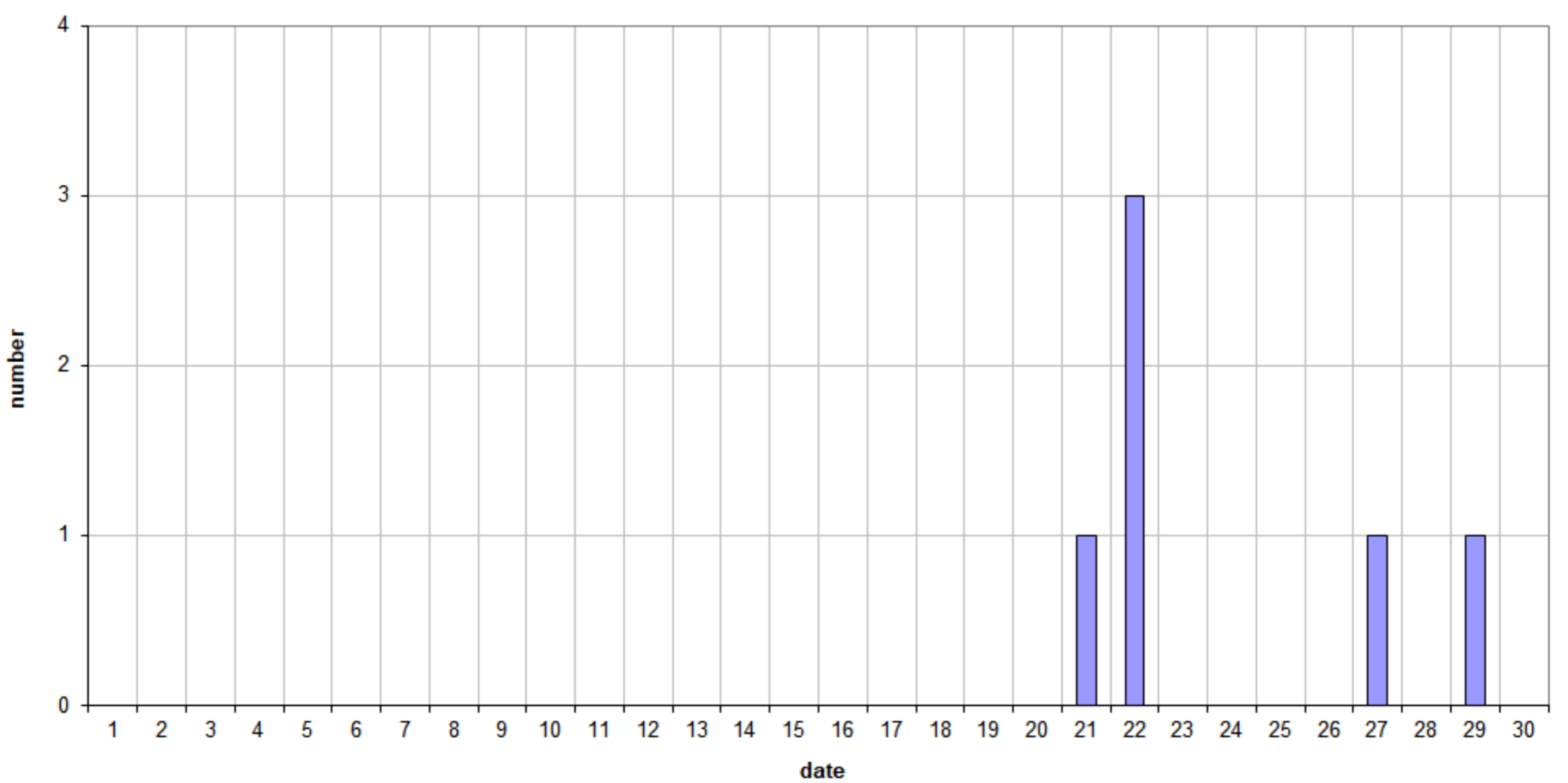
49.99MHz - RadioMeteors April 2024 daily totals of reflections longer than 1 minute Felix Verbelen (Kampenhout)
