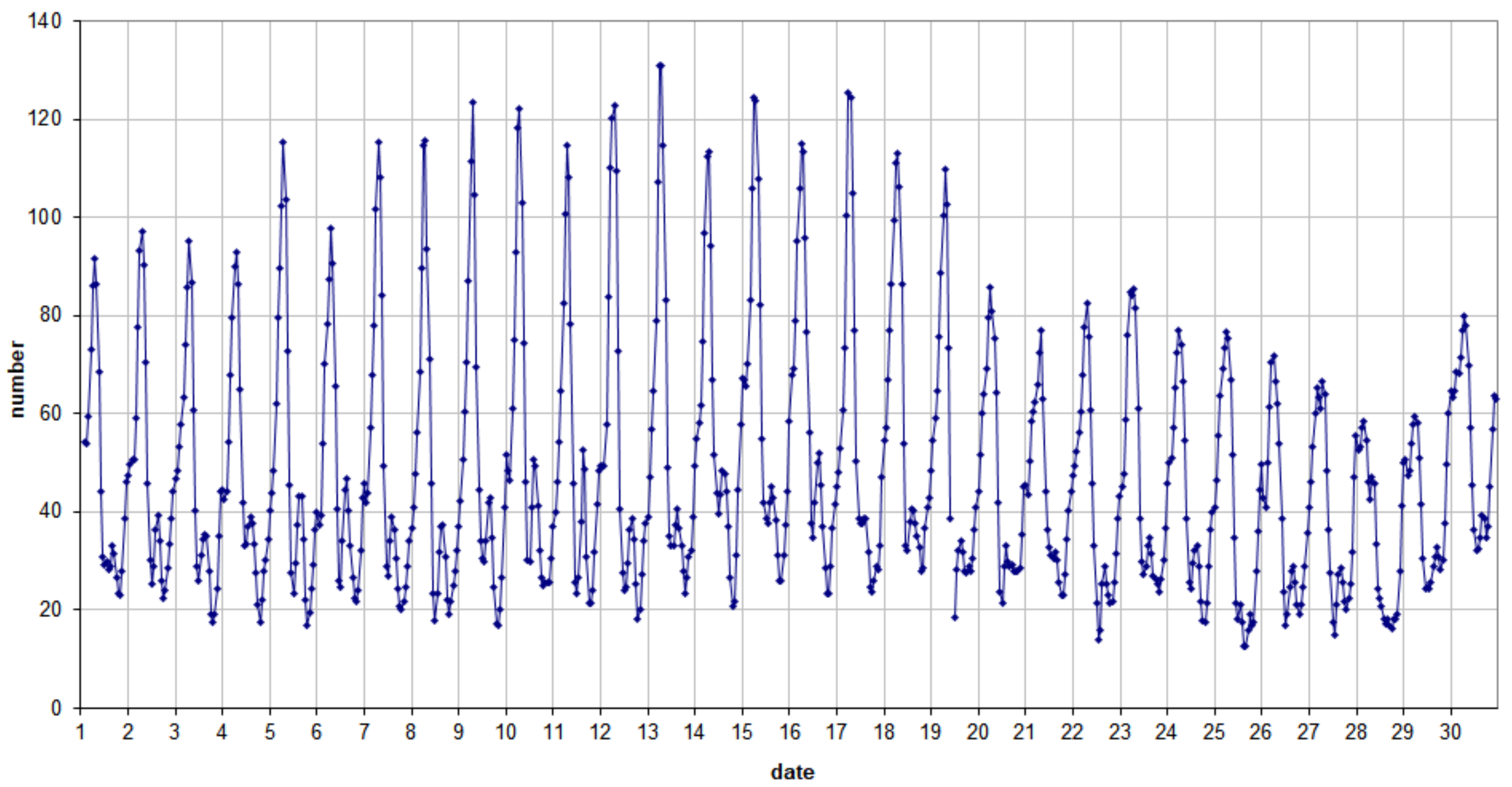
49.99 MHz - RadioMeteors June 2024 number of "all" reflections per hour (weighted average) (automatic count_Mettel5_7Hz) Felix Verbelen (Kamphenhout)
