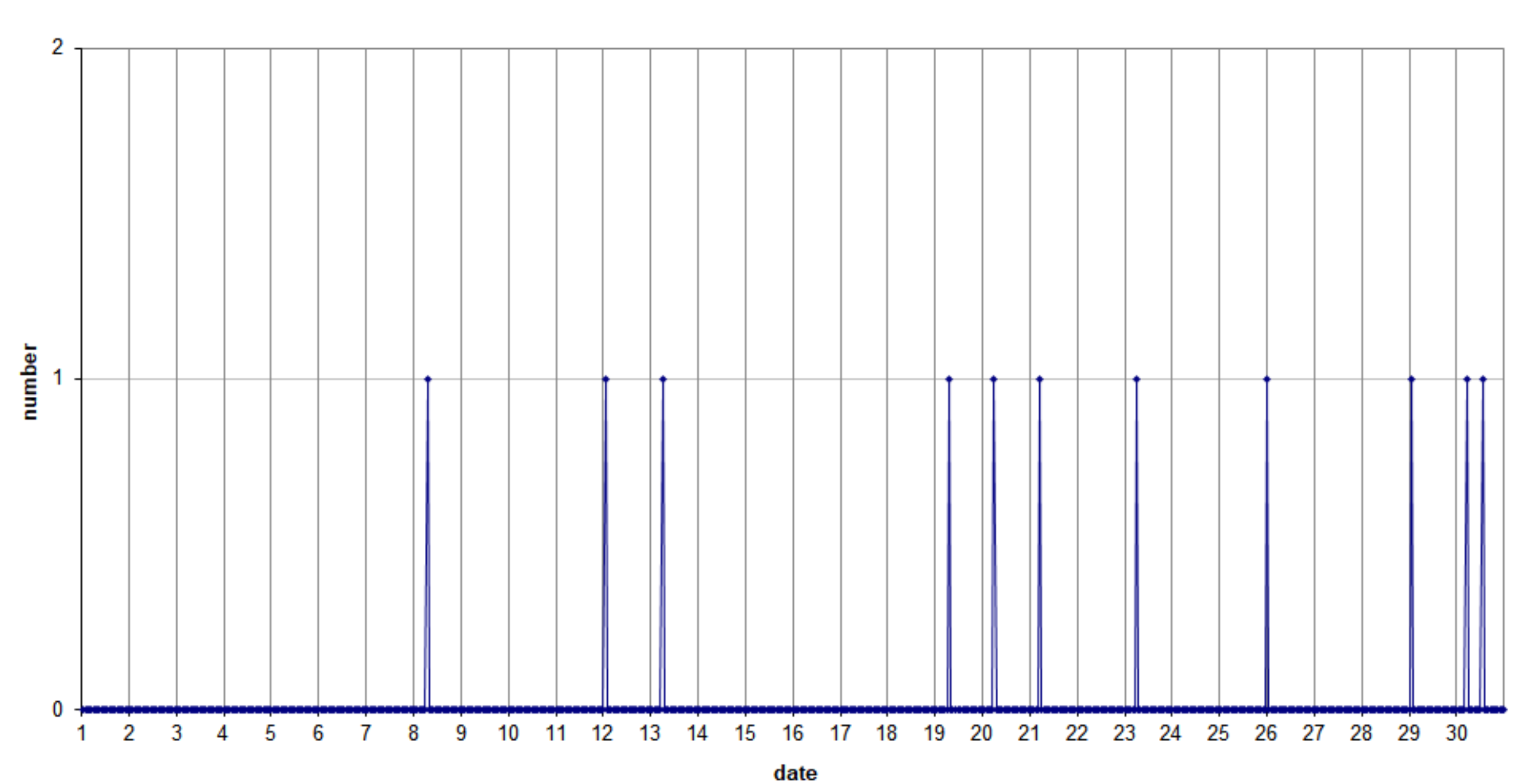
49.99MHz - RadioMeteors June 2024 hourly totals of overdense reflections longer than 1 minute Felix Verbelen (Kamphenhout/BE)
