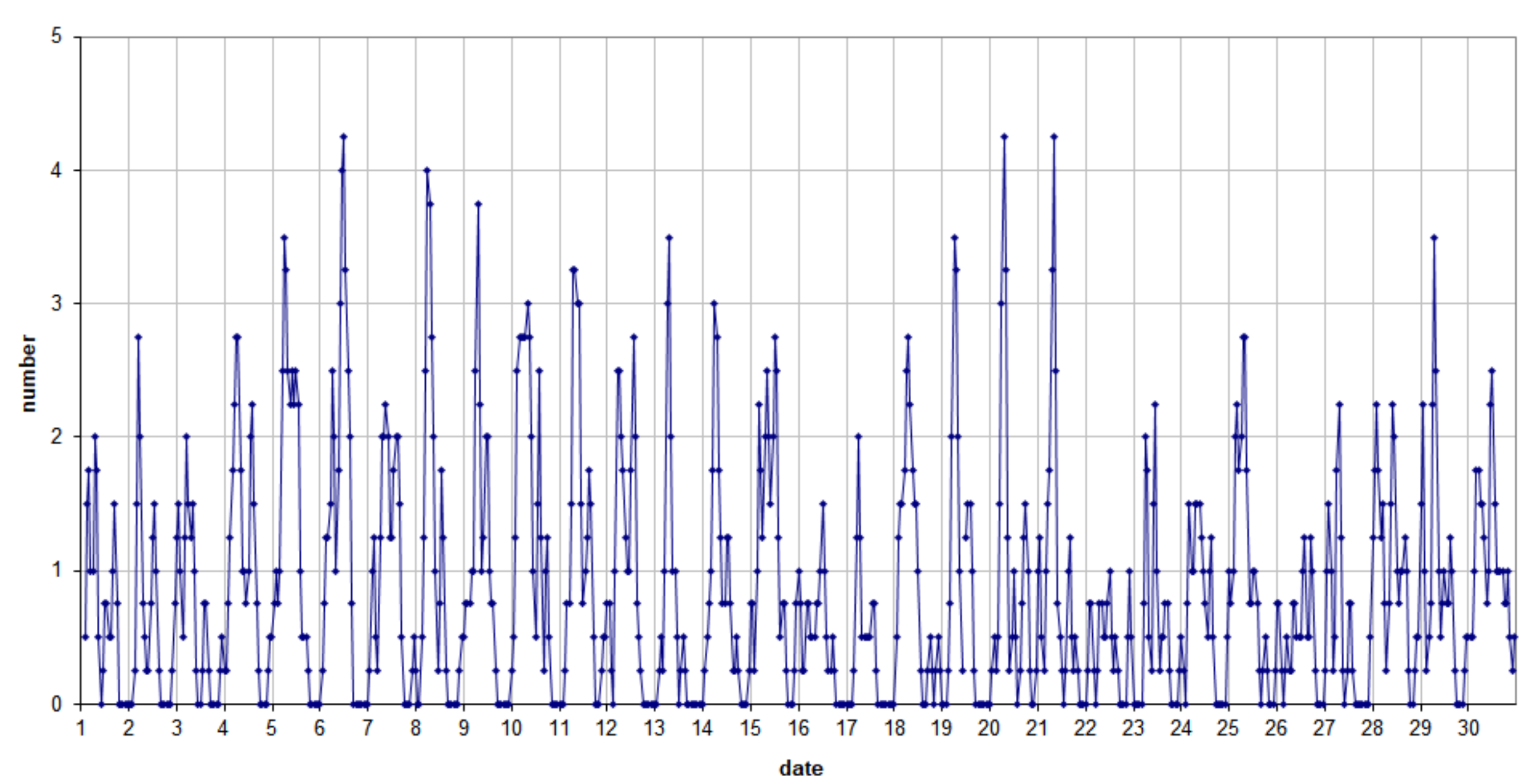
49.99MHz - RadioMeteors June 2024 number of reflections >10 seconds per hour (weighted average) Felix Verbelen (Kamphenhout)
