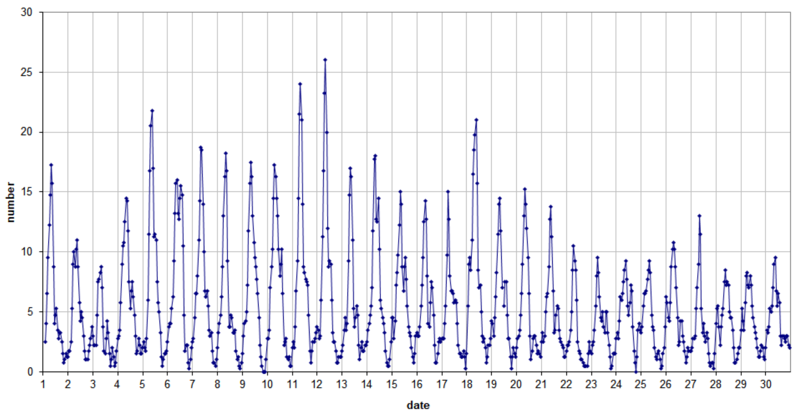
49.99MHz - RadioMeteors June 2024 number of overdense reflections per hour (weighted average) Felix Verbelen (Kamphenhout)
