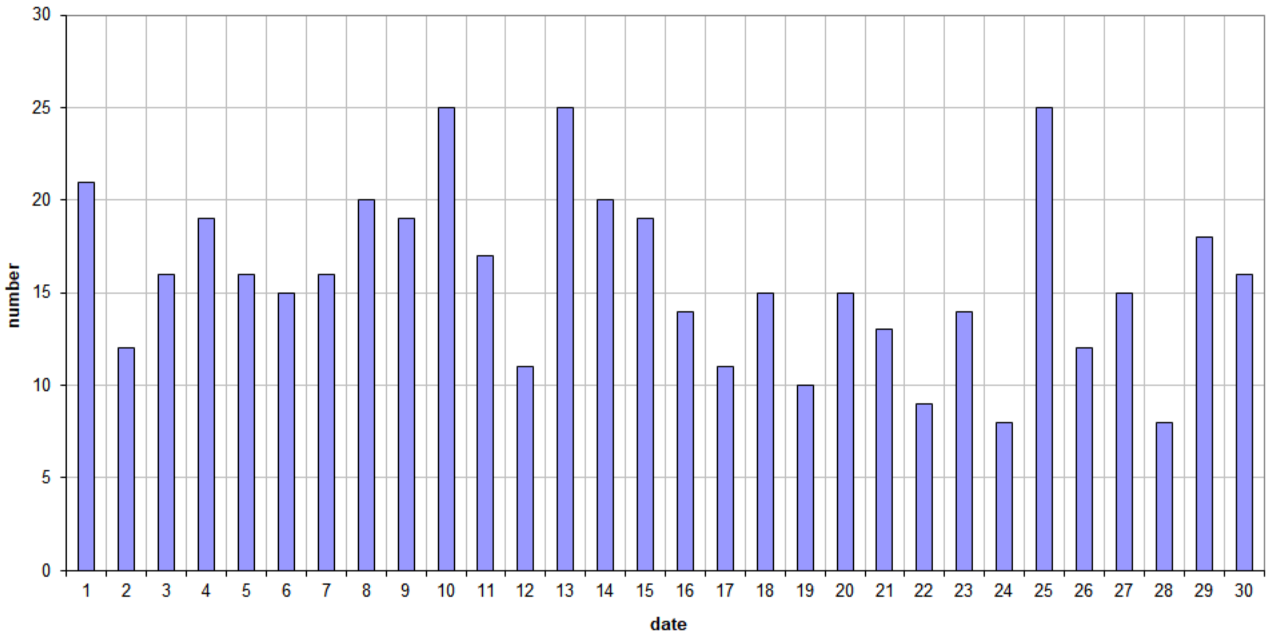
49.99MHz - RadioMeteors September 2024 daily totals of reflections longer than 10 seconds Felix Verbelen (Kampenhout)
