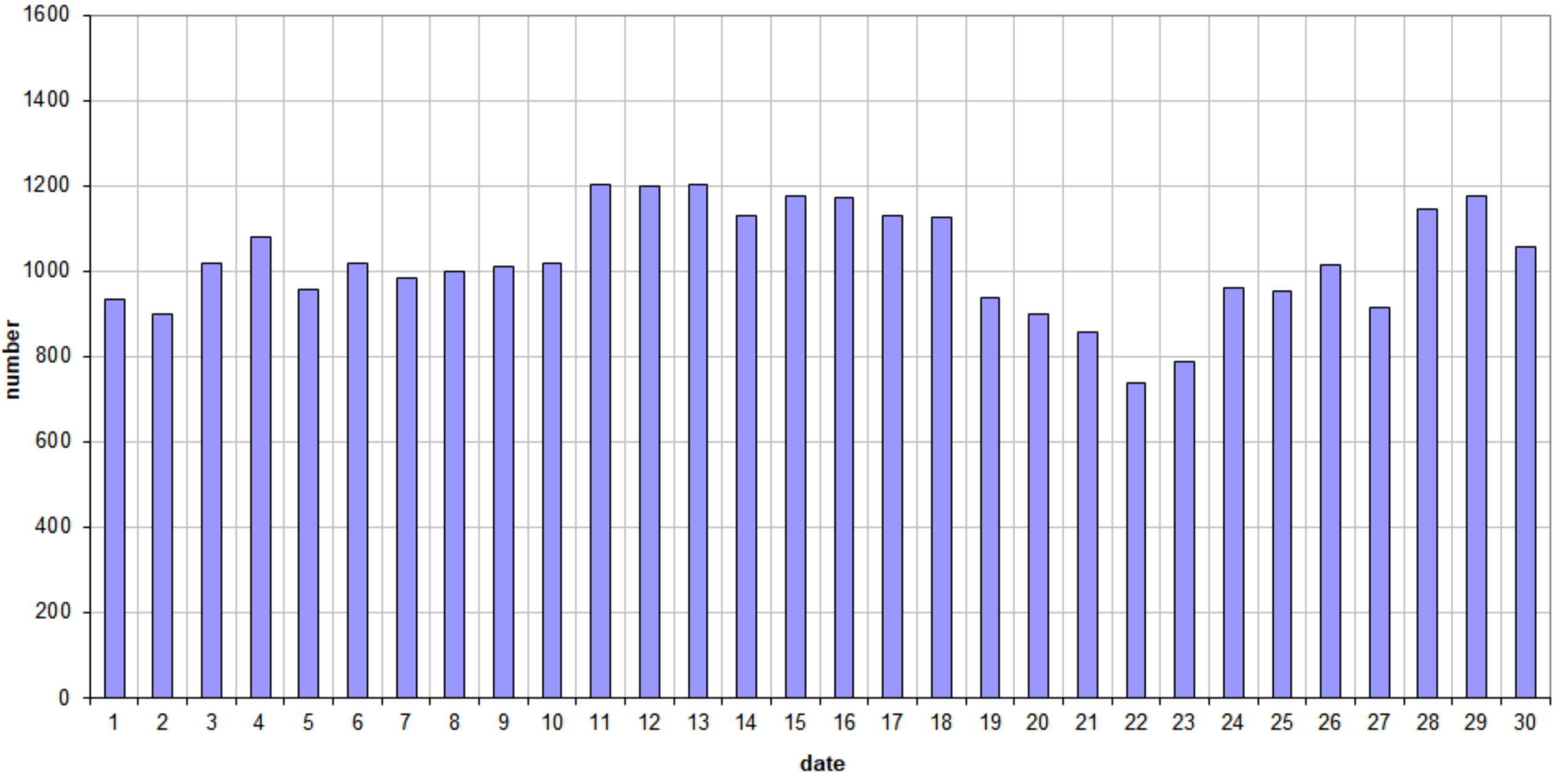
49.99MHz - RadioMeteors September 2024 daily totals of "all" reflections (automatic count_Mettel5_7Hz) Felix Verbelen (Kampenhout)
