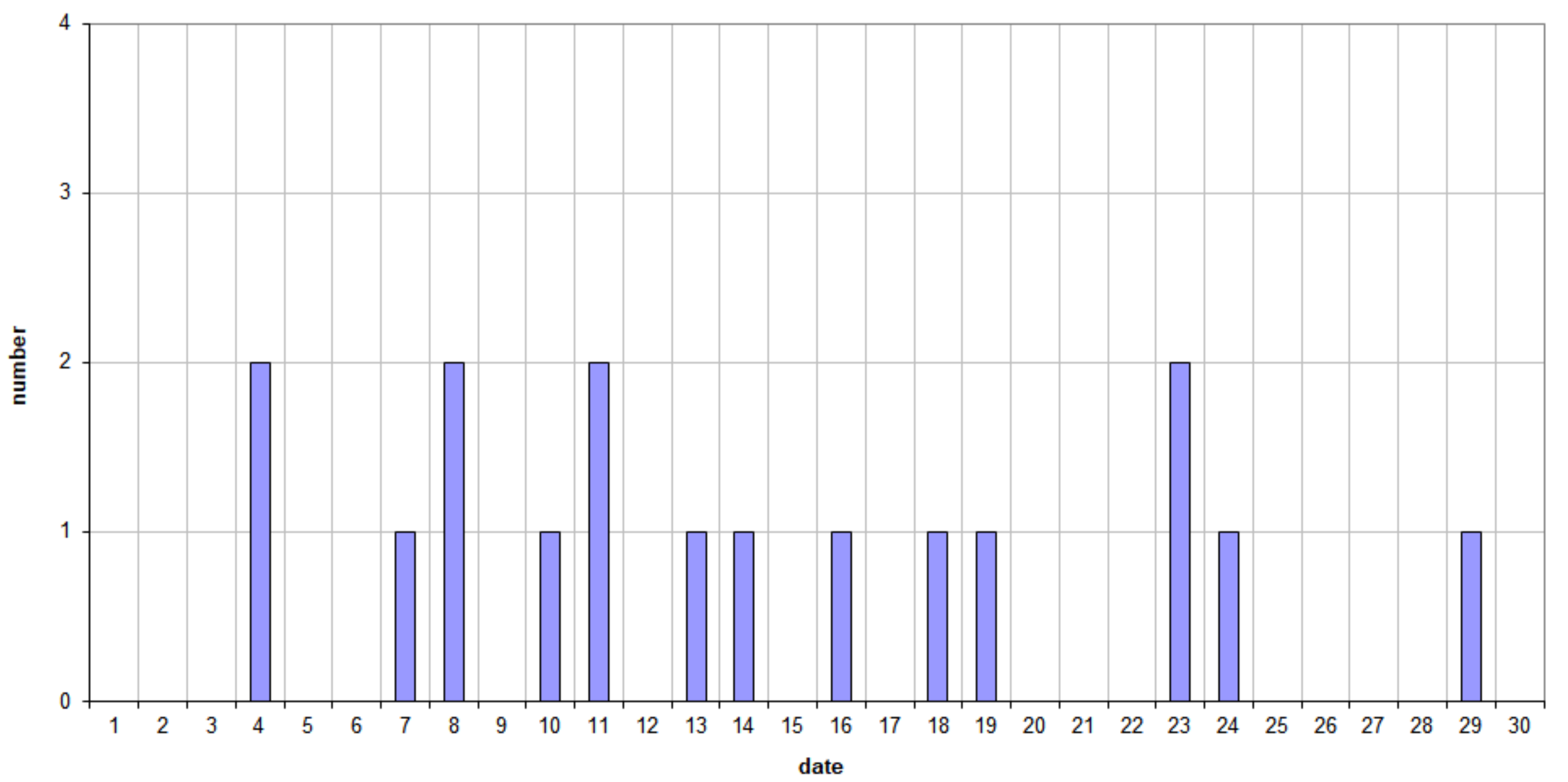
49.99MHz - RadioMeteors September 2024 daily totals of reflections longer than 1 minute Felix Verbelen (Kampenhout)
