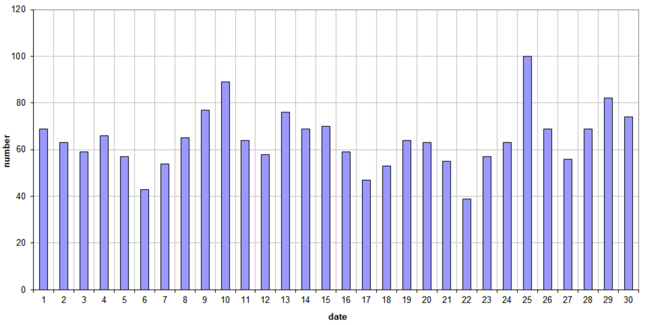
49.99MHz - RadioMeteors September 2024 daily totals of all overdense reflections Felix Verbelen (Kampenhout)
