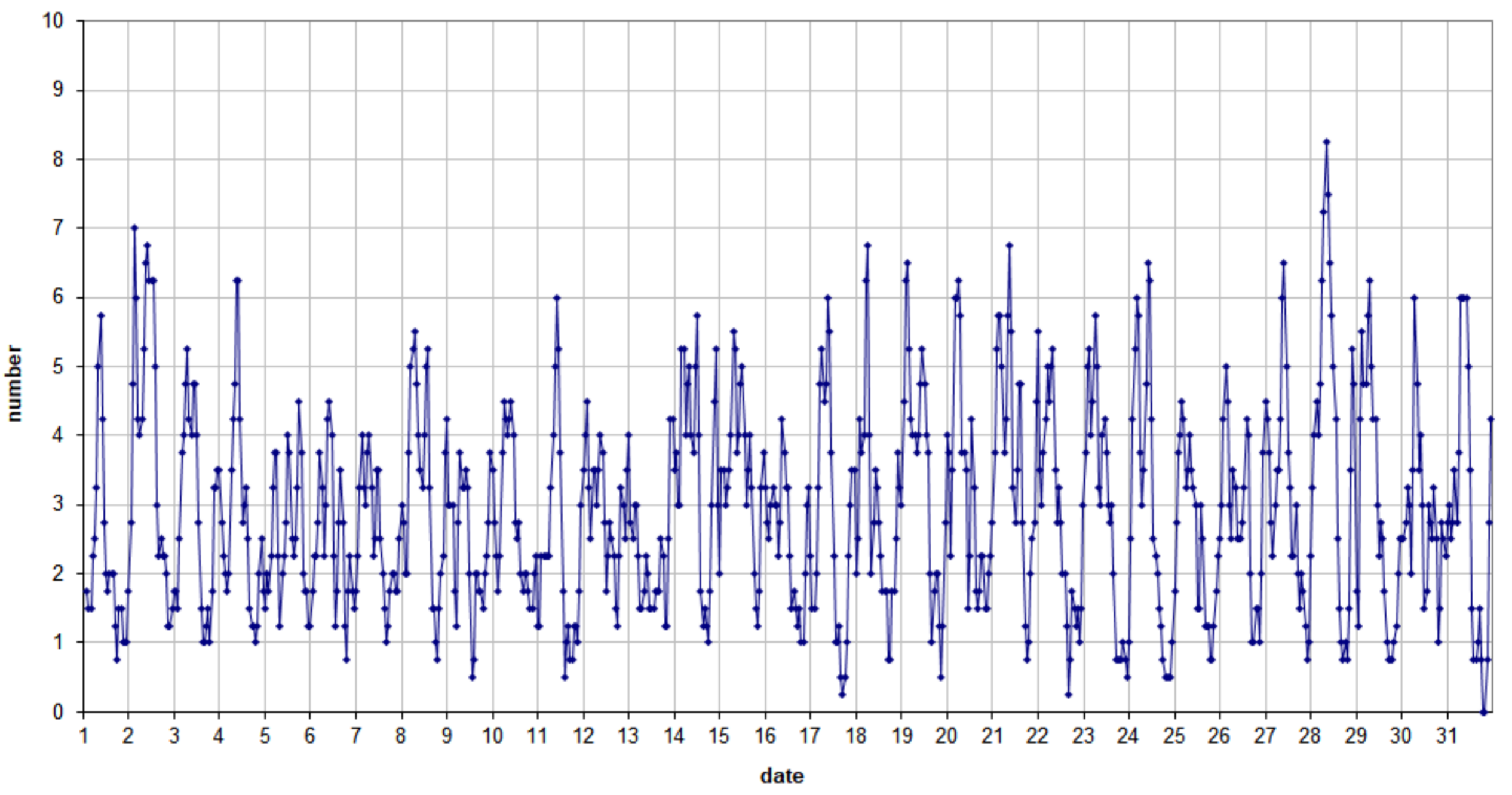
49.99MHz - RadioMeteors October 2024 number of overdense reflections per hour (weighted average) Felix Verbelen (Kamphenhout)
