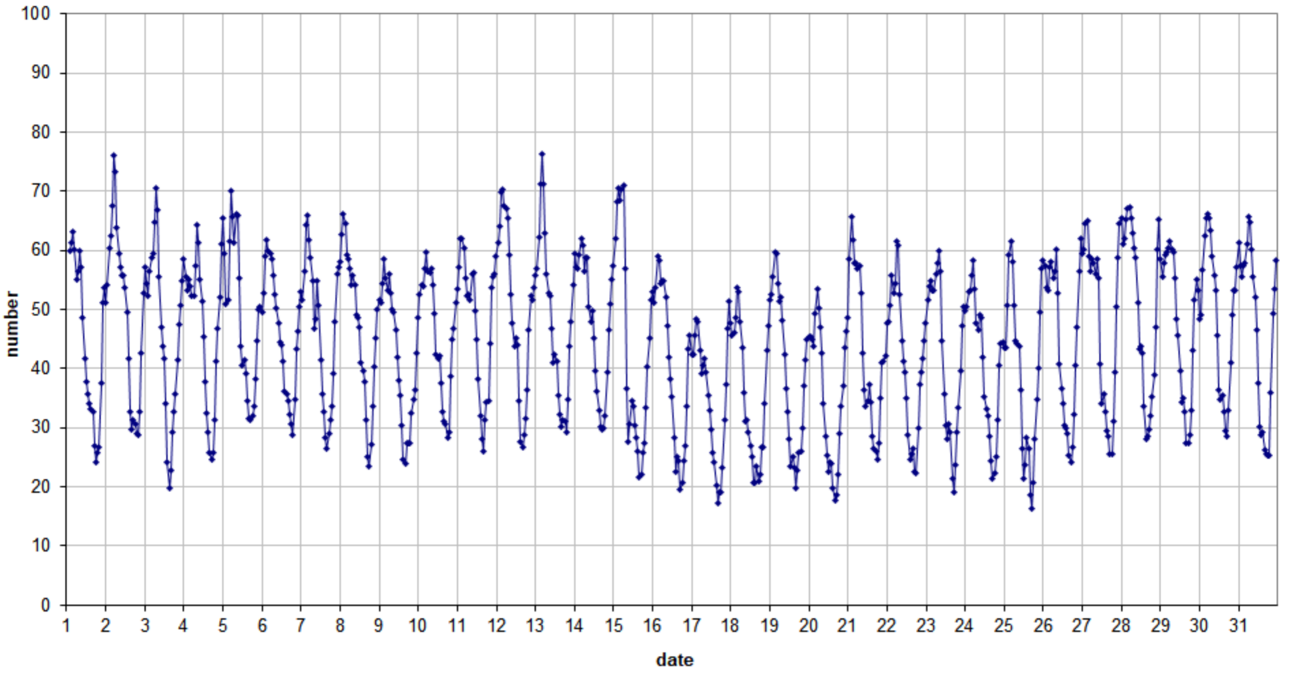
49.99 MHz - RadioMeteors October 2024 number of "all" reflections per hour (weighted average) (automatic count_Mettel5_7Hz) Felix Verbelen (Kamphenhout)
