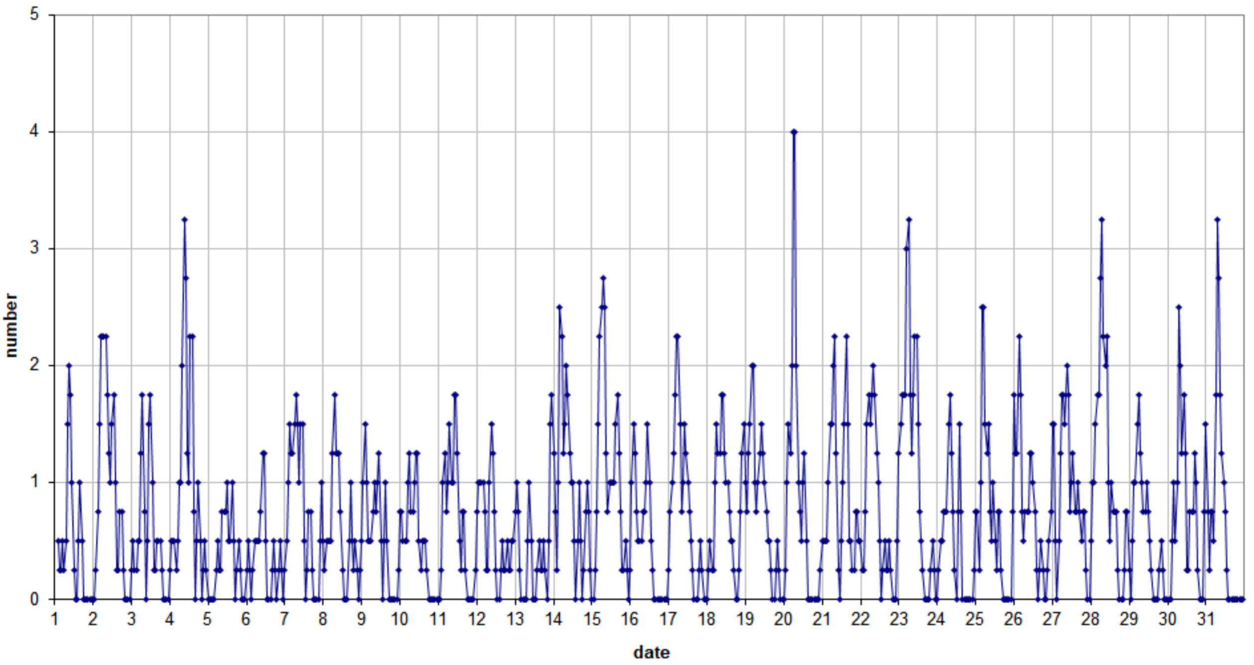
49.99MHz - RadioMeteors October 2024 number of reflections >10 seconds per hour (weighted average) Felix Verbelen (Kamphenhout)
