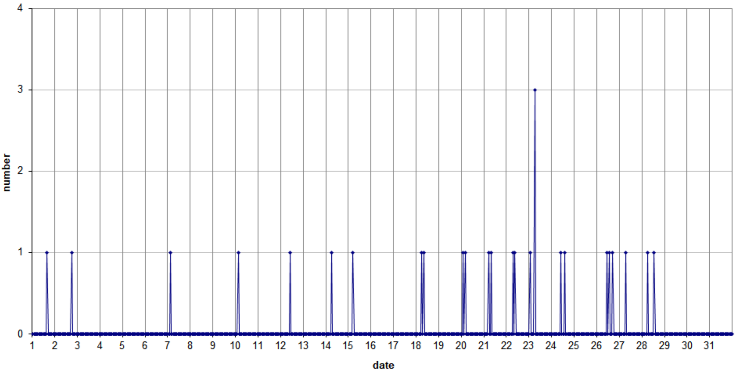
49.99MHz - RadioMeteors October 2024 hourly totals of overdense reflections longer than 1 minute Felix Verbelen (Kamphenhout/BE)
