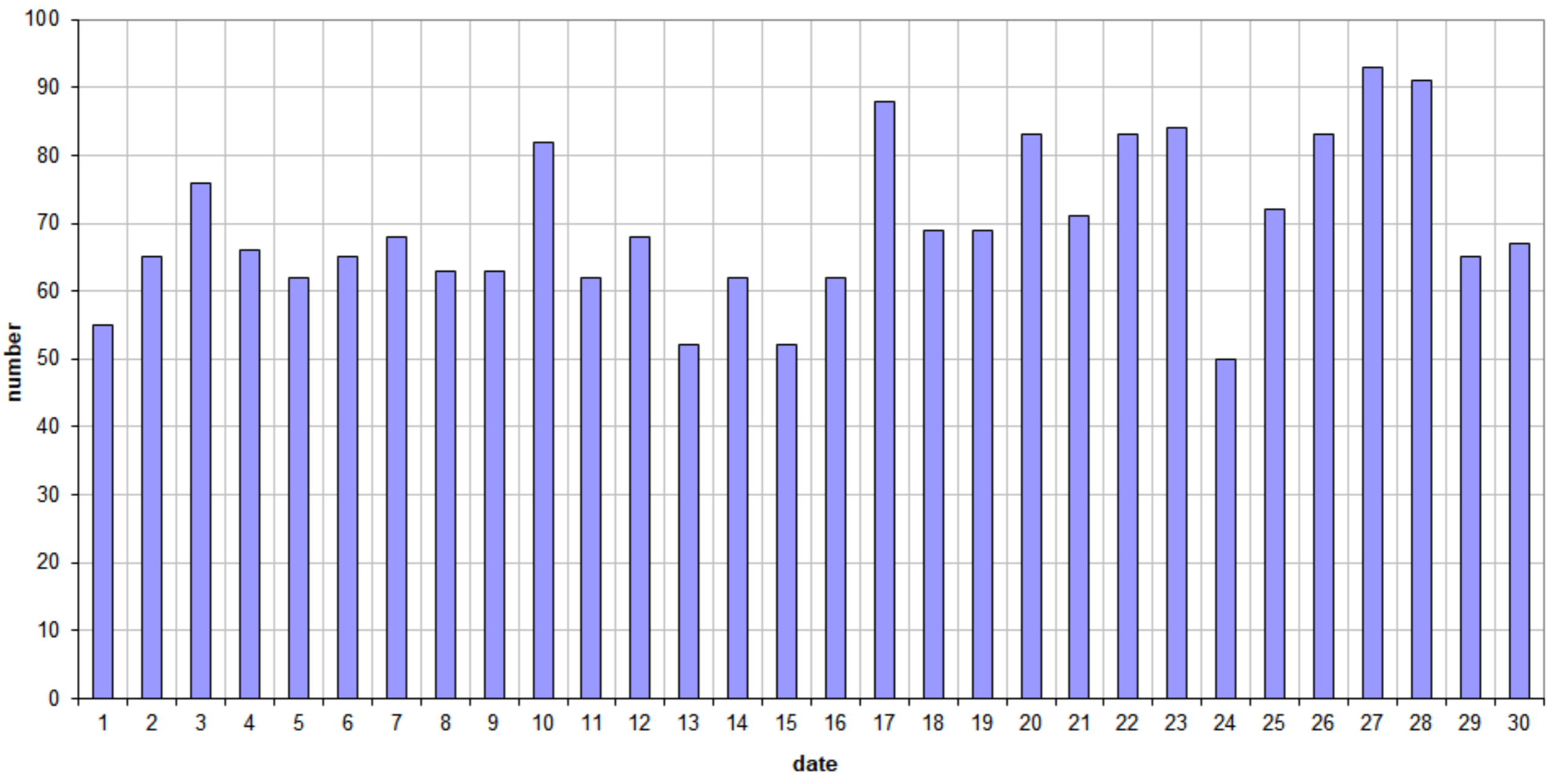
49.99MHz - RadioMeteors November 2024 daily totals of all overdense reflections Felix Verbelen (Kampenhout)
