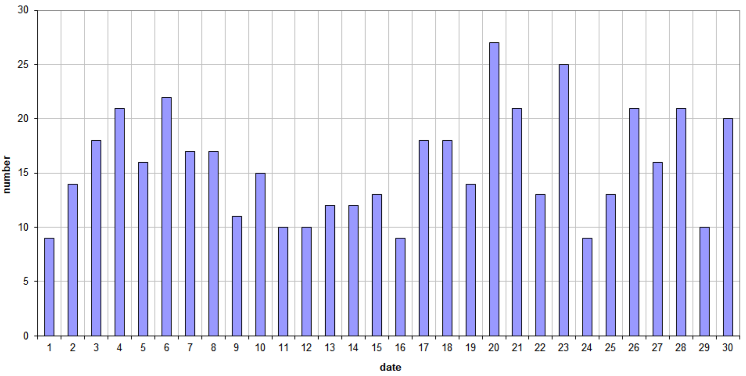
49.99MHz - RadioMeteors November 2024 daily totals of reflections longer than 10 seconds Felix Verbelen (Kampenhout)
