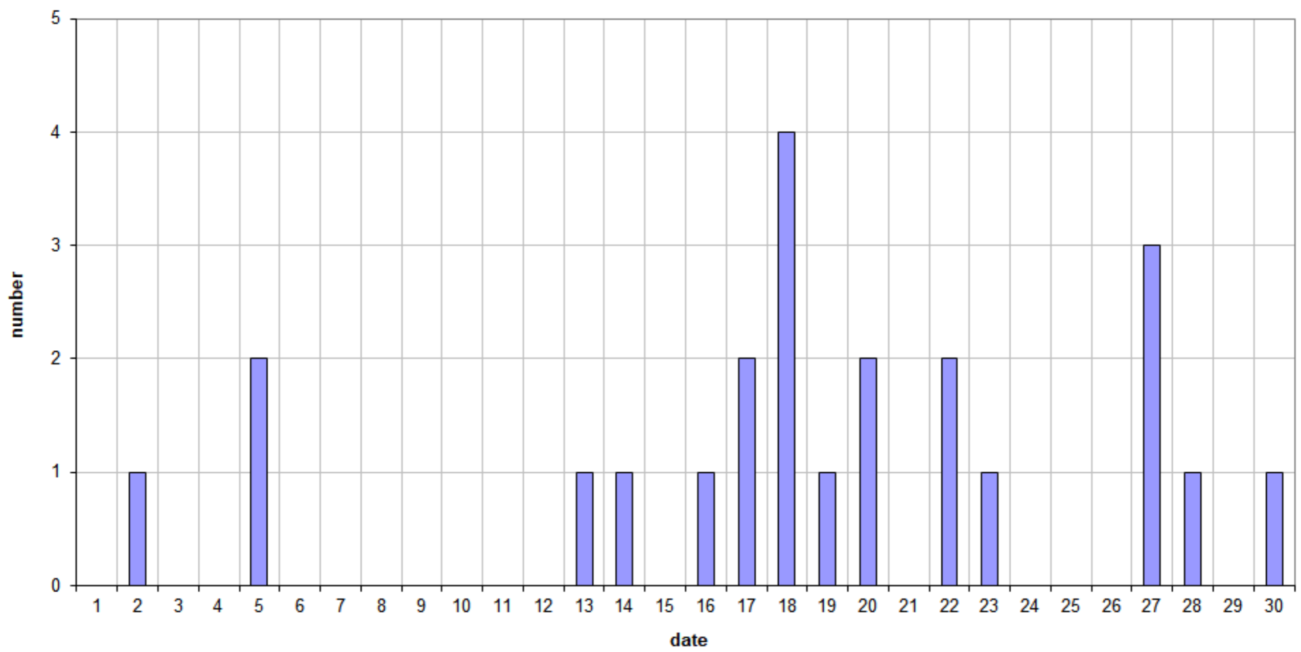
49.99MHz - RadioMeteors November 2024 daily totals of reflections longer than 1 minute Felix Verbelen (Kampenhout)
