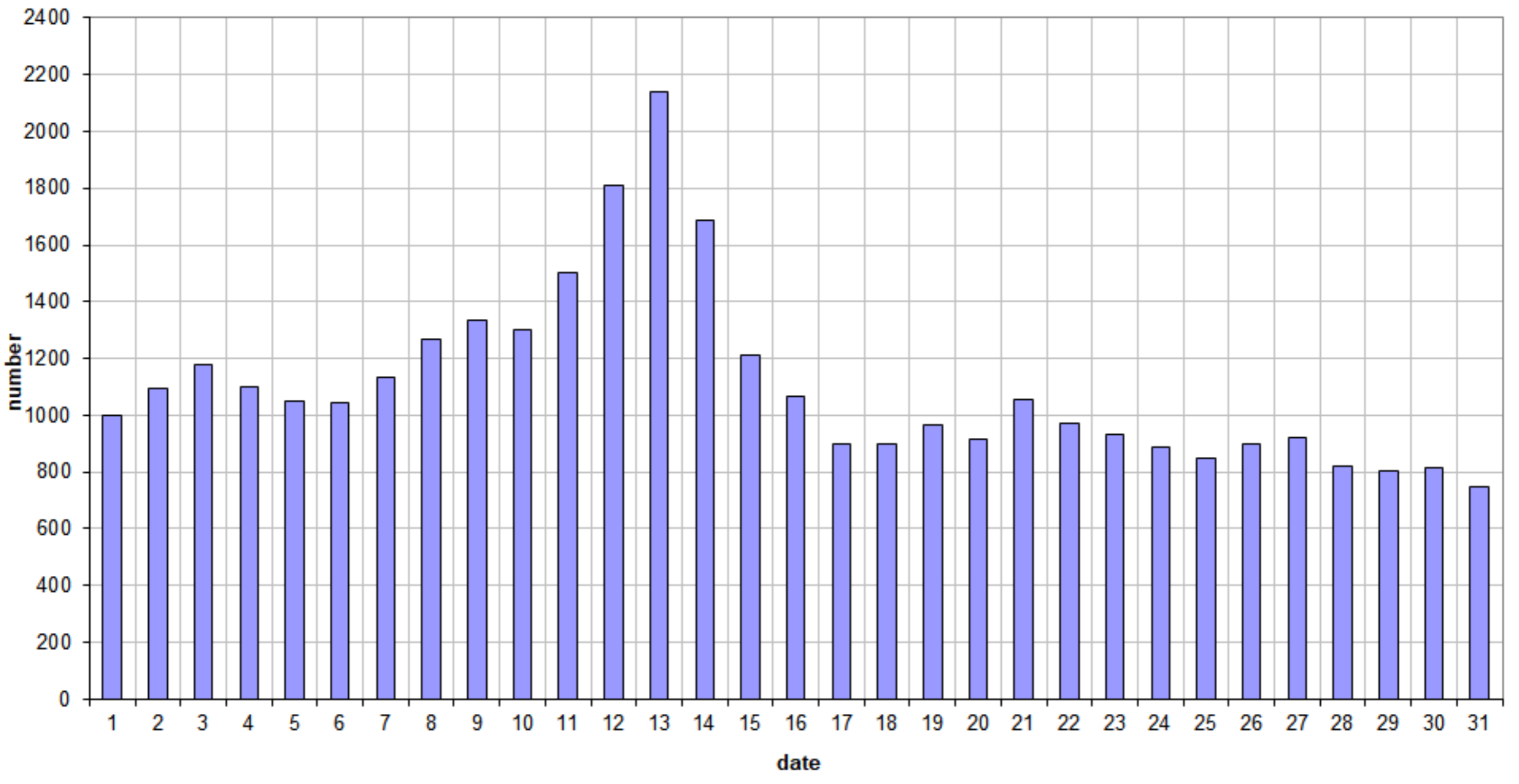
49.99MHz - RadioMeteors December 2024 daily totals of "all" reflections (automatic count_Mettel5_7Hz) Felix Verbelen (Kampenhout)
