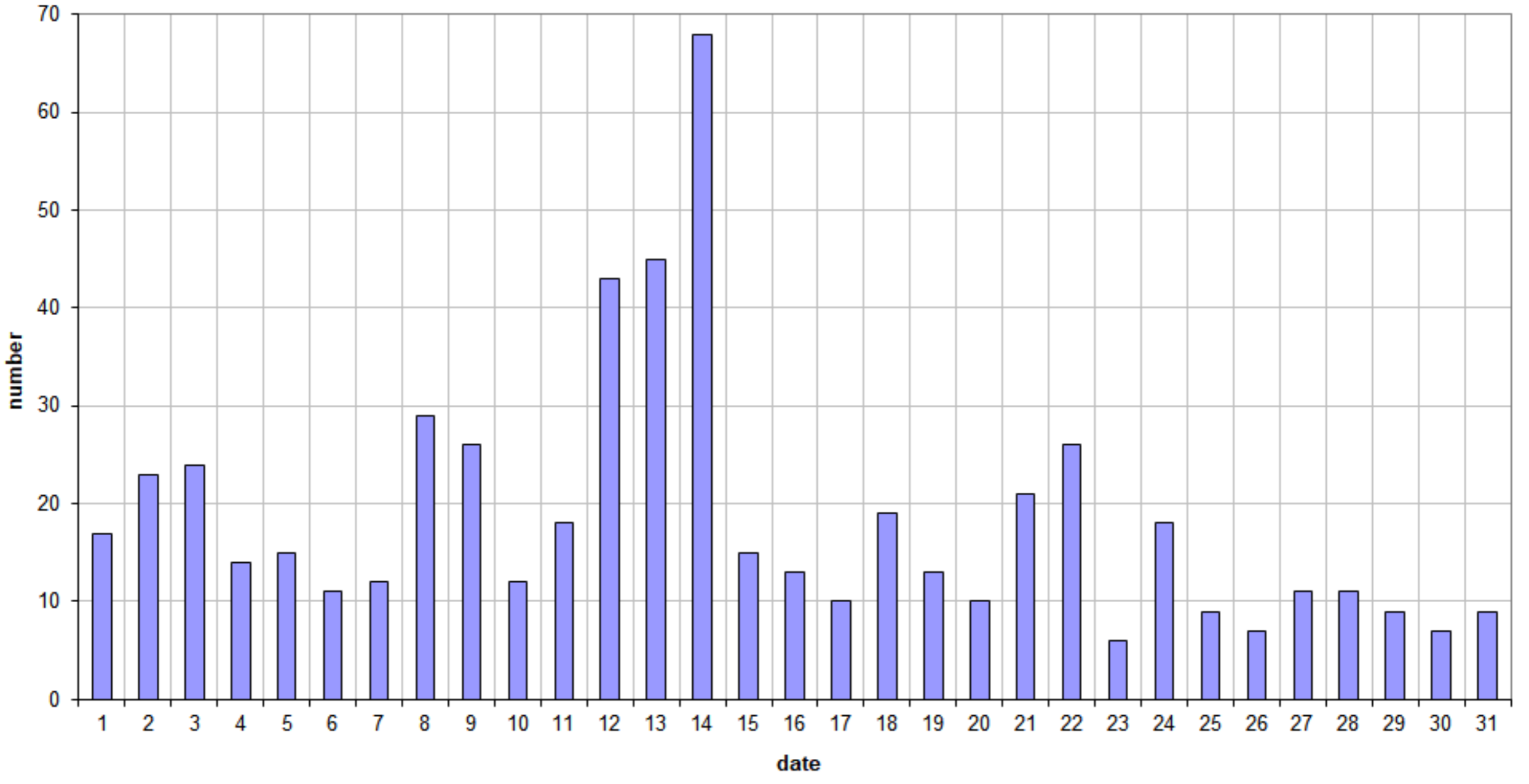
49.99MHz - RadioMeteors December 2024 daily totals of reflections longer than 10 seconds Felix Verbelen (Kampenhout)
