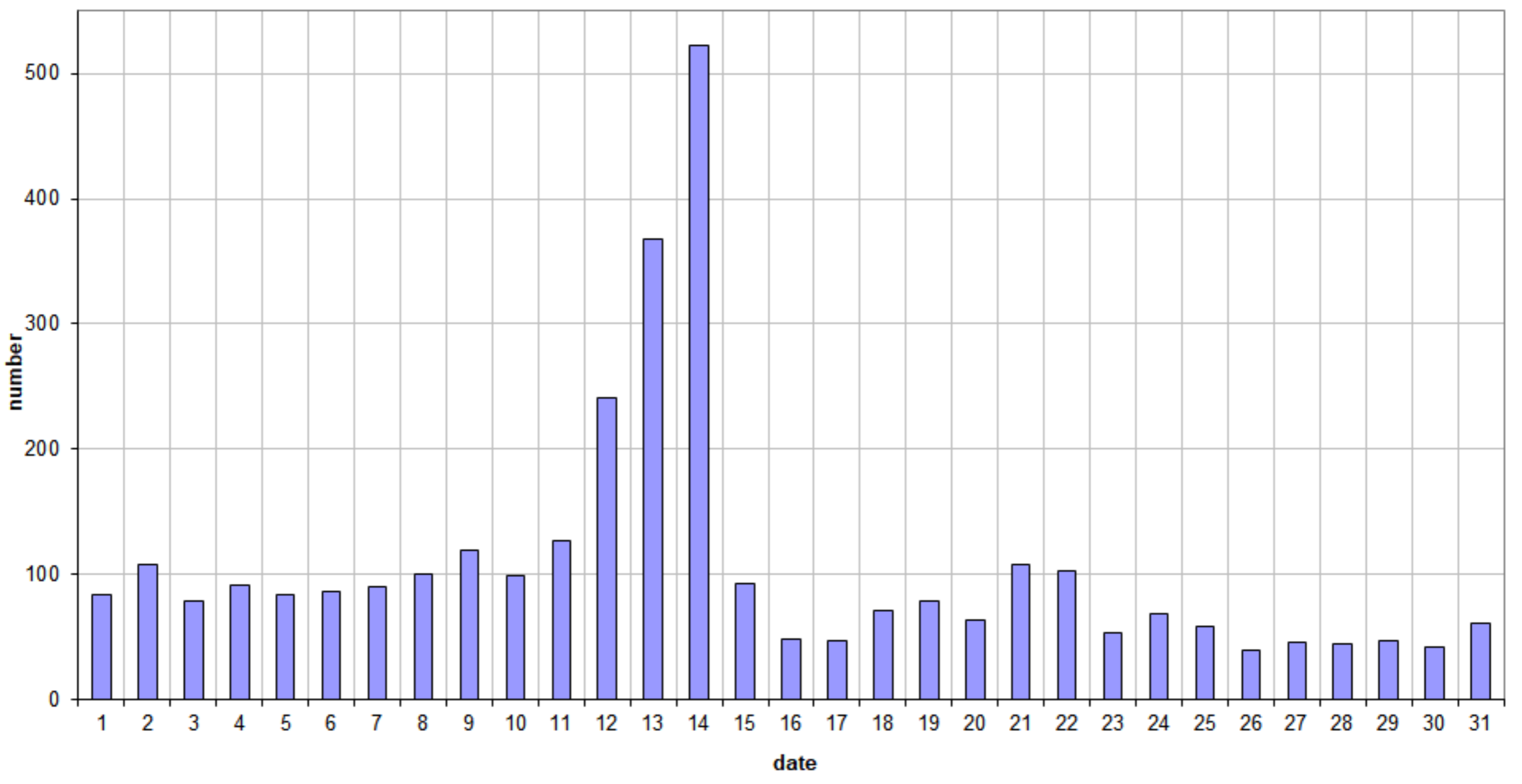
49.99MHz - RadioMeteors December 2024 daily totals of all overdense reflections Felix Verbelen (Kampenhout)
