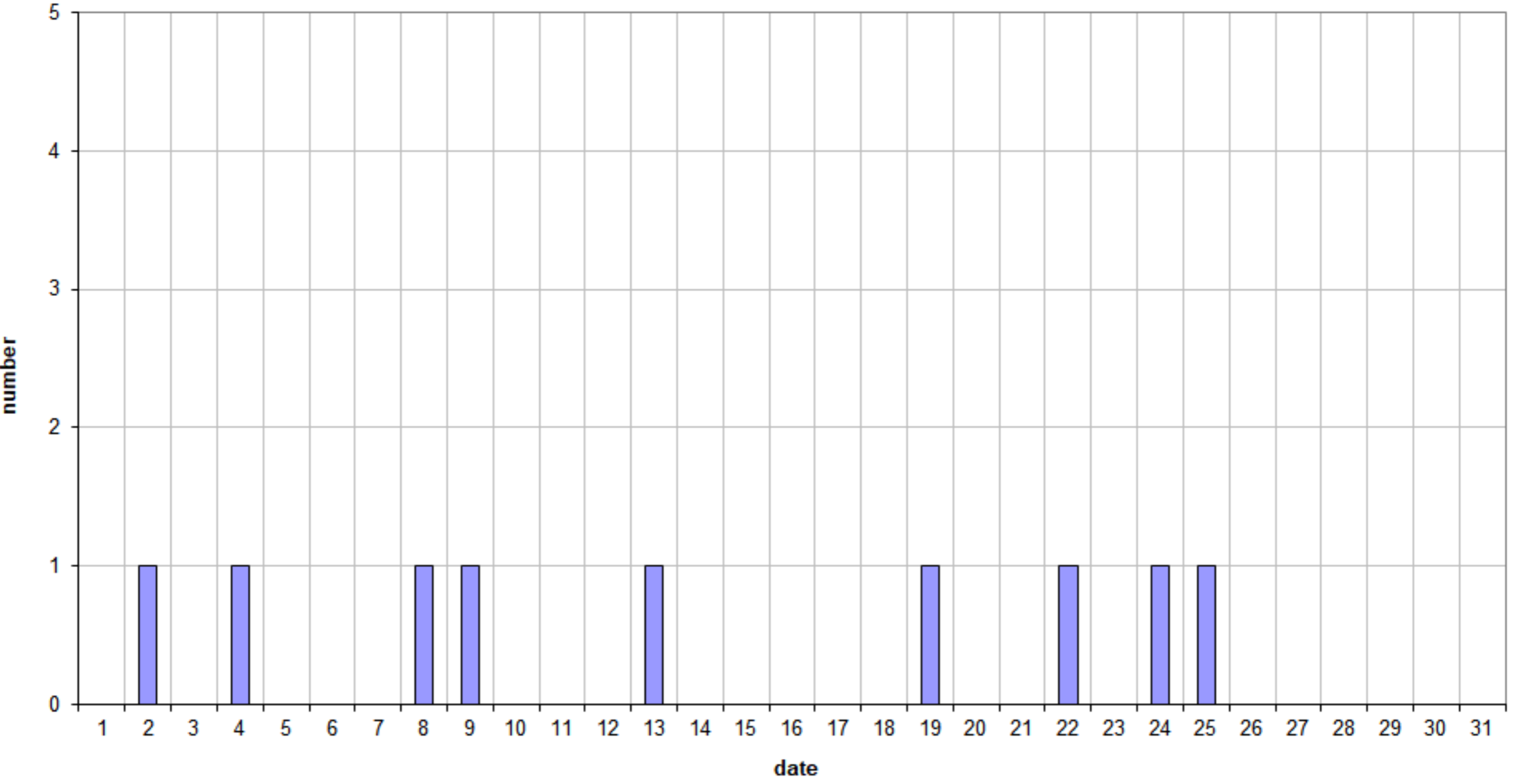
49.99MHz - RadioMeteors December 2024 daily totals of reflections longer than 1 minute Felix Verbelen (Kampenhout)
